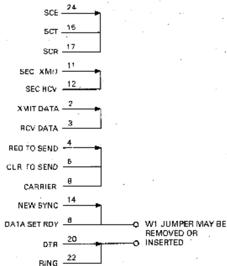
Figure 1-5 Loopback Connection
