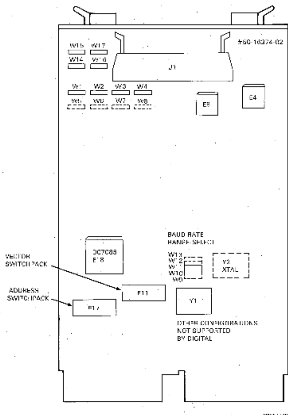
Figure 2-3 Jumper Locations (DC7085 Surface Mount)
