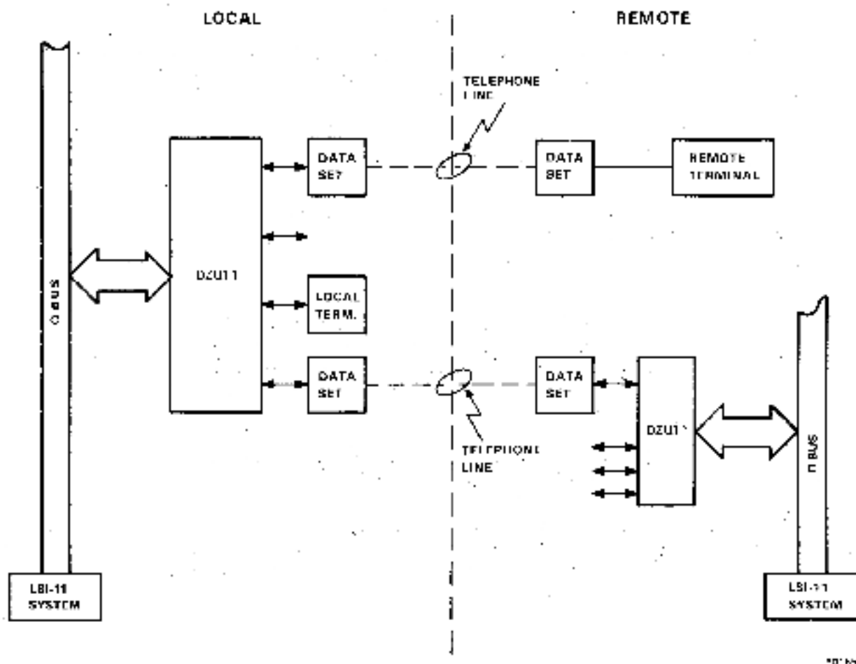
Figure 1-2 DZQ11 System Applications
