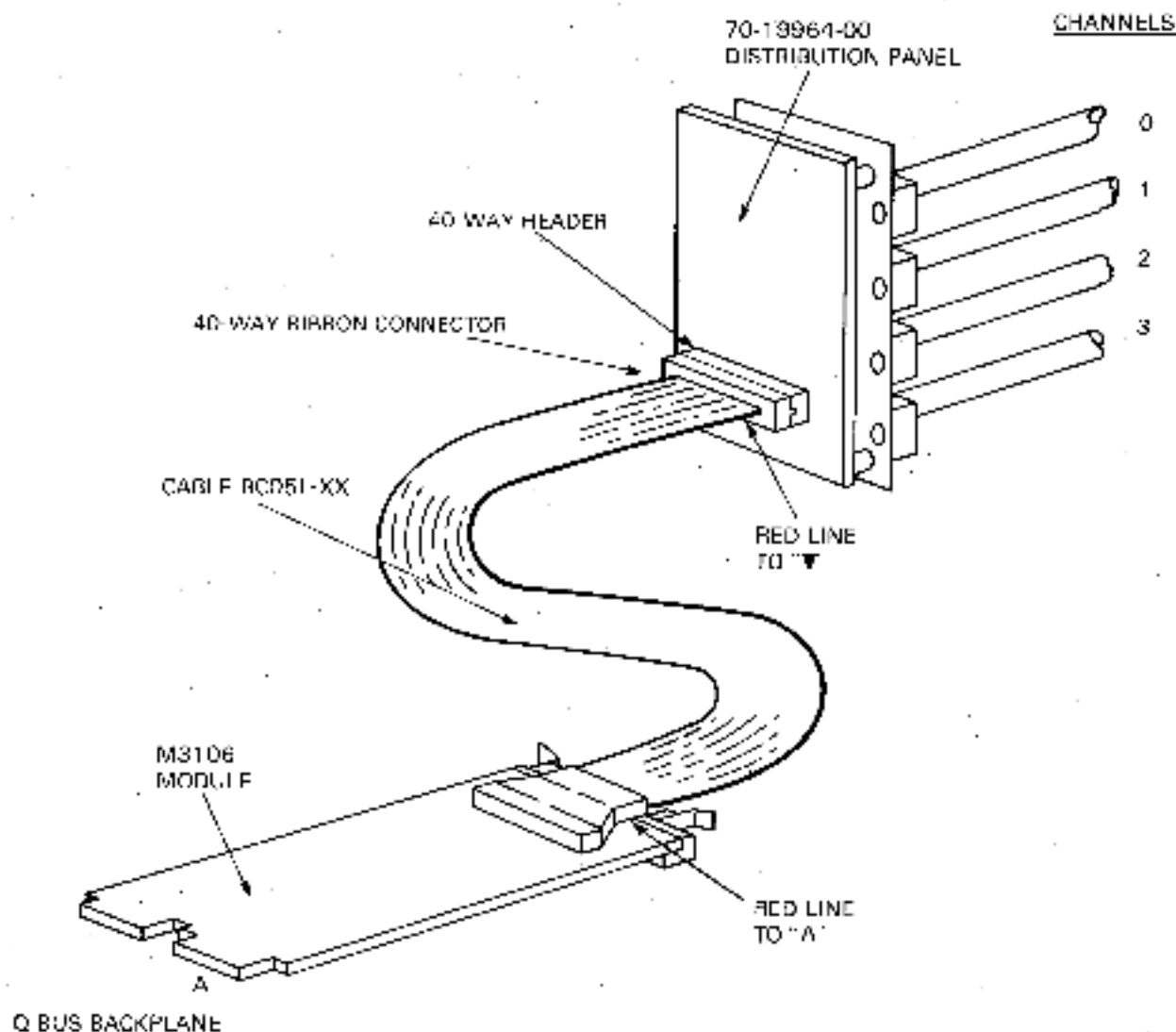
Figure 2-5 DZQ11 Installation (70-19964-00)
