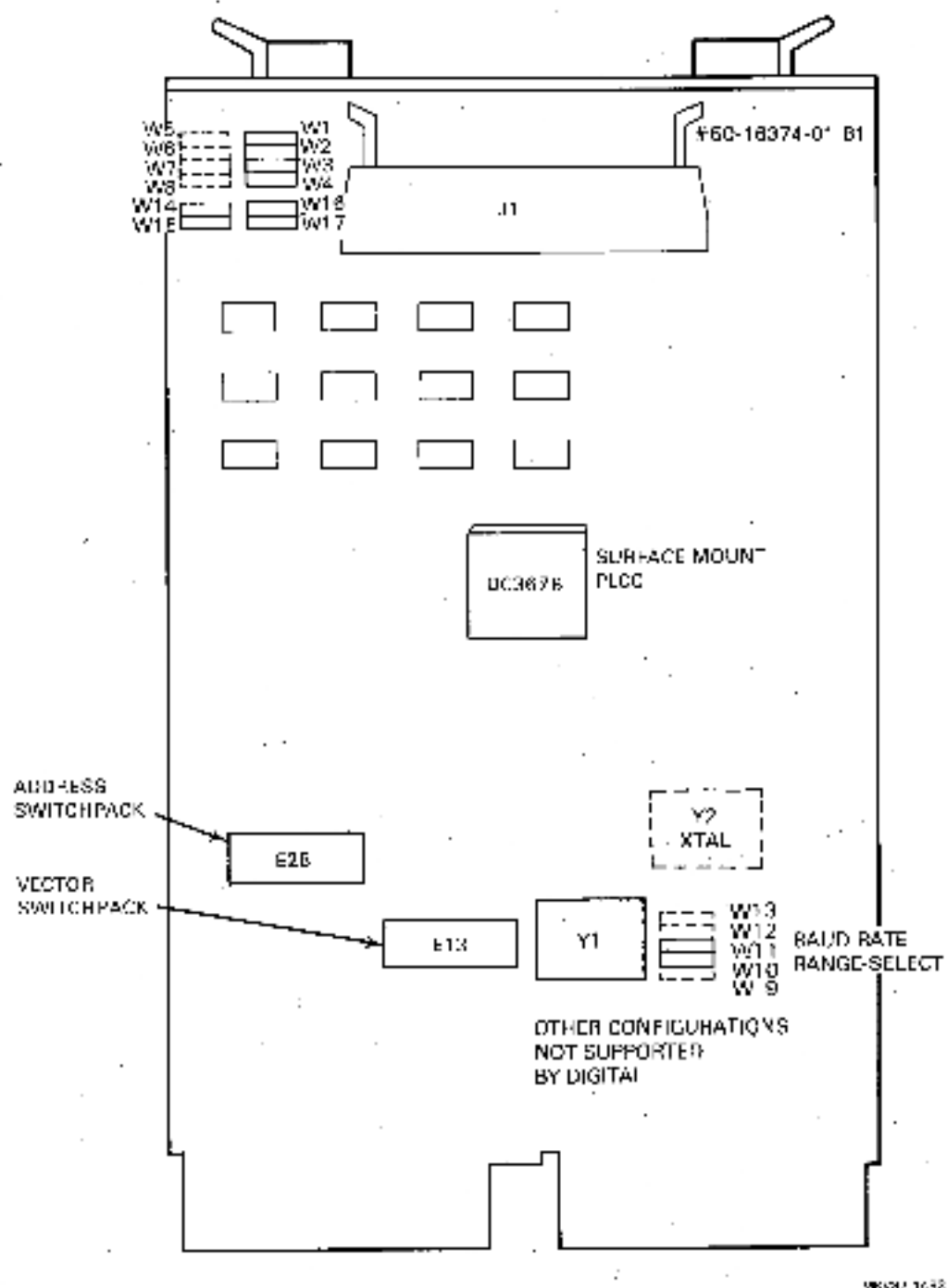
Figure 2-2 Jumper Locations (DC367B Surface Mount)
