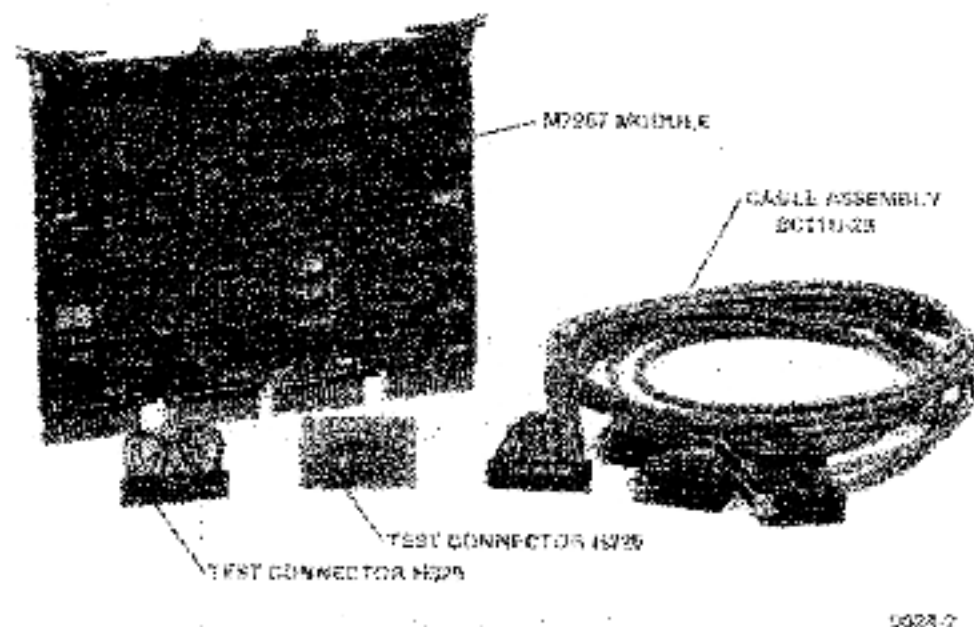
Figure 1-3 DZV11-B (M7957 Module, H325 and H329 Connectors and Cable Assembly BC11U-25)
