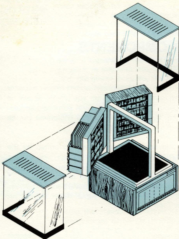
Figure 1 — Table Model PDP-8 showing removeable covers and swinging palets that allow access to all components.
