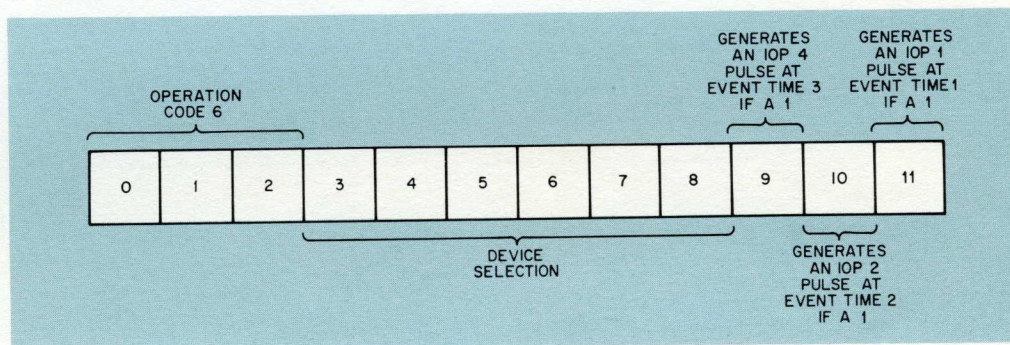
Figure 5 IOT Instruction Format
