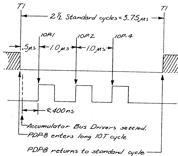
Fig. 11 IOT Timing Cycle
