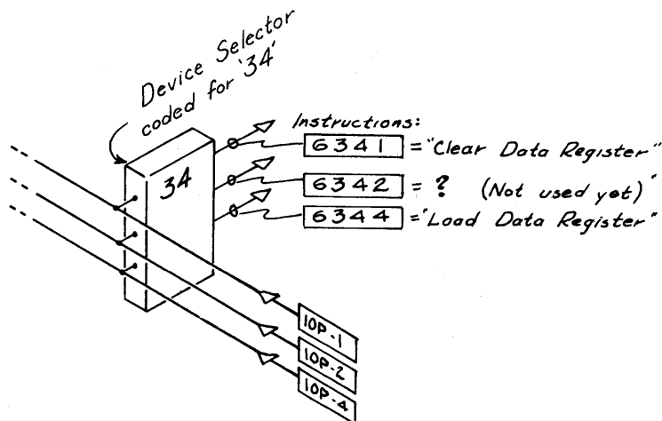
Fig. 5 Instruction Coding for Producing IOT Pulses
