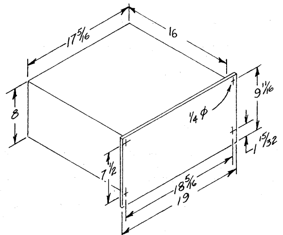
Power Supply
