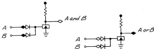
Fig. 27 Diamonds Indicate Voltage Levels
