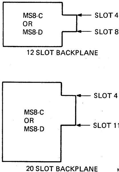
Figure 2-1 Configuration with One Backplane
