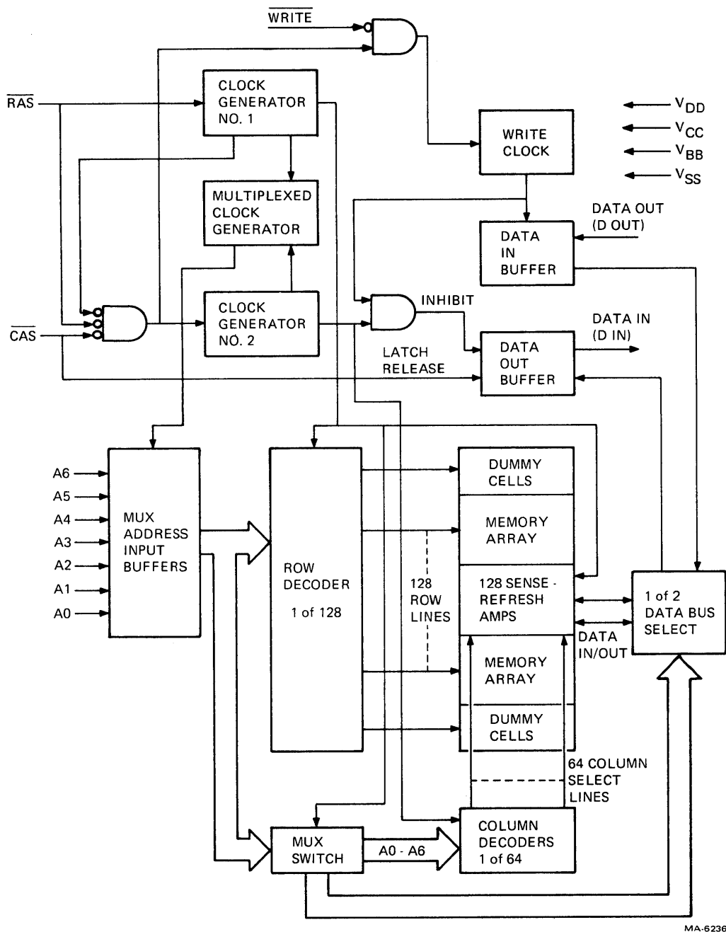
Figure 3-3 16384 × 1 Bit MOS RAM Block Diagram
