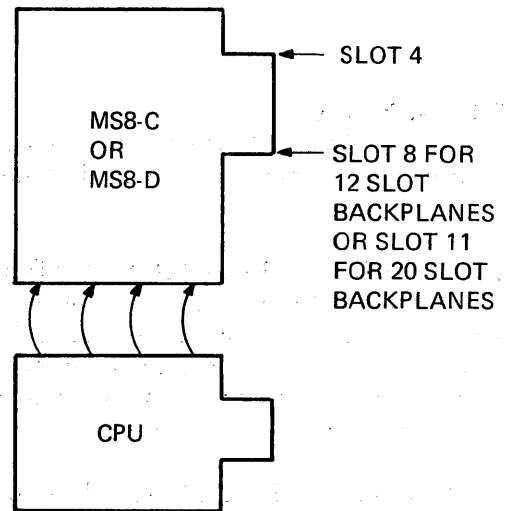
Figure 2-2 Typical Configuration with Two Backplanes
