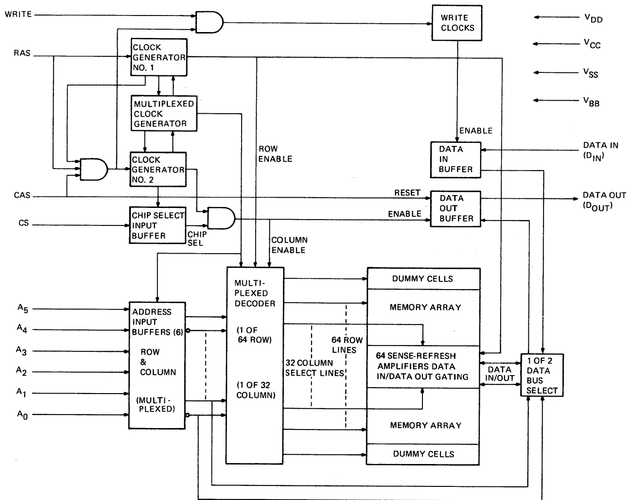
Figure 3-2 4096 \times 1 Bit MOS RAM Block Diagram
