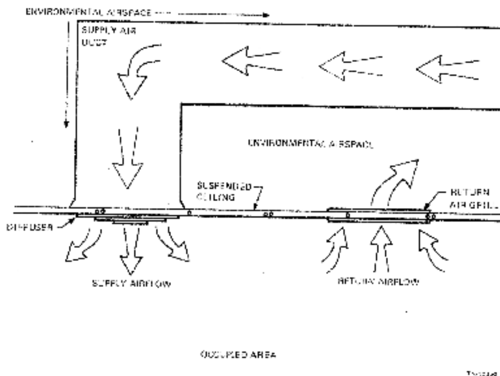
Figure 2-5 Typical Above-Ceiling Environmental Airspace
