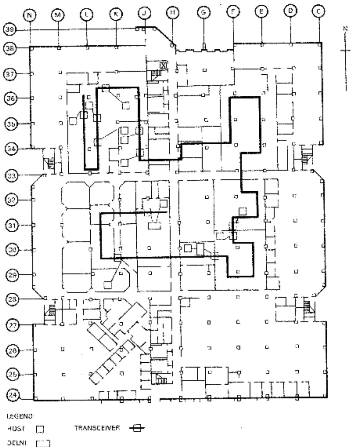
Figure 3-2 Ethernet Component Layout
