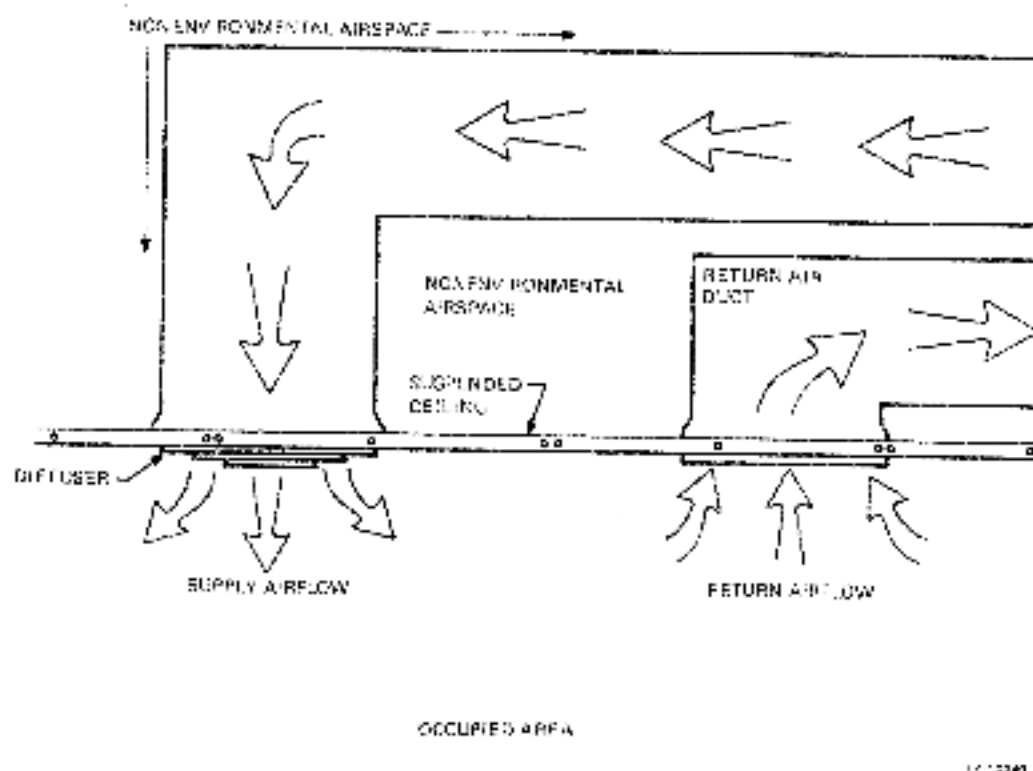
Figure 2-6 Typical Above-Ceiling Nonenvironmental Airspace
