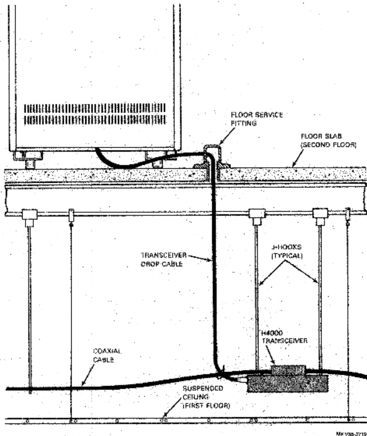
Figure 2-4 Transceiver Drop Cable Routed to an Above-Served Station in a Suspended-Ceiling Installation
