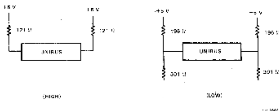
Figure 4-10 Hi/Lo Terminator Circuit Example
