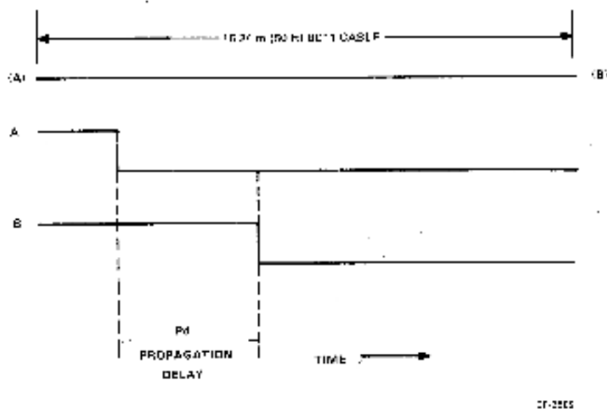
Figure 3-4 BC11-A Unibus Cable Delay Example
