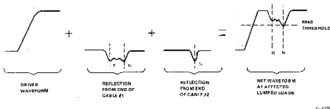
Figure 2-17 Violation of Rule No. 5 (Waveform Example)
