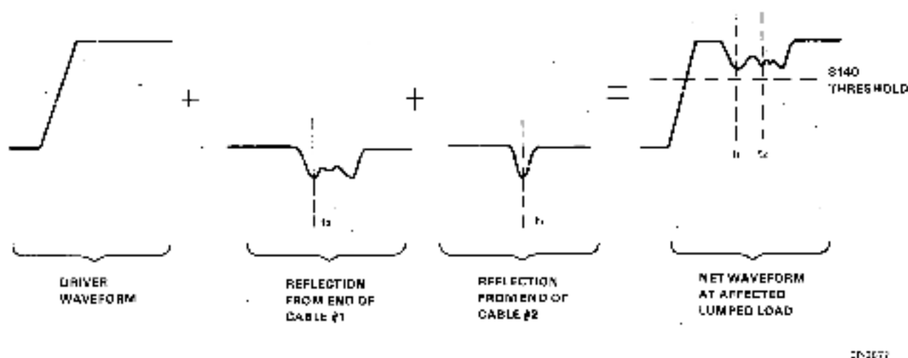
Figure 2-18 Implementation of Rule No. 5 (Waveform Example)
