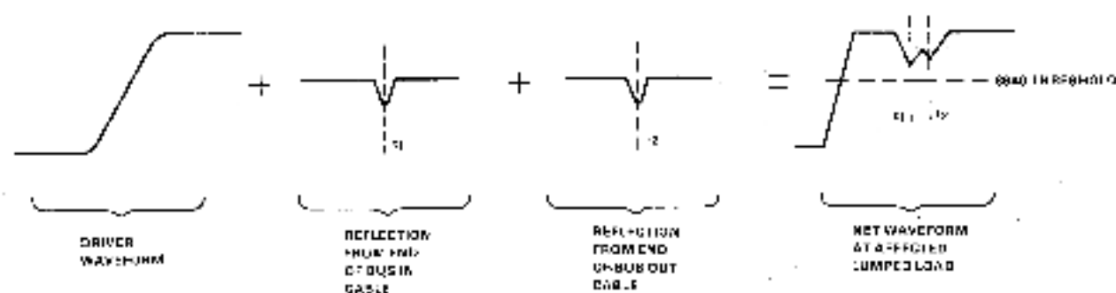
Figure 2-14 Rule No. 4 Implementation (Waveform Example)
