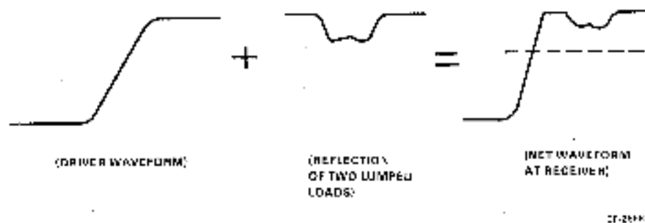
Figure 2-8 Rule No. 3 Implementation (Waveform Example)
