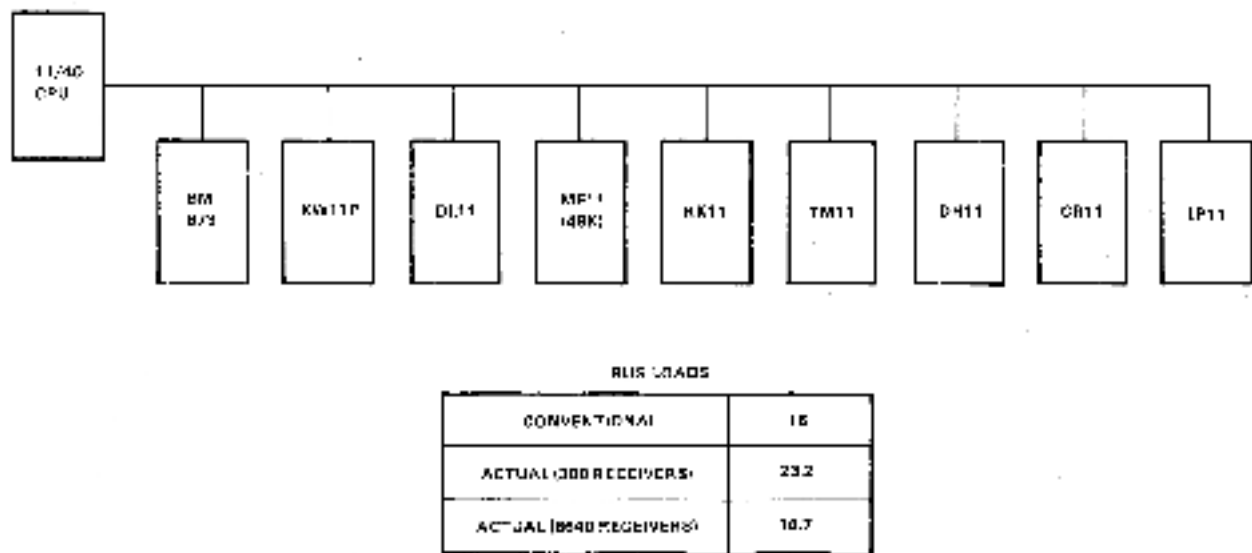
Figure 2-19 Actual Bus Loads Example
