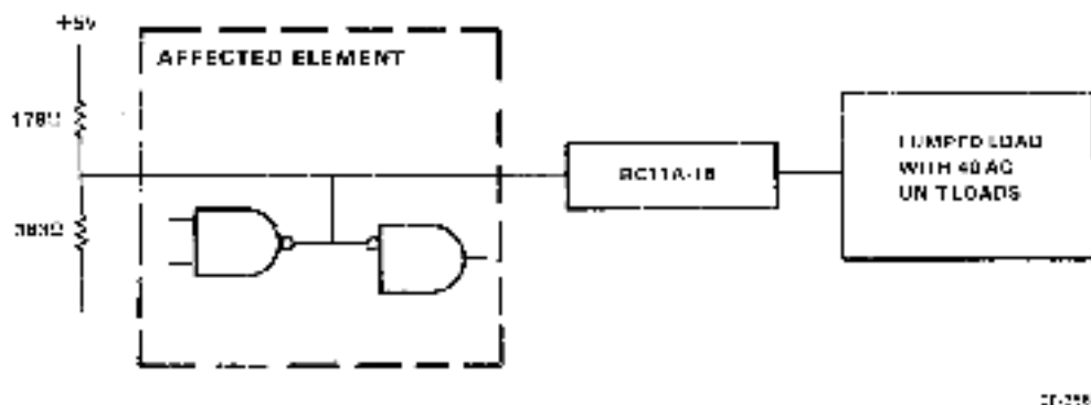
Figure 2-5 Rule No. 3 Violation (Block Diagram)
