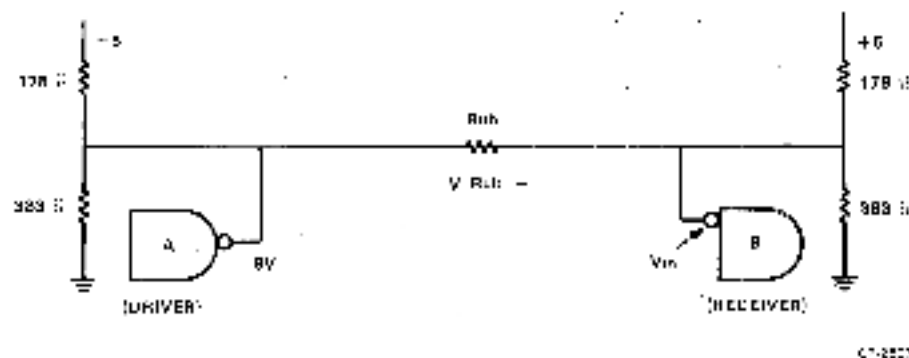
Figure 3-12 Cable Resistance Problems Example
