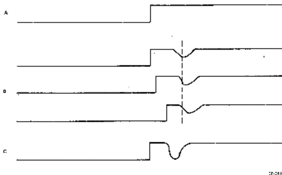
Figure B-1 Composite and Signature Waveforms
