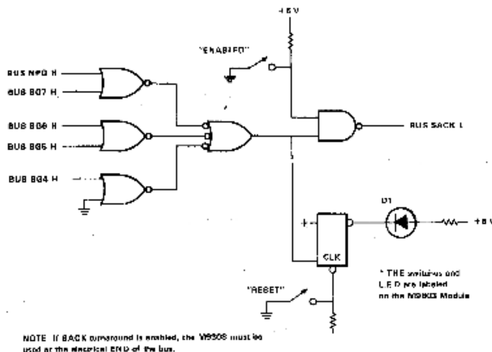
Figure 4-17 M9308 SACK Turnaround Logic
