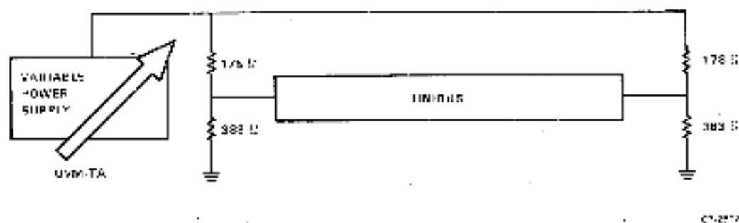
Figure 4-11 UVM-TA Circuit Representation
