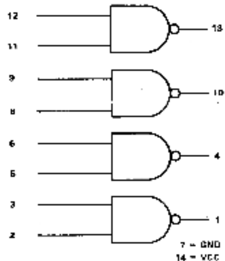
8881 DRIVER
