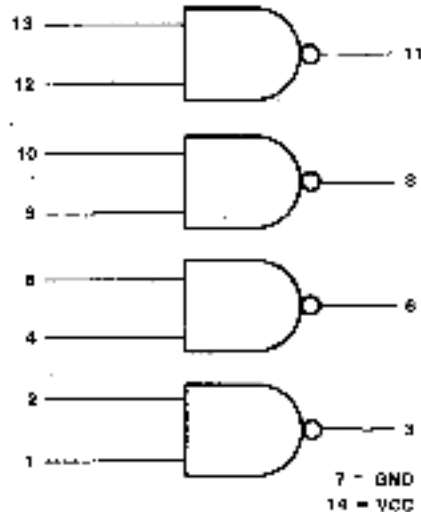
74H01 DRIVER
