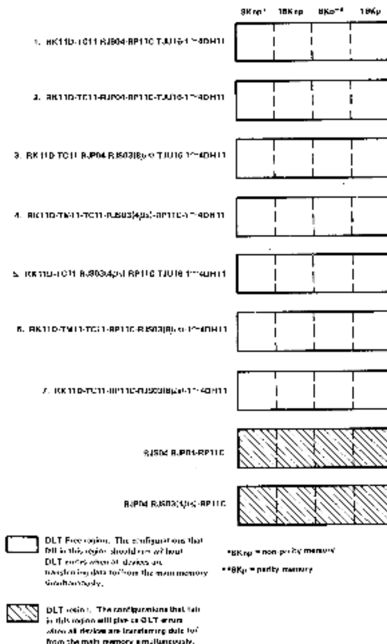
Figure 2-24 DLT Configurations
