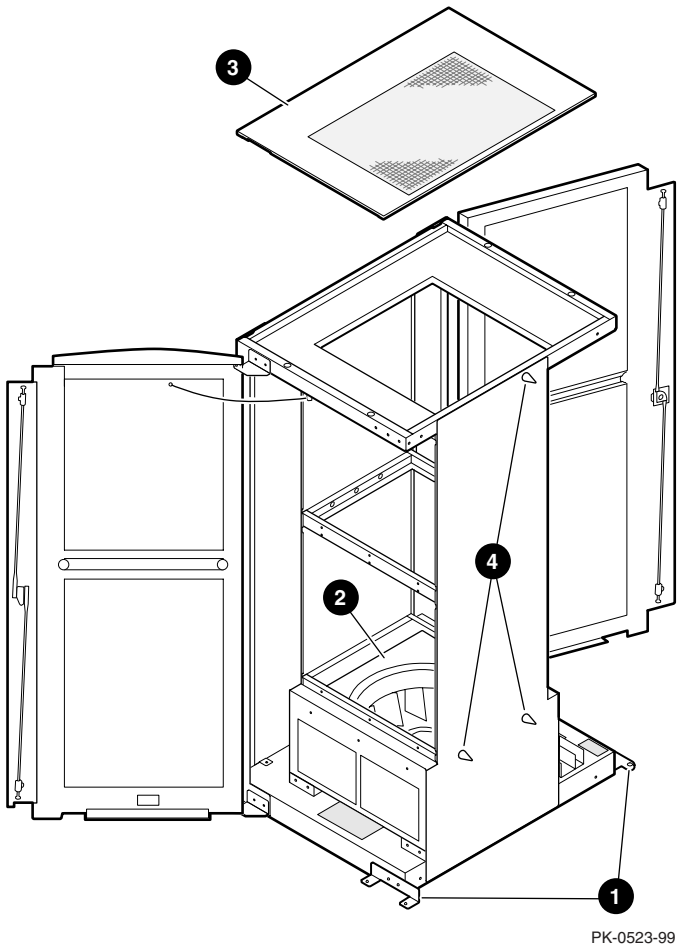
Figure 3-4 Preparing System Cabinet 2 for Joining
