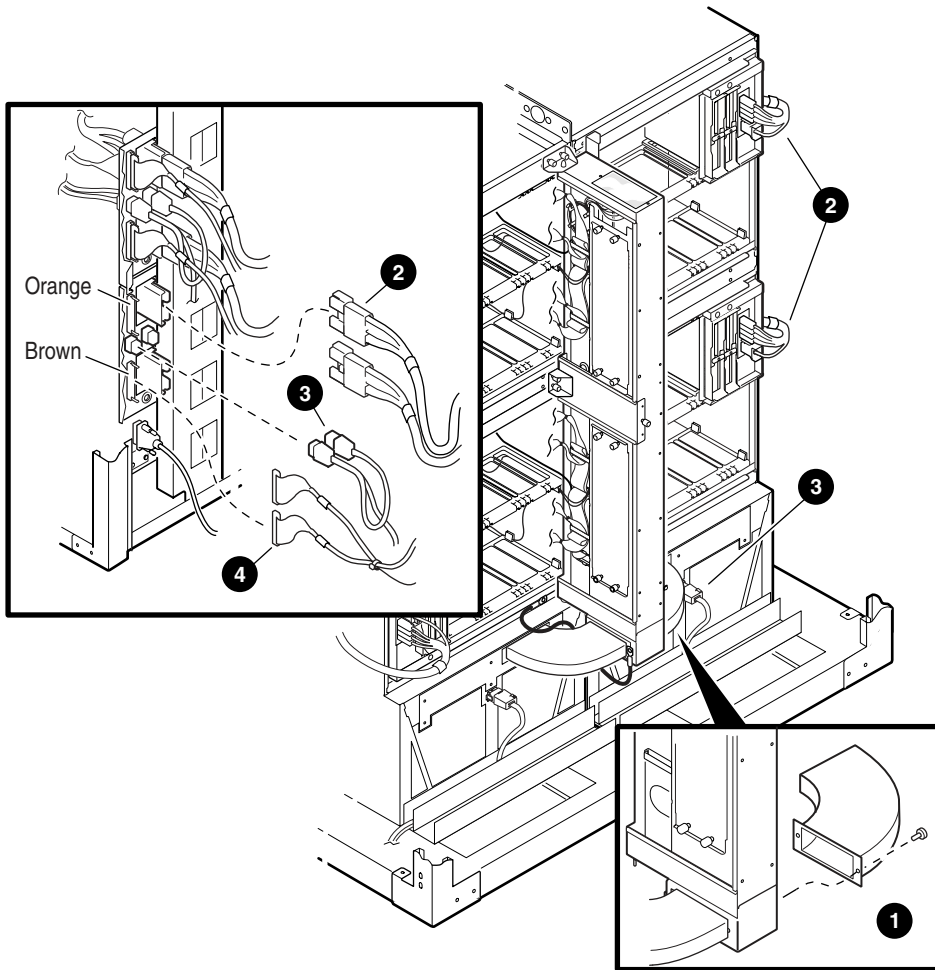
Figure 3-9 External Cable Connections
