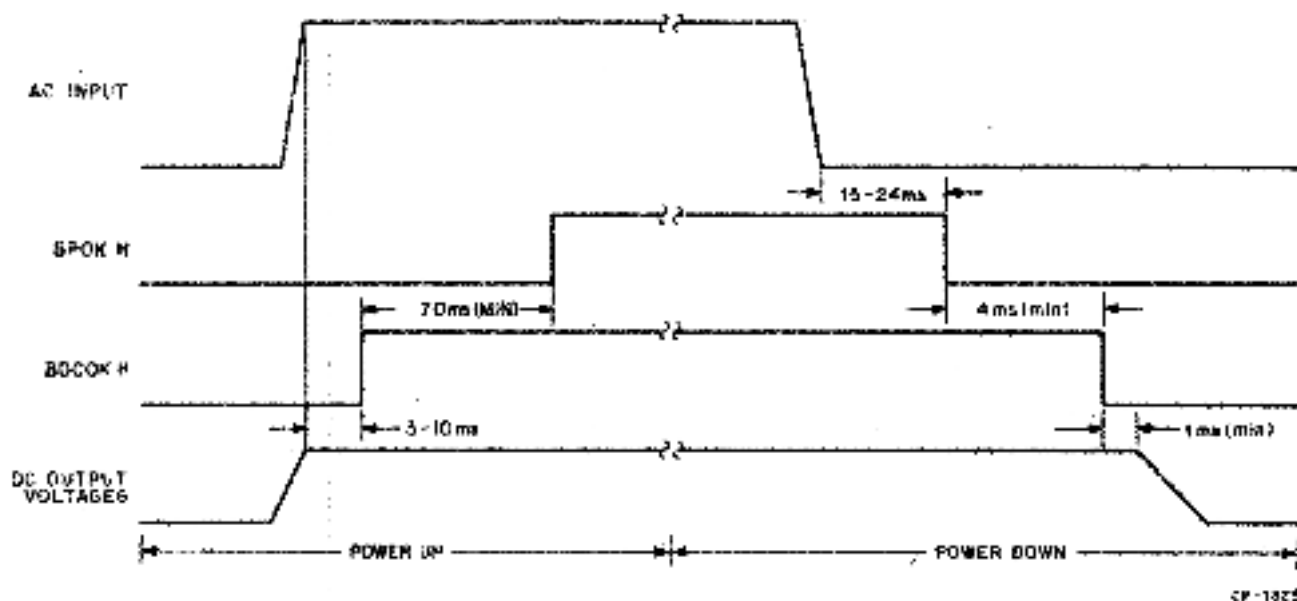
Figure 3-6 Power-Up/Power-Down Sequence
