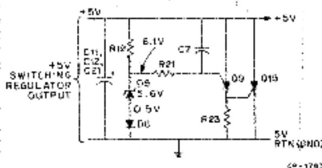
Figure 3-4 Crowbar Circuit
