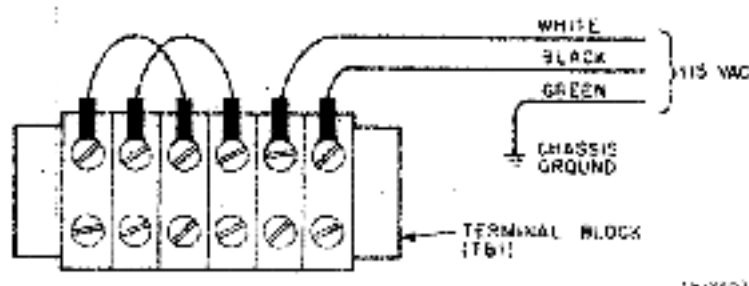
Figure 2-2 H780-C, -H, and -K (115 Vac) AC Terminal Block Wiring Configuration
