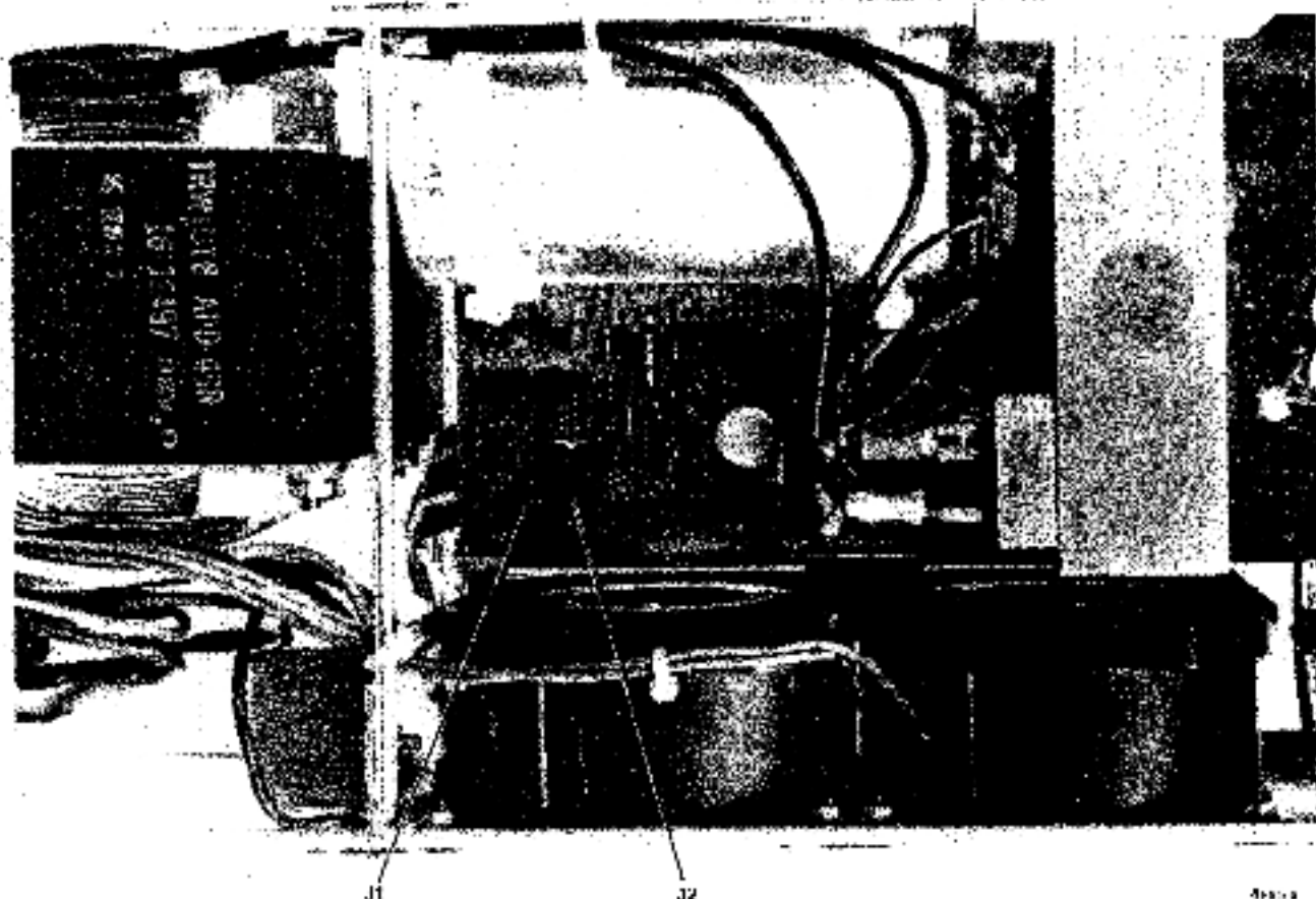
Figure 2-4 Locations of J1 and J2 on Power Supply Board
