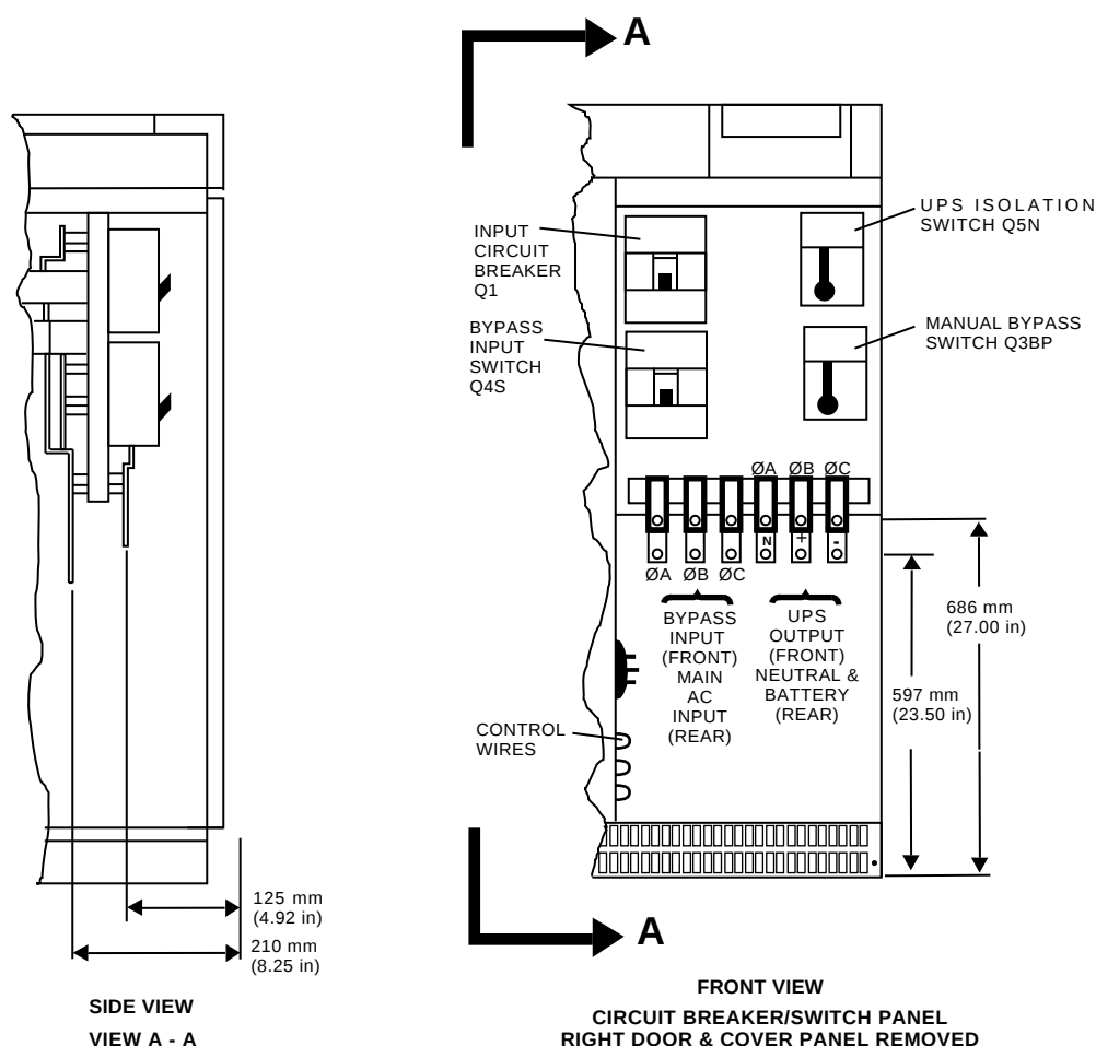
Figure 4-1 UPS Cabinet Power Wiring Connections
