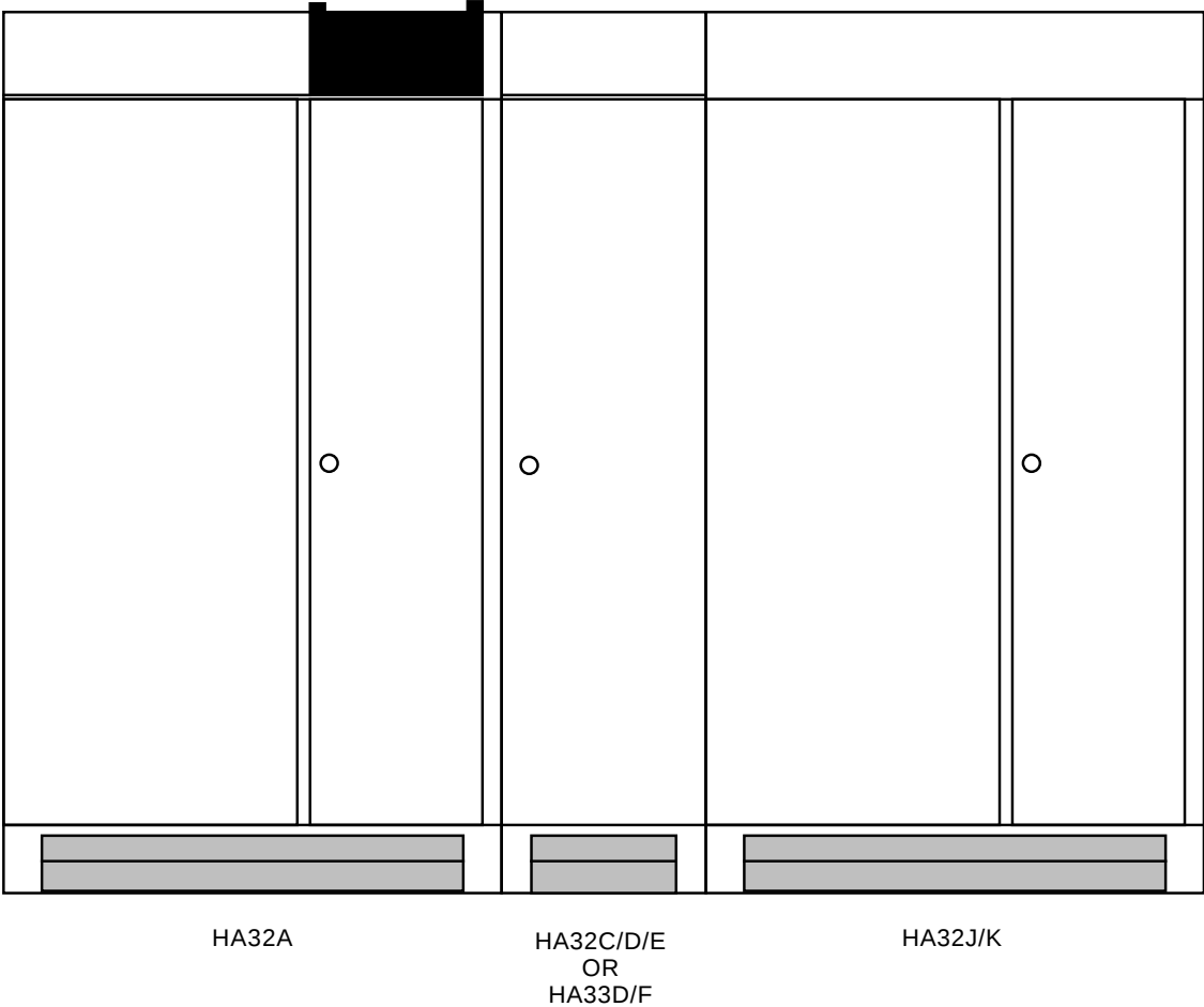
Figure 2-8 UPS Cabinet, UPS Auxiliary Cabinet or UPS CSA Cabinet, and UPS Distribution Cabinet Placement
