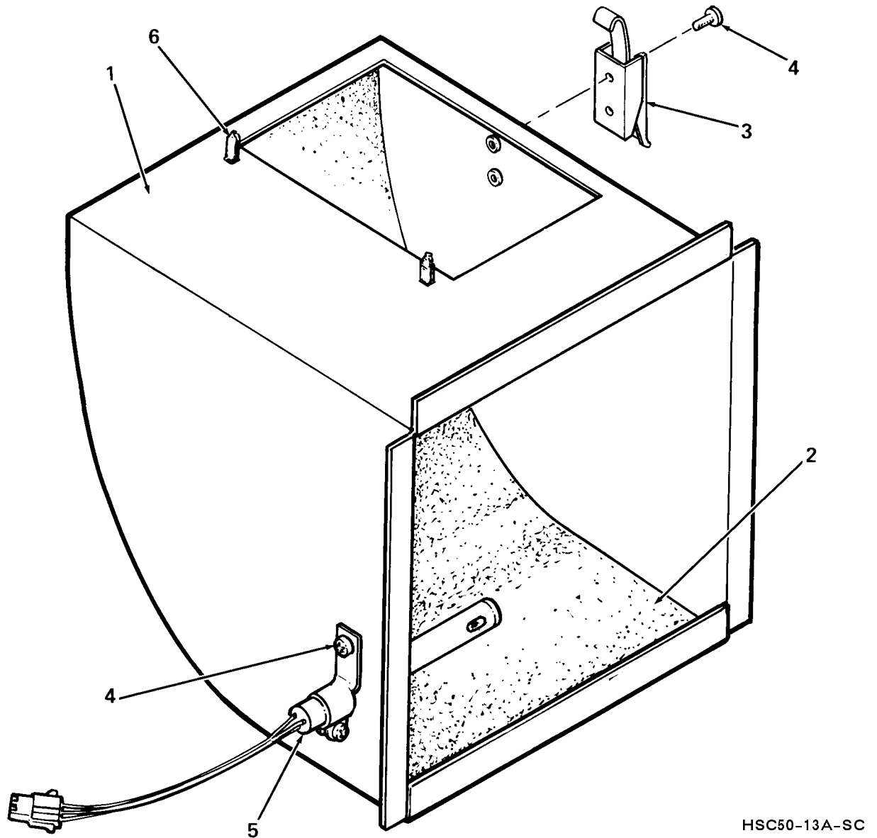
Figure 13A. Duct Assembly, Outlet (Modified Design)
