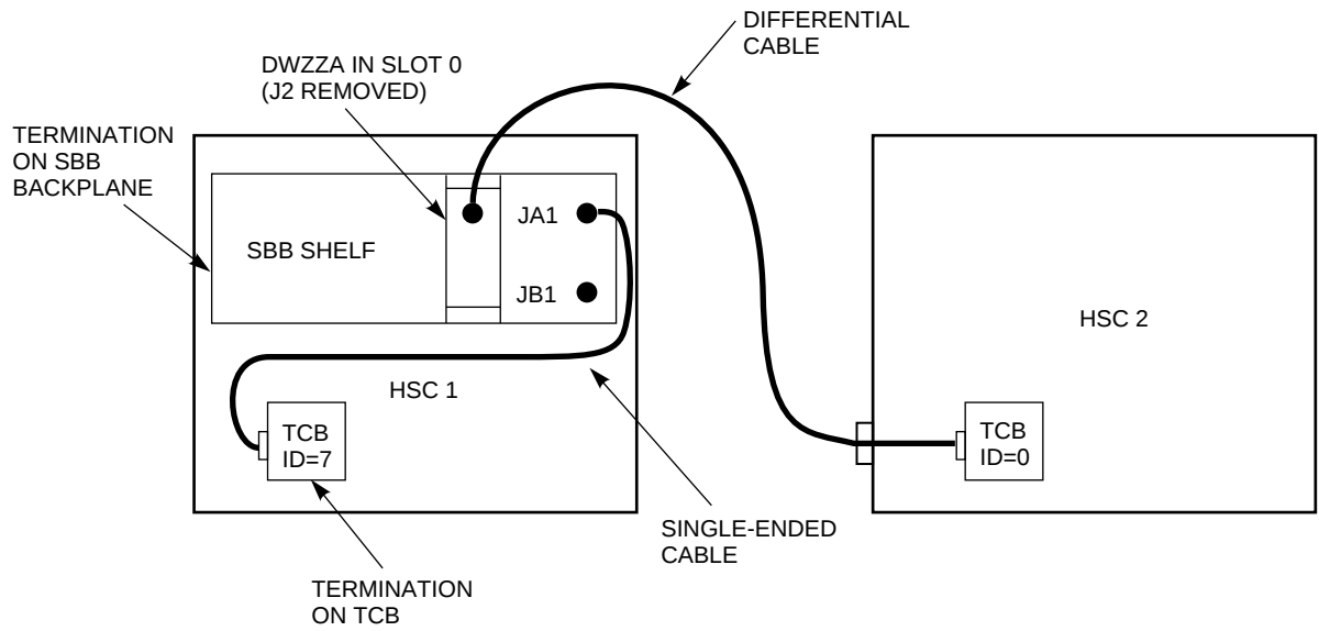
Figure A-3 Dual-Path HSC Controllers with Internal SBBs
