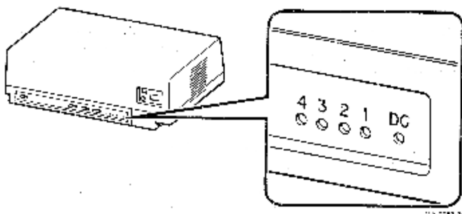
Figure 4-5 System Unit Status Indicators
