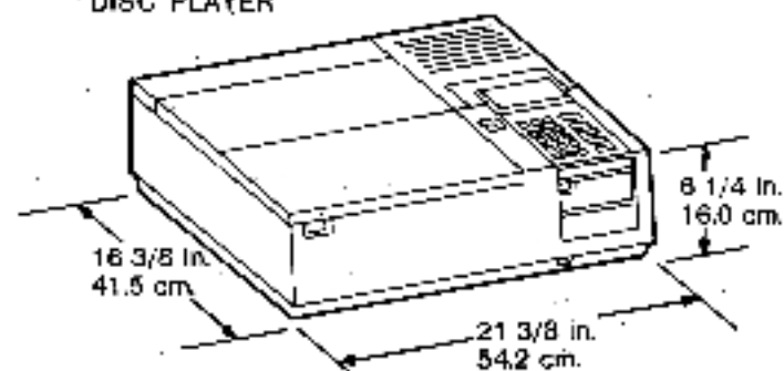
DISC PLAYER
