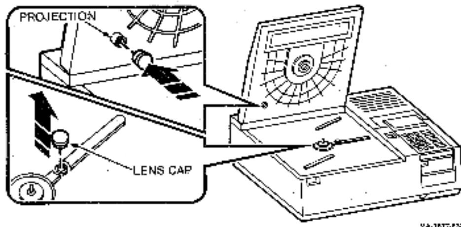
Figure 4-13 VDP40 (Sony LDP-1000A) Objective Lens
