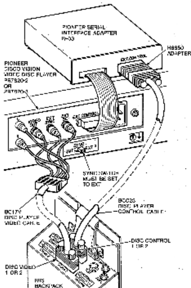
Figure 5-3 Connecting a Pioneer/Discovision Video Disc Player
