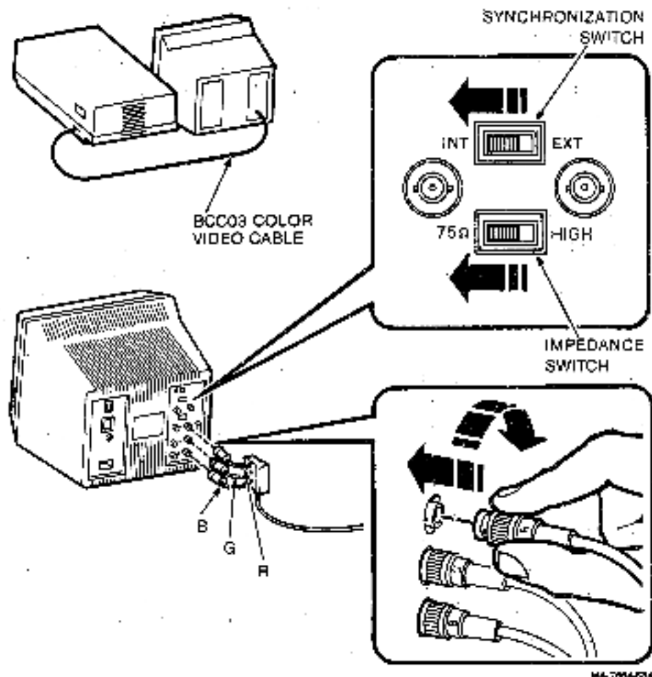
Figure 5-6 Connecting One Color Video Monitor
