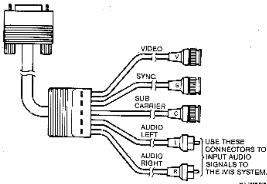
Figure 5-13 BCL7V Audio Input Connectors
