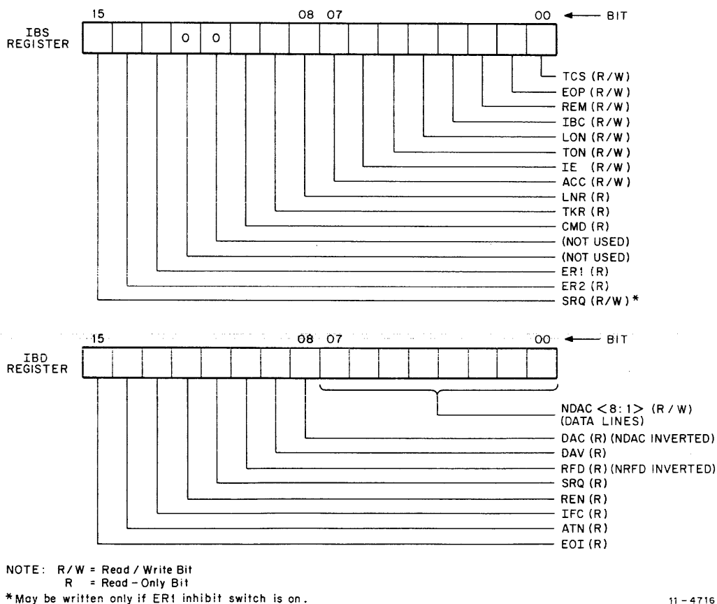
Figure 2-3 IBV11-A Register and Bit Assignments
