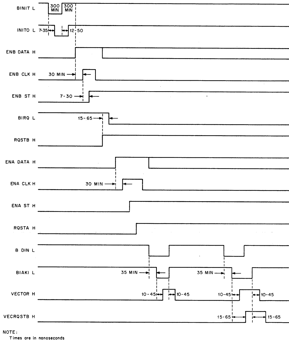
Figure A-3 DC003 "A" and "B" Interrupt Sections Timing Diagrams
