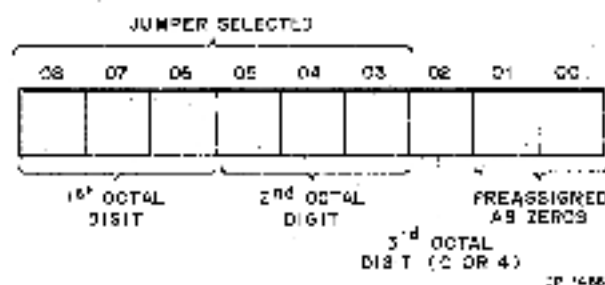
Figure 2-2 DECKit I-M Interrupt Vector Address Select Format
