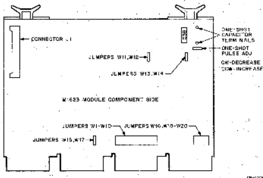
Figure 2-5 M1623 Module Layout
