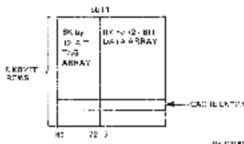
Figure 3-15 Second-Level Cache Organization
