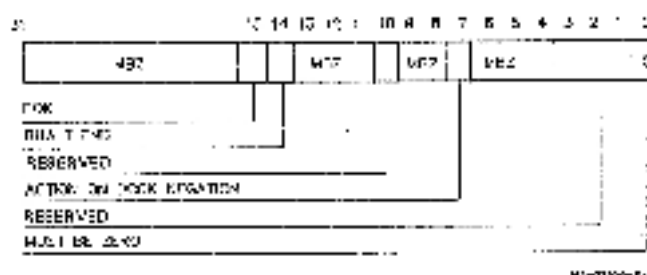
Figure 3-40 System Configuration Register
