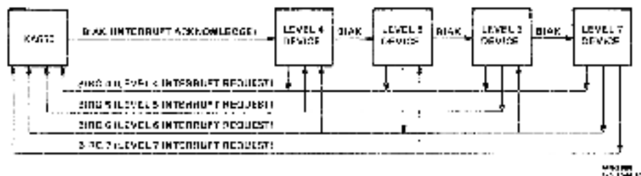
Figure C-13 Position-Independent Configuration
