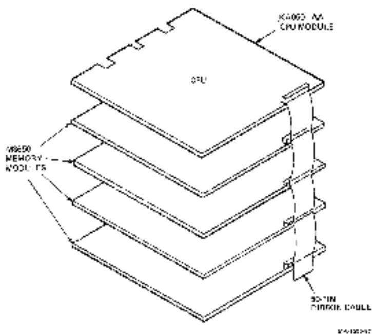
Figure 2-2 Cable Connections
