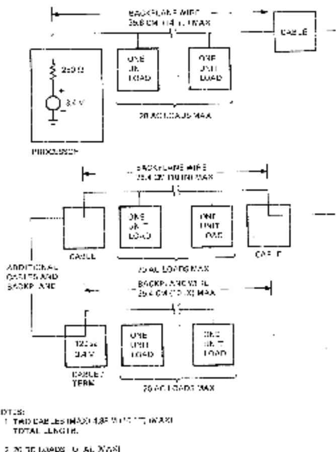
Figure C-18 Multiple Backplane Configuration
