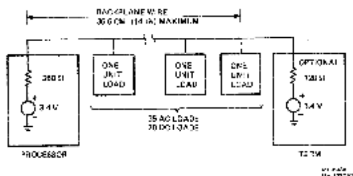
Figure C-17 Single-Backplane Configuration
