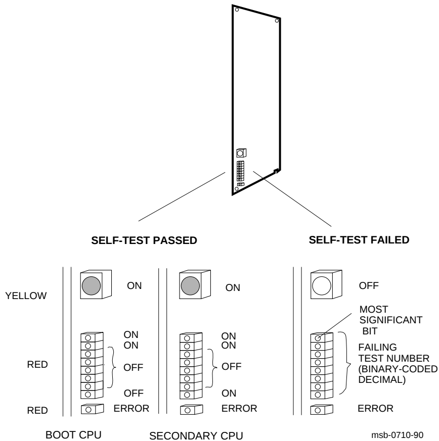
Figure B-1: KA65A LEDs After Power-Up Self-Test
