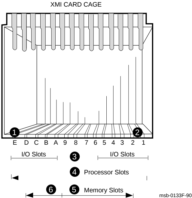
Figure A-1: Configuration Rules for Model 500 Scalar Systems
