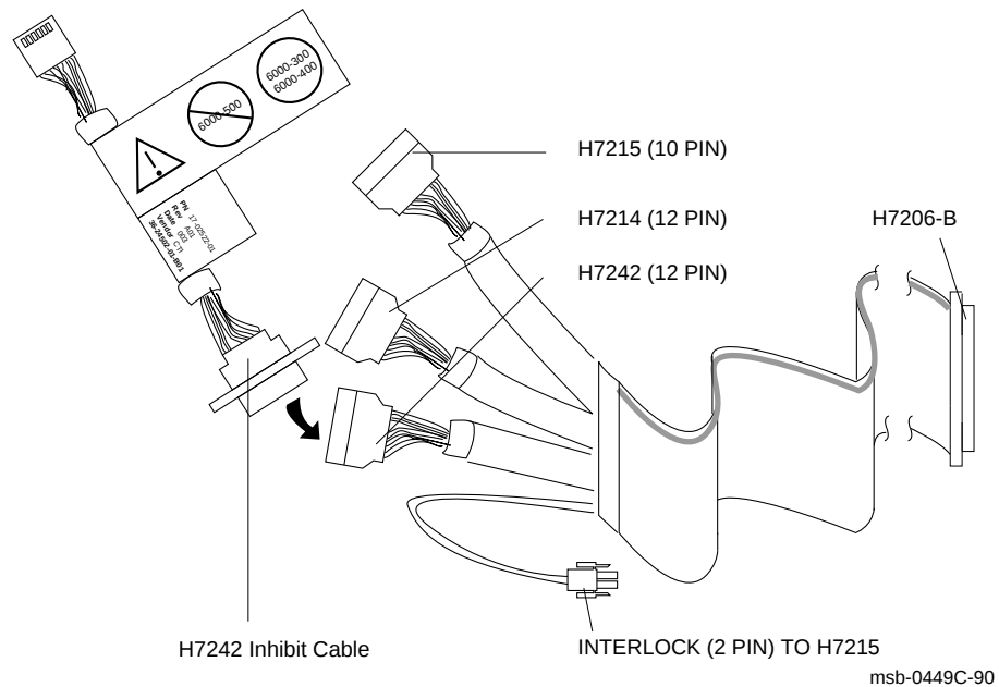
Figure 3–1: Removing the +3.3V Inhibit Cable
