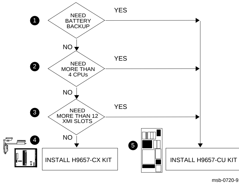
Figure 1-2: Tradeoffs Between the H9657-CX and H9657-CU Upgrades
