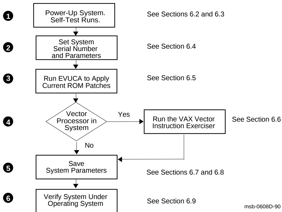
Figure 6-1: Verification Flowchart
