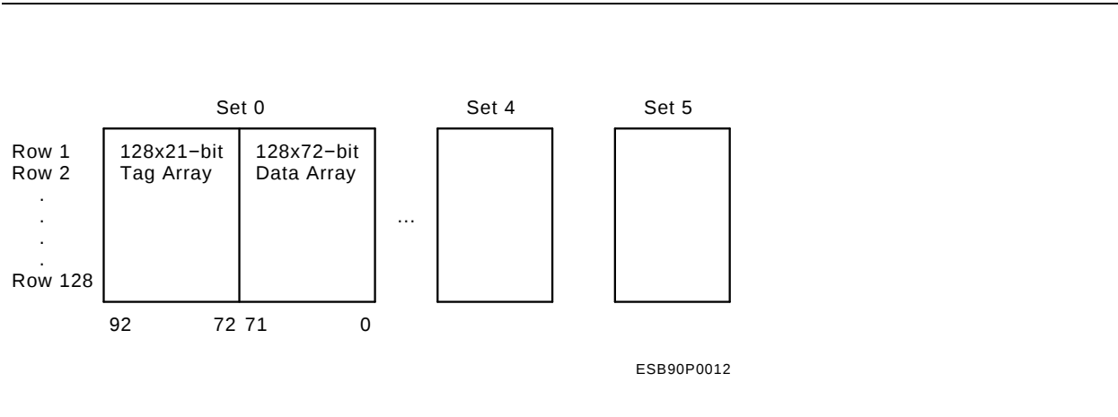
Figure 4-1: Logical Organization of Cache
