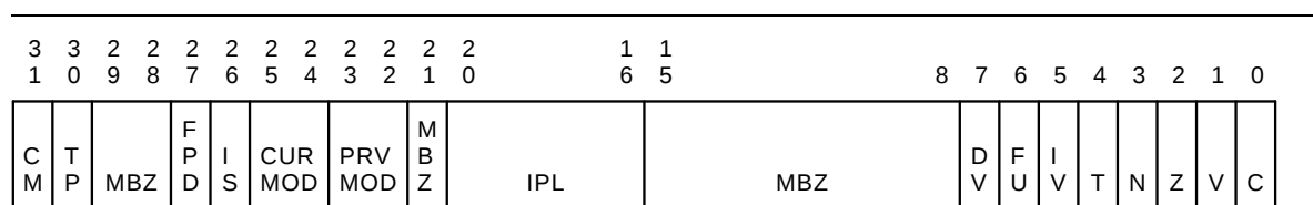
Figure 3-2: PSL Format
