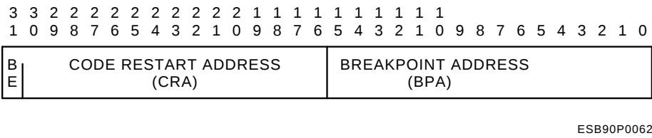
Figure 10–12: NICSR14 format
