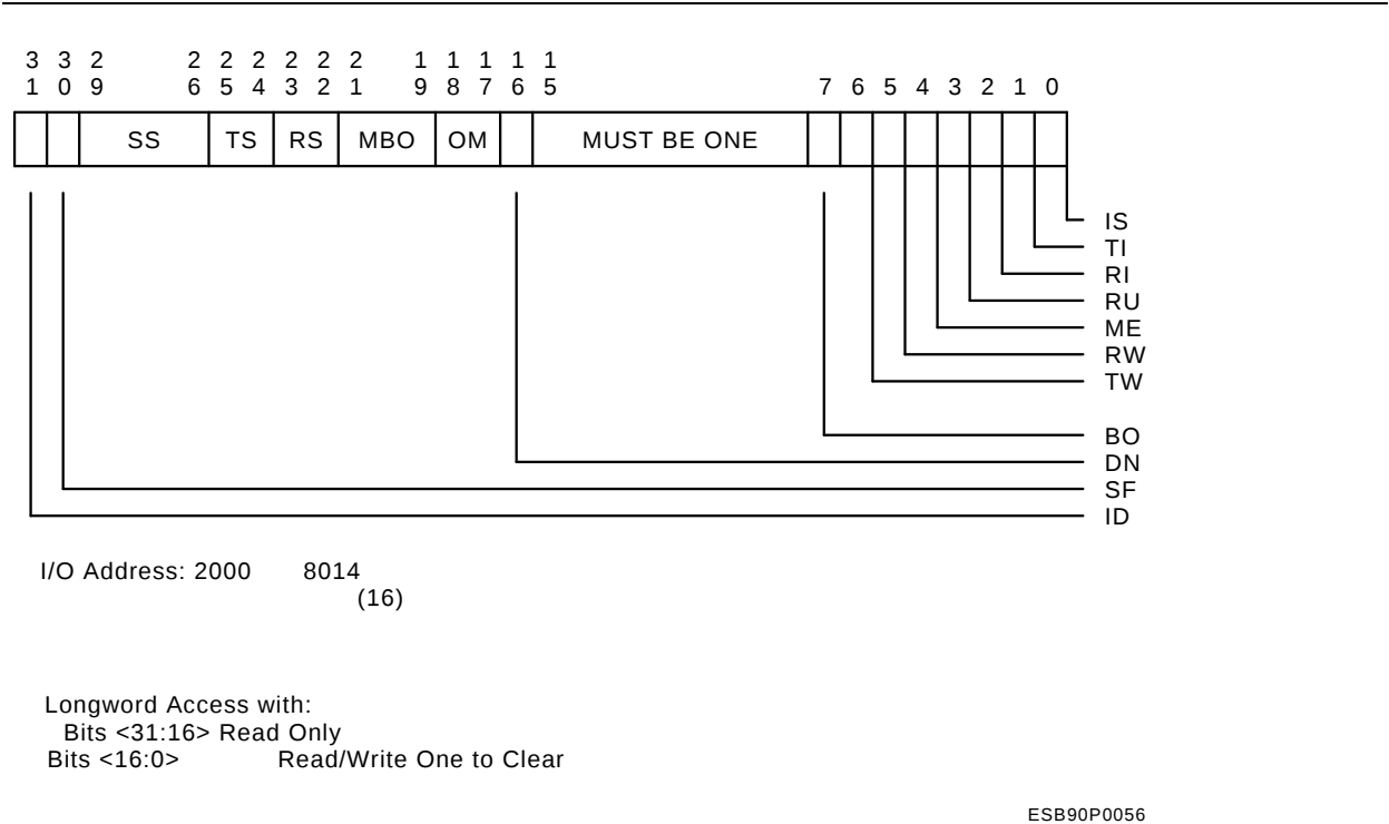
Figure 10–6: NICSR5 bits
