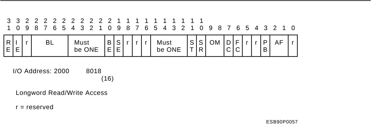
Figure 10–7: NICSR6 format
