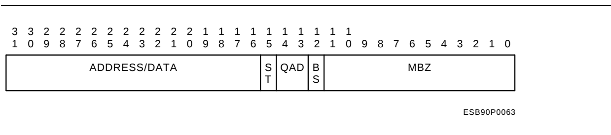
Figure 10–13: NICSr15 format
