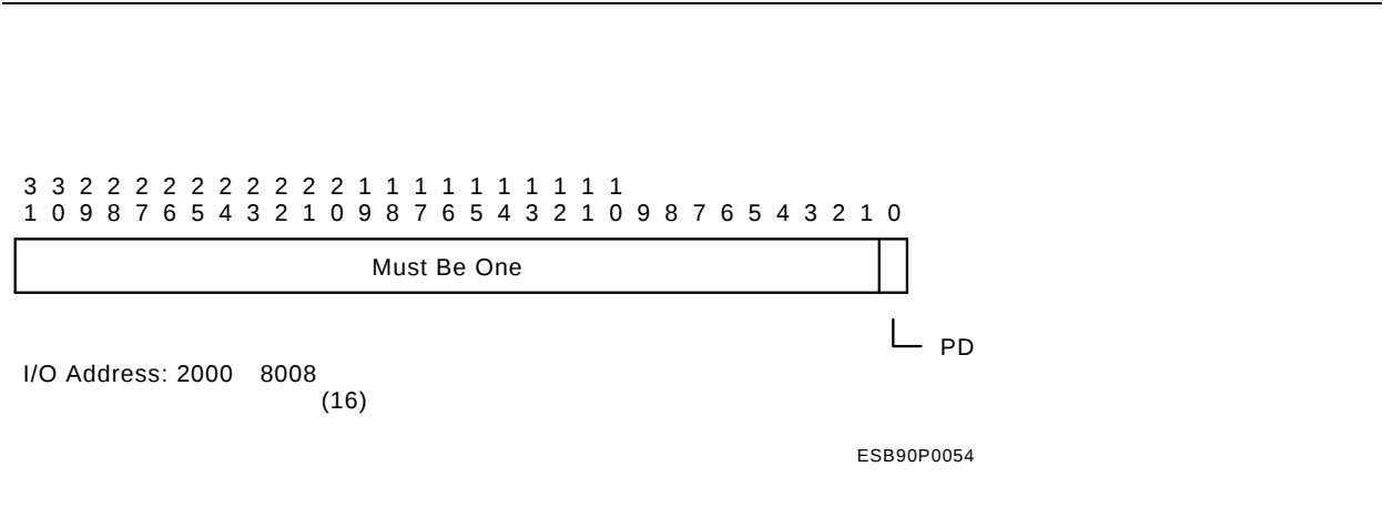
Figure 10–4: NICSR2 format
