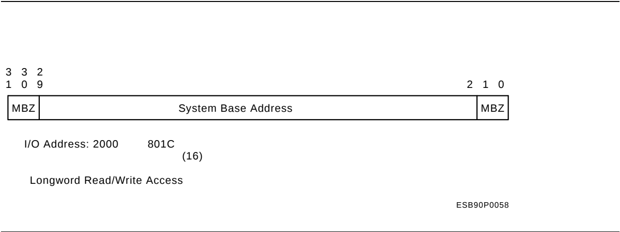
Figure 10–8: NICSR7 format
