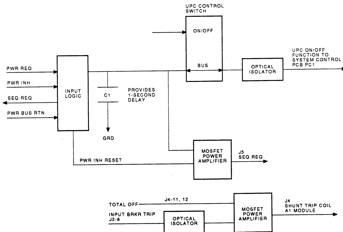
Figure 10-12 Remote Operation
