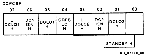
Figure 6-36 PEM DCPCSR
