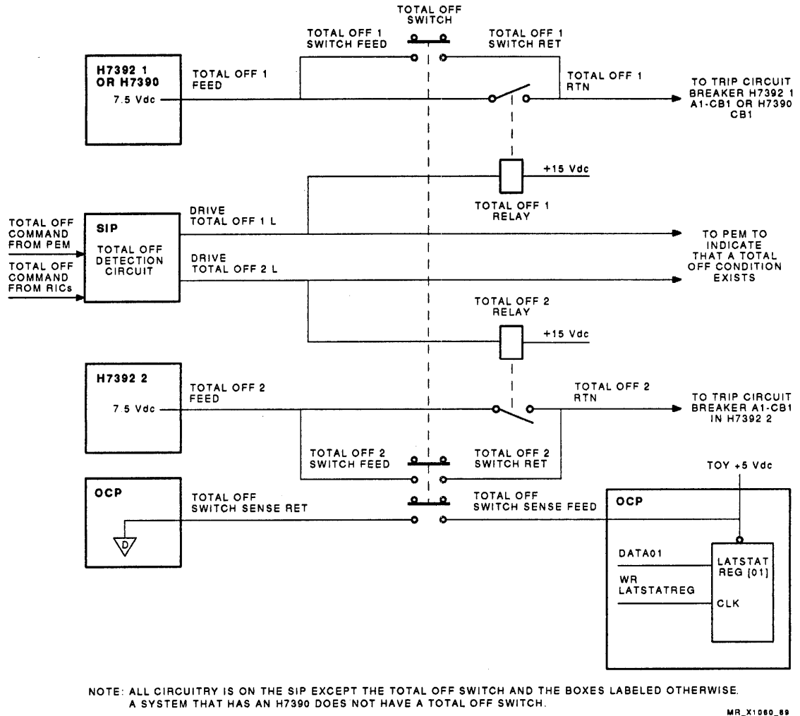
Figure 6-18 SIP Total Off Circuit
