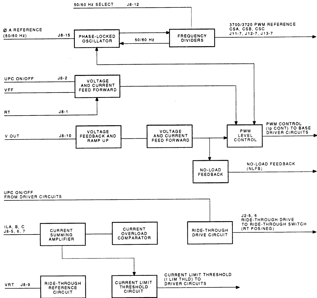
Figure 10-19 PWM Control
