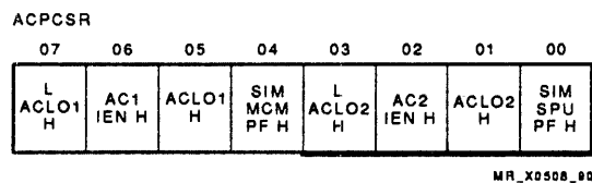
Figure 6-35 PEM ACPCSR
