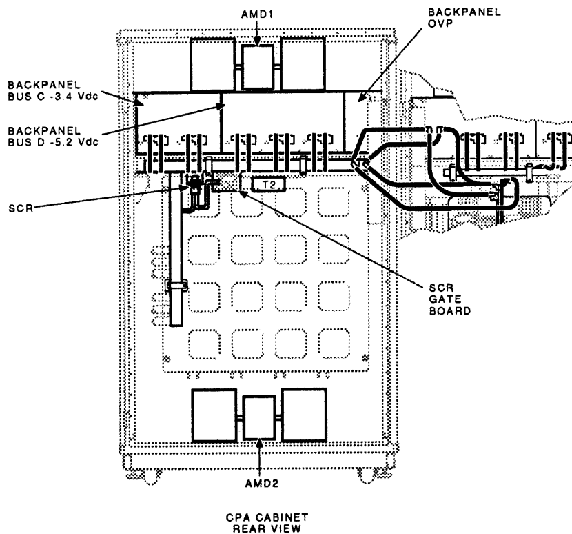
Figure 2-6 Model 210 CPA Cabinet Configuration, Rear View
