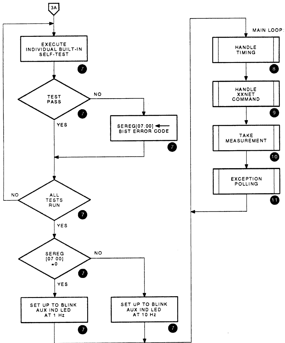
Figure 8-5 (Cont.) RIC Initialization and Diagnostics Flow Diagram
