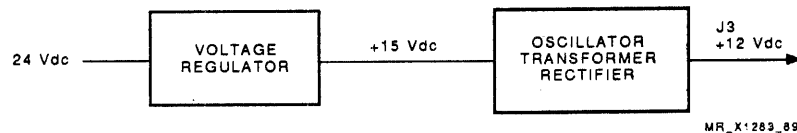
Figure 10-11 12 V Isolated Power Supply
