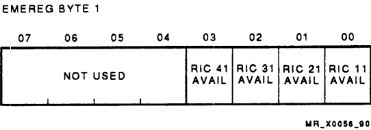
Figure 7-17 EMEREG Byte 1 (Model 400 RICBUS B)
