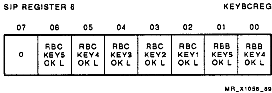
Figure 6-16 SIP Keying B and C Register
