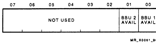
Figure 7-22 EMEREG Byte 6 (BBU Availability)
