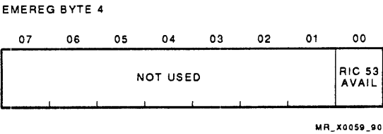
Figure 7-20 EMEREG Byte 4 (Model 210 RICBUS B)
