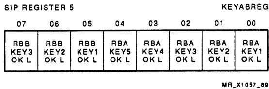
Figure 6-15 SIP Keying A and B Register
