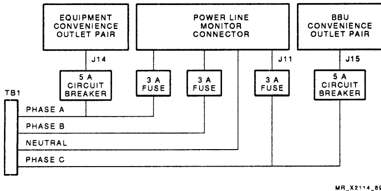
Figure 9-9 Convenience Outlets
