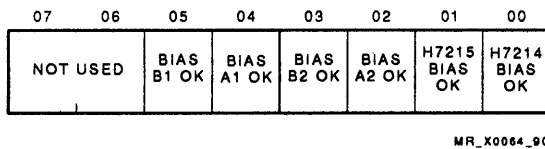
Figure 7-25 EMEREG Byte 9 (Bias OKs)
