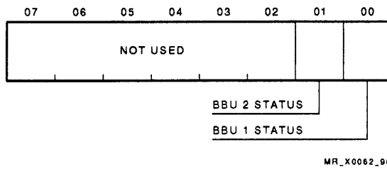
Figure 7-23 EMEREG Byte 7 (BBU Status)
