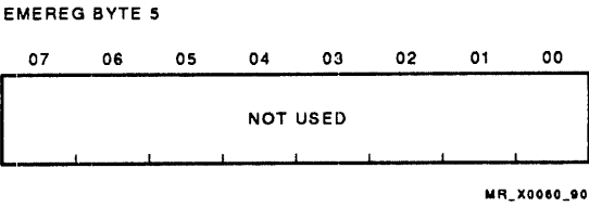
Figure 7-21 EMEREG Byte 5 (Model 210 RICBUS A)
