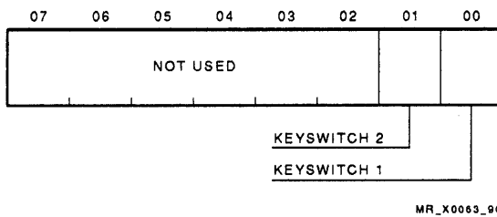
Figure 7-24 EMEREG Byte 8 (Keyswitch)
