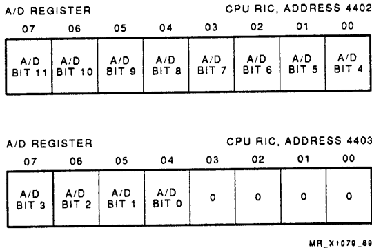
Figure 6-52 A/D Register
