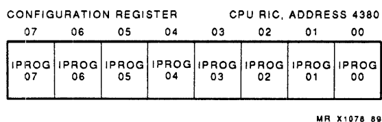
Figure 6-51 CPU RIC Configuration Register
