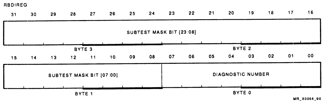
Figure 8-4 RBDIREG Format
