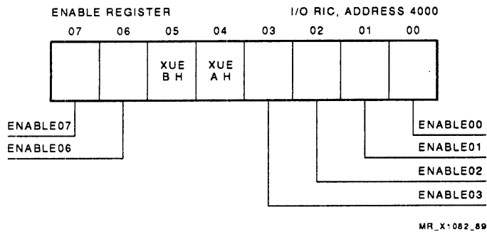
Figure 6-55 I/O RIC Regulator Enable Register
