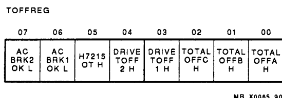
Figure 8-3 PEM TOFFREG
