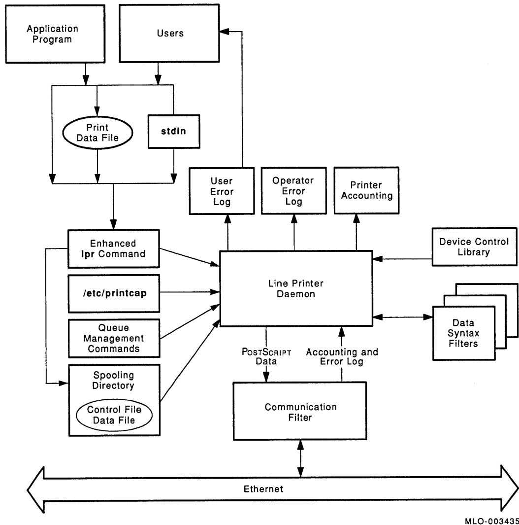
Figure 1-4 PrintServer Client Software on an ULTRIX System
