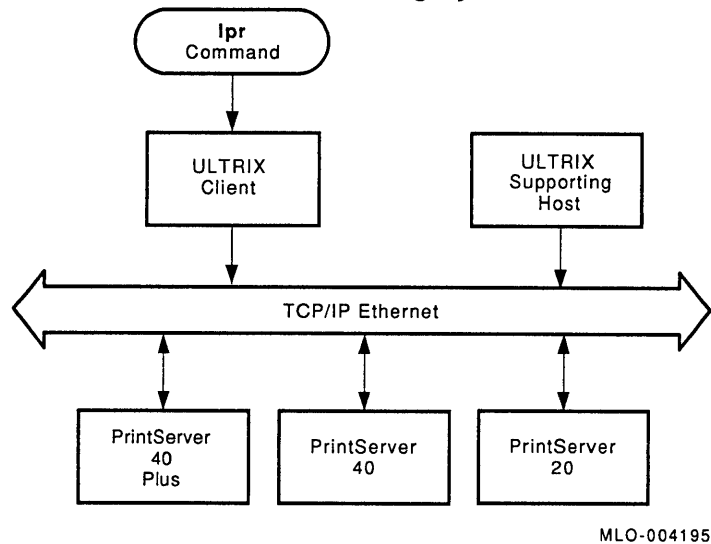
Figure 1–3 PrintServer TCP/IP Printing System
