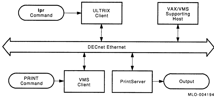
Figure 1–2 PrintServer DECnet Printing System
