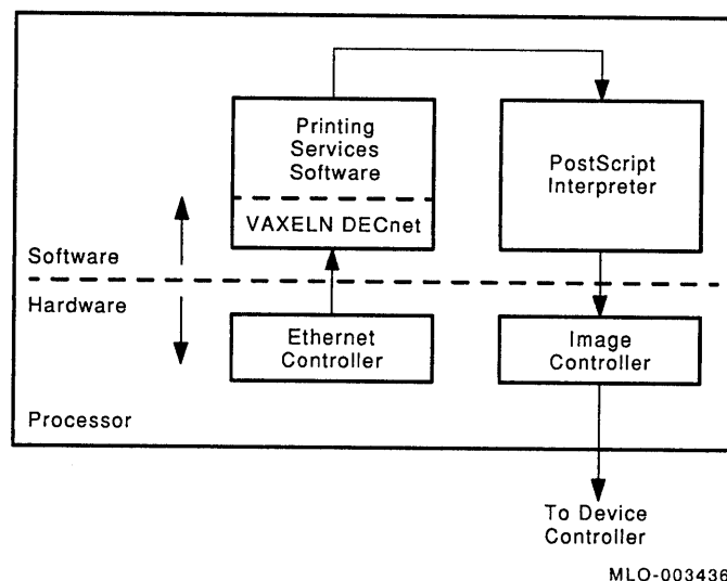
Figure 1-8 PrintServer 40 Data Controller
