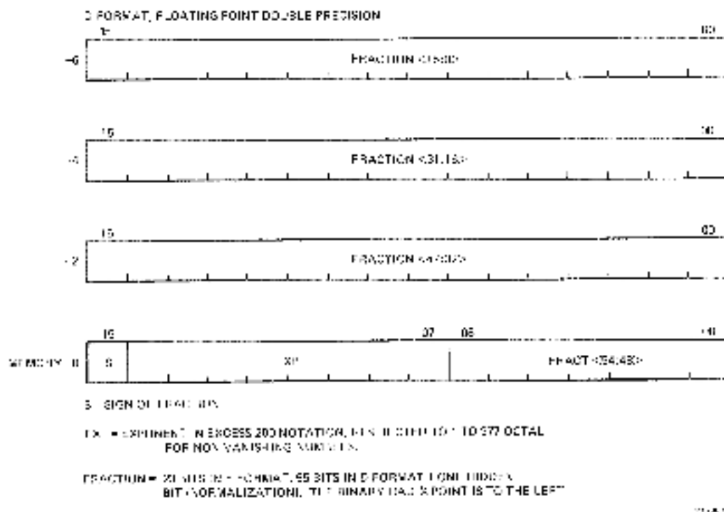
Figure 9-2 Double-Precision Format
