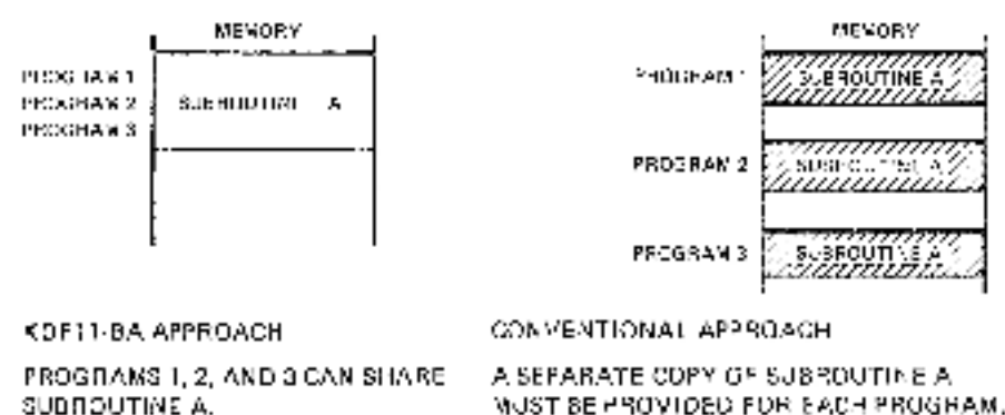
Figure 10-6 Reentrant Routines
