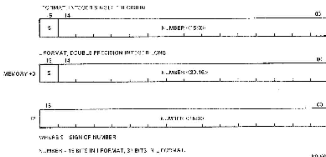
Figure 9-3 2's Complement Format
