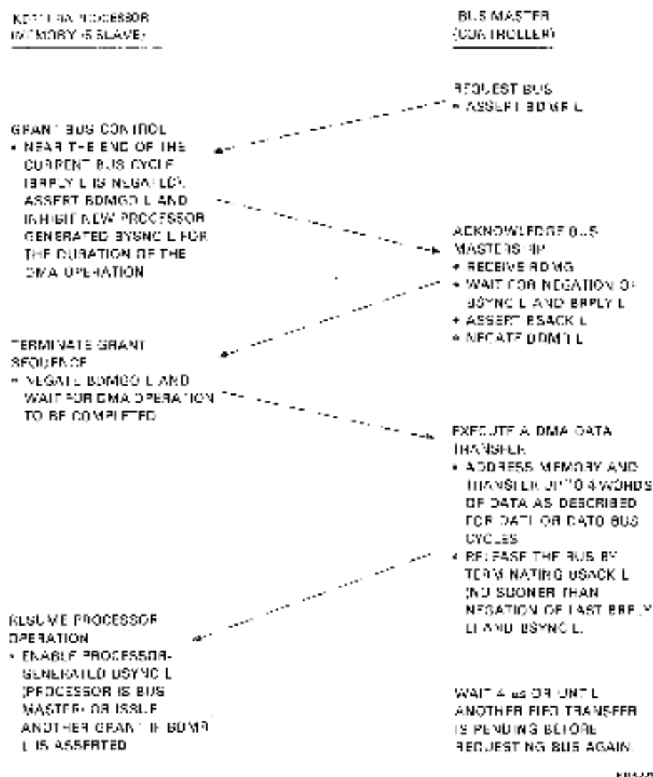
Figure 4-7 DMA Request/Grant Sequence
