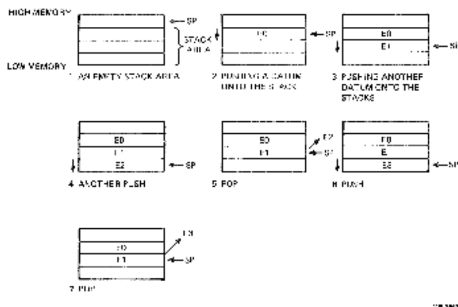
Figure 10-2 Push and Pop Operations
