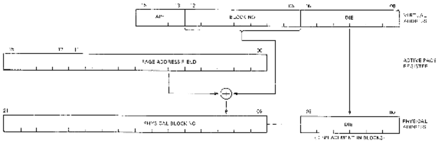
Figure 5-13 Formation of a Physical Address
