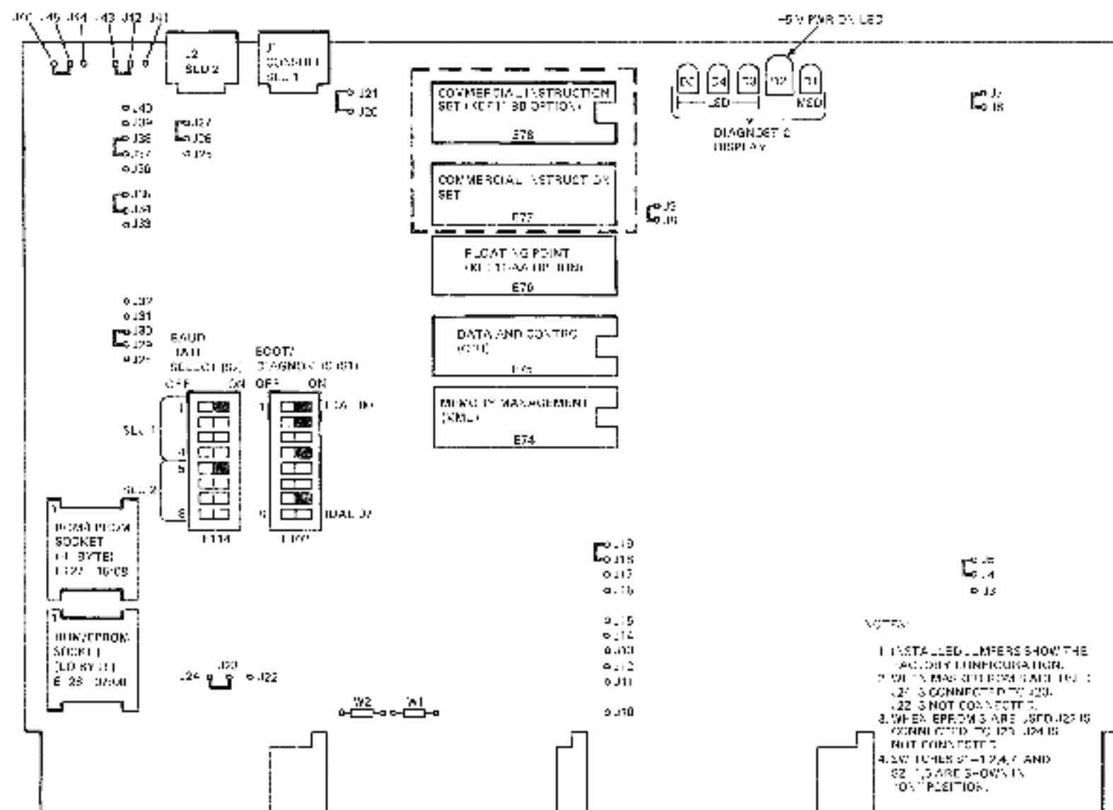
Figure 3-1 KDE11-BA Jumper, Switch, and Diagnostic Display Locations
