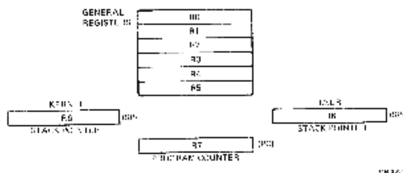
Figure 1-1 General-Purpose Registers
