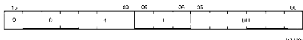
Figure 6-36 Program Control Group JSR
