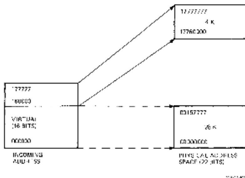
Figure 1-7 16-Bit Mapping
