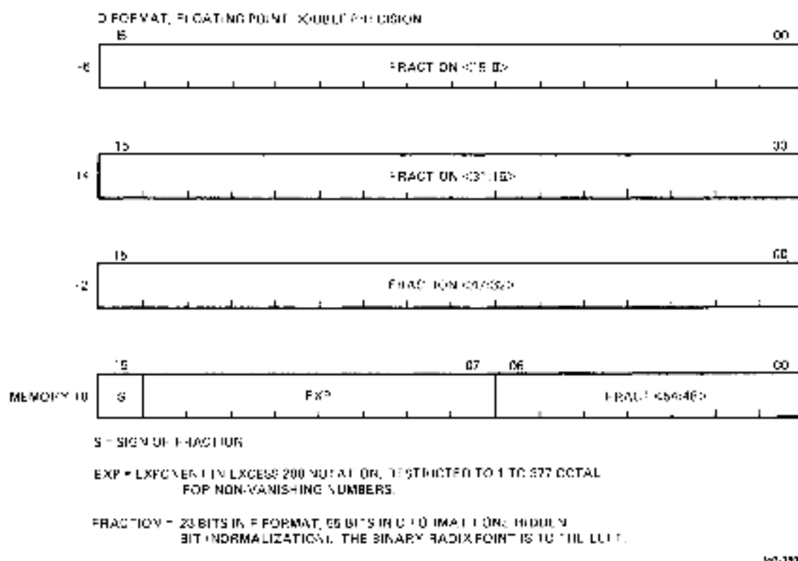
Figure 1-29 Double Precision Format
