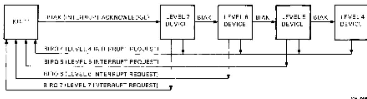
Figure 5-12 Position-Dependent Configuration
