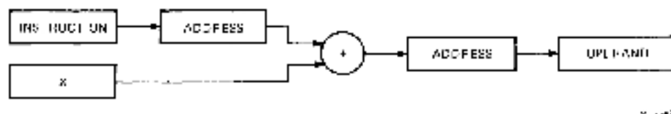
Figure 6-22 Mode 7 Index-Deferred
