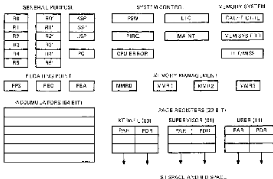
Figure 1-1 Programming Model
