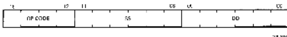
Figure 6-33 Double-Operand Group 1
