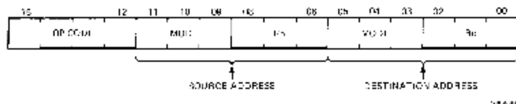
Figure 6-2 Double-Operand Addressing
