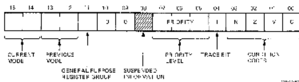
Figure 1-2 Processor Status Register
