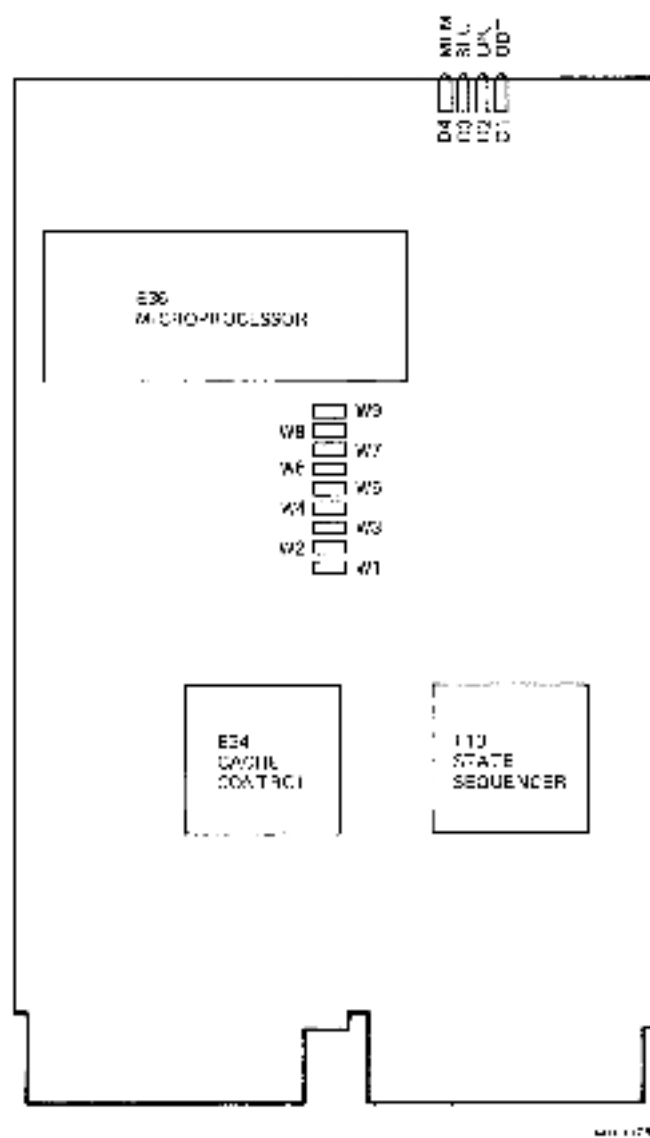
Figure 2-1 KD111-A Jumper Locations
