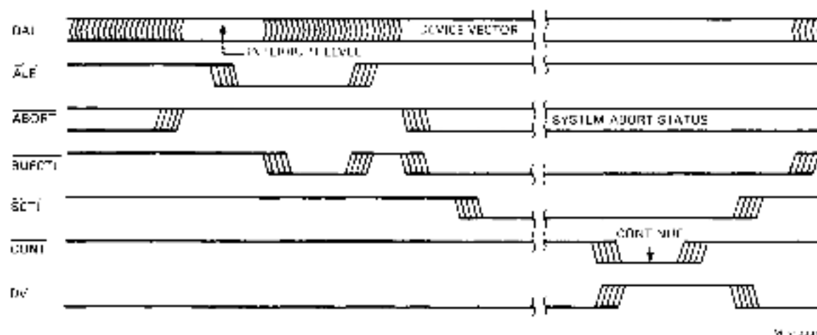
Figure 4-10 Interrupt Acknowledge Transaction:
