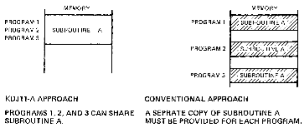
Figure 8-6 Reentrant Routines
