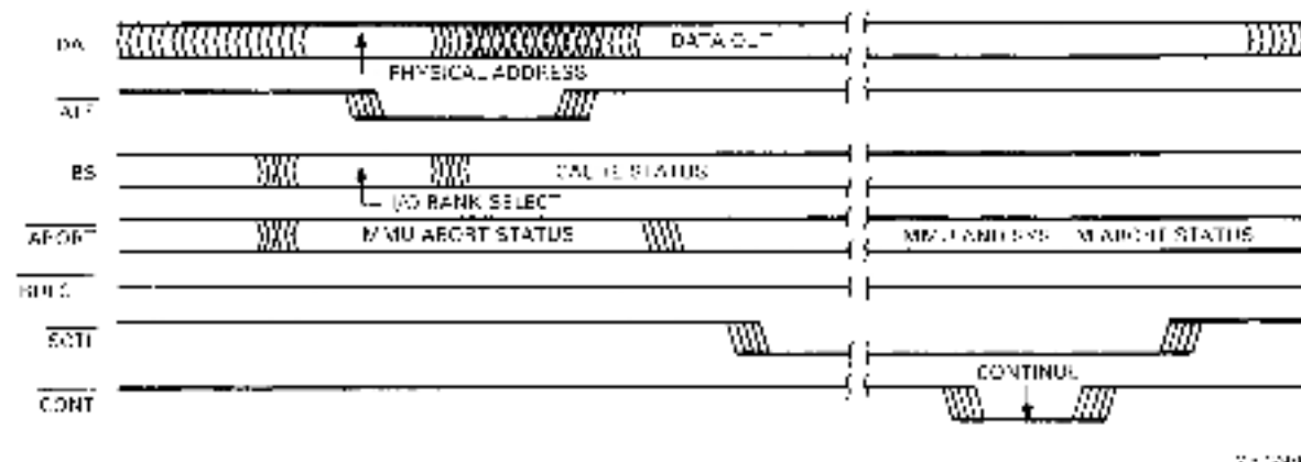
Figure 4-7 Bus Write Transaction
