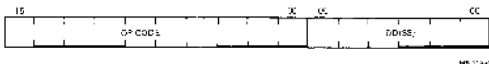
Figure 6-45 Move To And From Previous Instruction/Data Space Group
