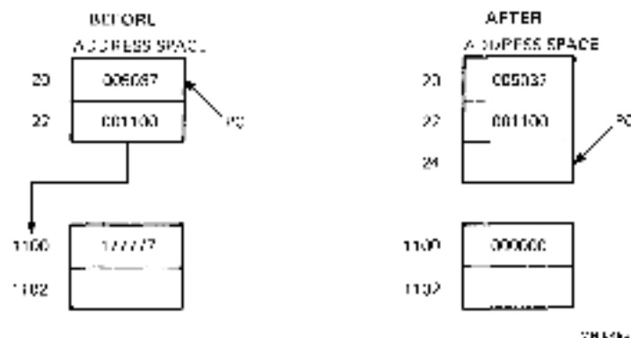
Figure 6-28 CLR @#1100 Clear
