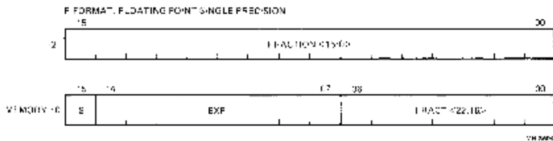
Figure 7-1 Single Precision Format
