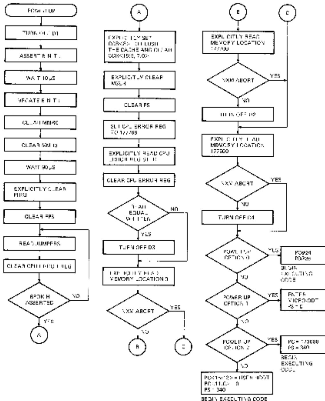
Figure 2-3 KIM-1A Power Up Sequence
