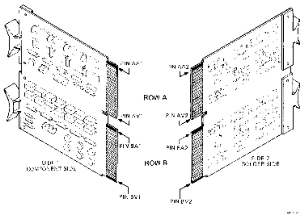
Figure 2-6 KDJ11-A Module Contacts
