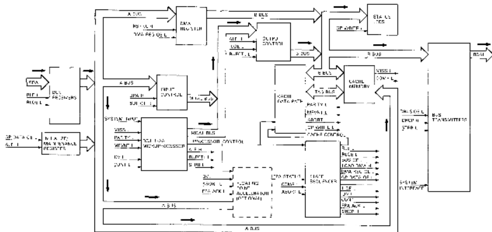
Figure 4-14 Write Data Busing
