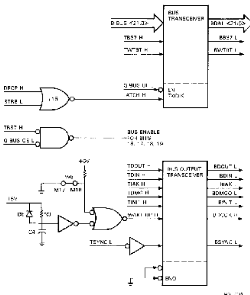
Figure 4-22 KDD11-A Bus Transmitters
