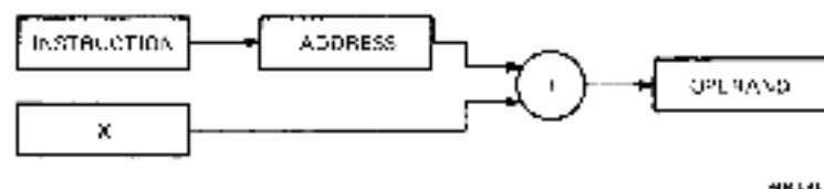
Figure 6-6 Mode 6 Index
