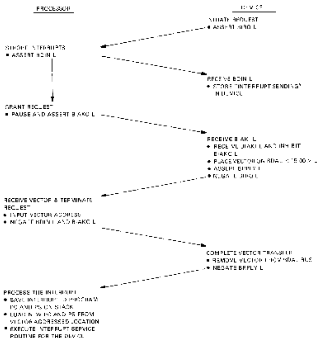
Figure 5-9 Interrupt Request/Acknowledge Sequence
