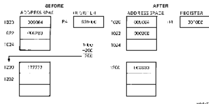
Figure 6-16 CLR 200(R4) Case
