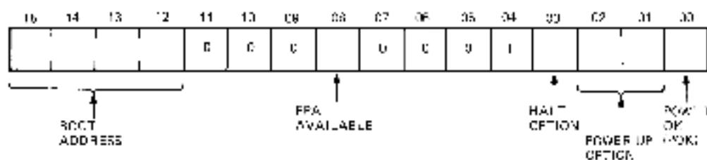
Figure 1-6 Maintenance Register
