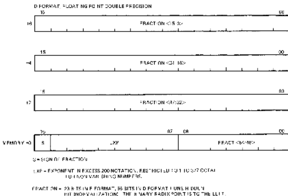
Figure 7-2 Double-Precision Format
