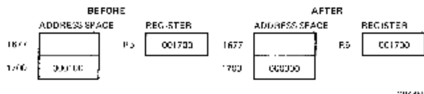
Figure 6-23 CLR @R5 Clear
