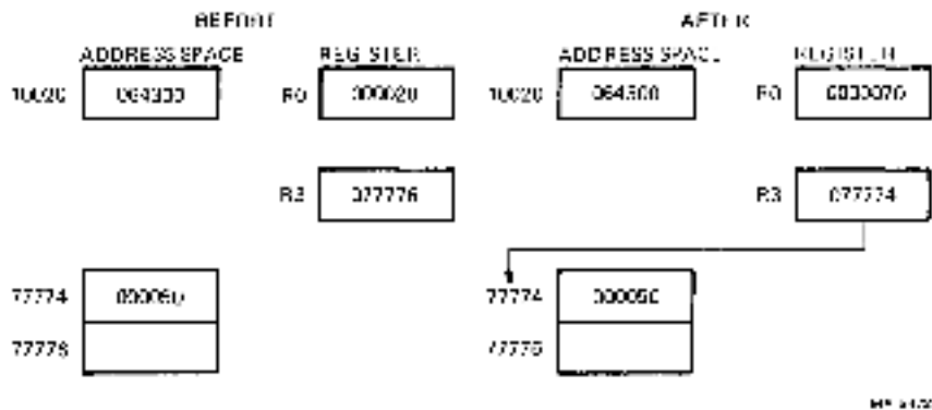
Figure 6-15 ADD \rightarrow (R3),R0 Add
