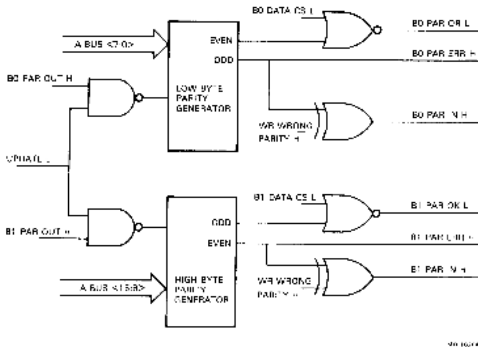
Figure 4-19 Cache Data Parity Logic
