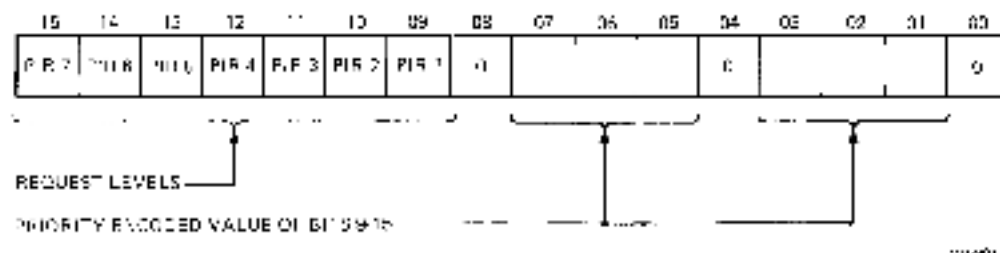
Figure 1-4 Program Interrupt Request Register (PIRQ)
