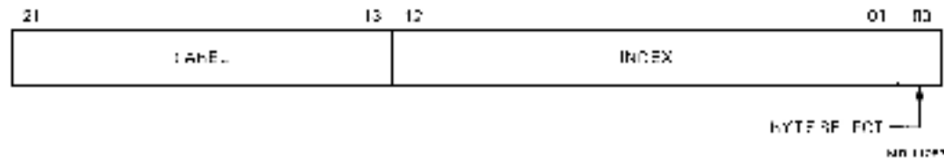
Figure 1-23 Cache Physical Address
