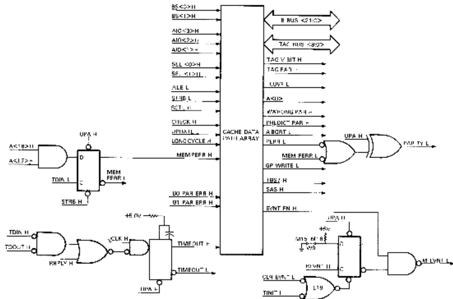
Figure 4-15 Cache Control Logic
