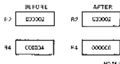
Figure 6-8 ADD R2, R4 Add
