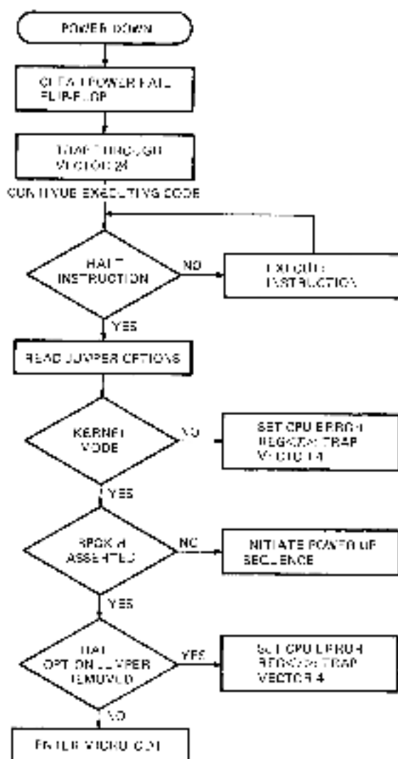
Figure 2-4 RDU-1-A Power-Down Sequence
