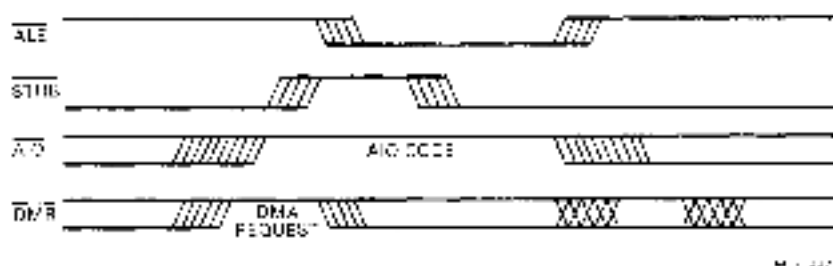
Figure 4-3 NOP Transaction
