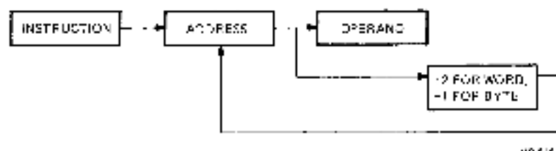
Figure 6-4 Mode 2 Autoincrement
