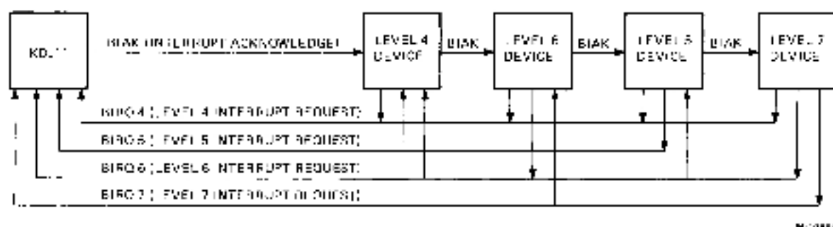
Figure 5-11 Position-Independent Configuration
