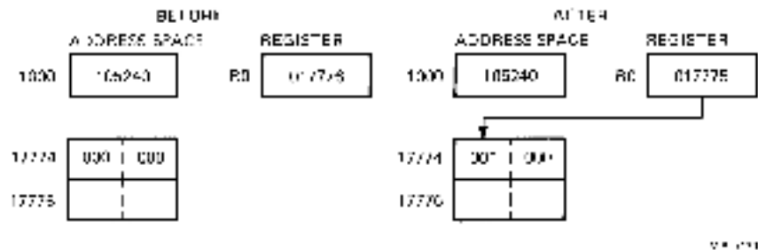
Figure 6-14 INCB \rightarrow (R0) Increment Byte
