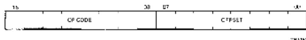
Figure 6-35 Program Control Group Branch
