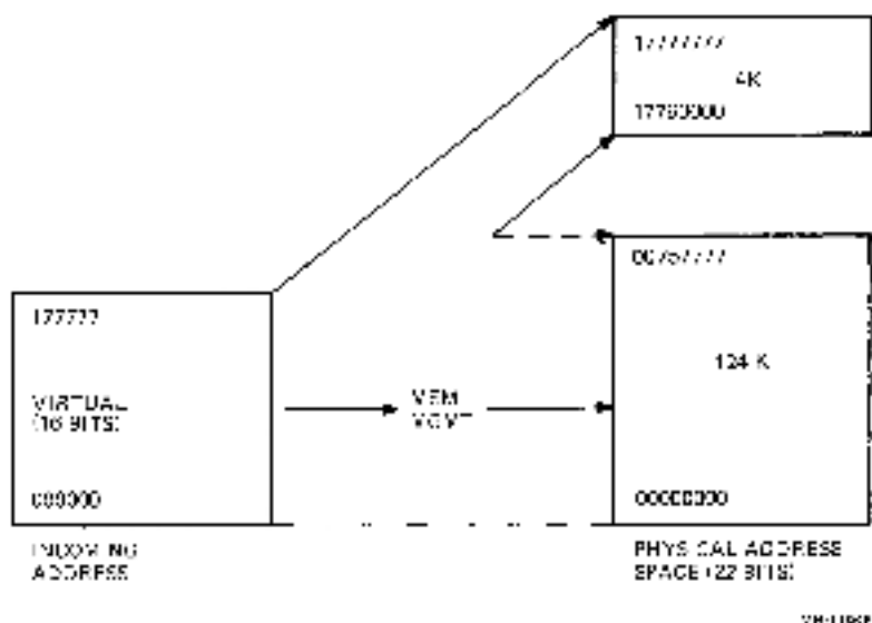
Figure 1-8 18-Bit Mapping
