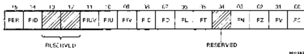
Figure 7-4 Floating-Point Status Register
