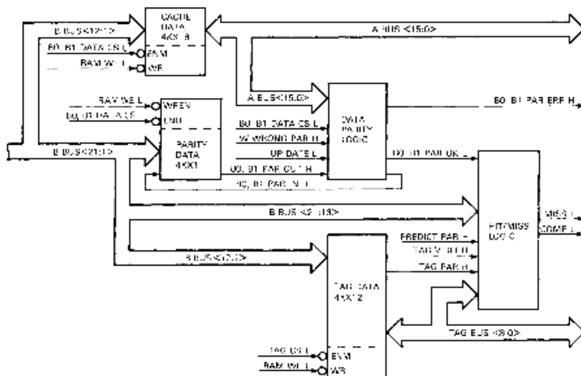
Figure 4-16 Cache Memory
