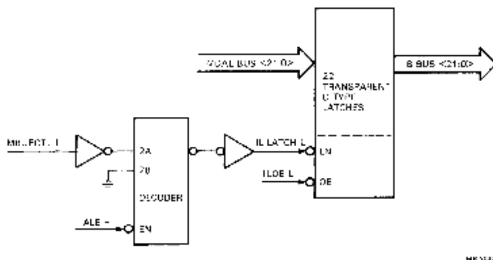
Figure 4-23 DCU11-A Output Control
