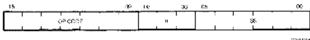
Figure 6-34 Double-Operand Group 2
