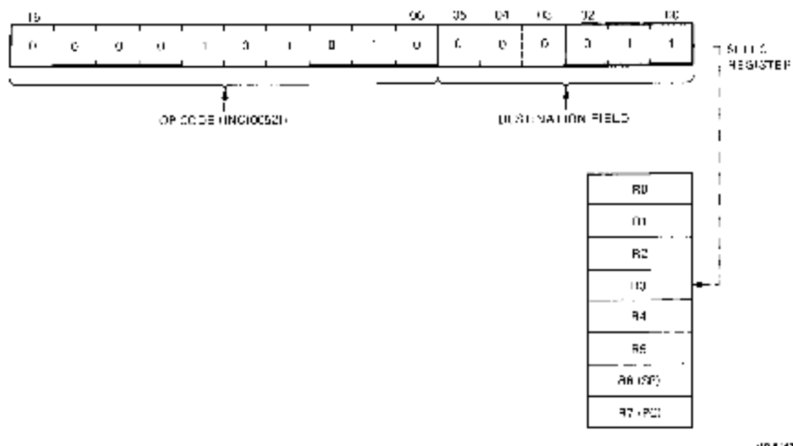
Figure 6-7 INC R3 Instruction
