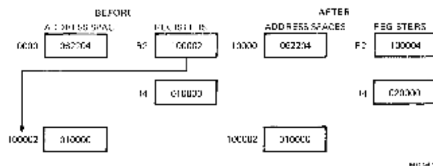
Figure 6-12 ADD (R2),R4 Add
