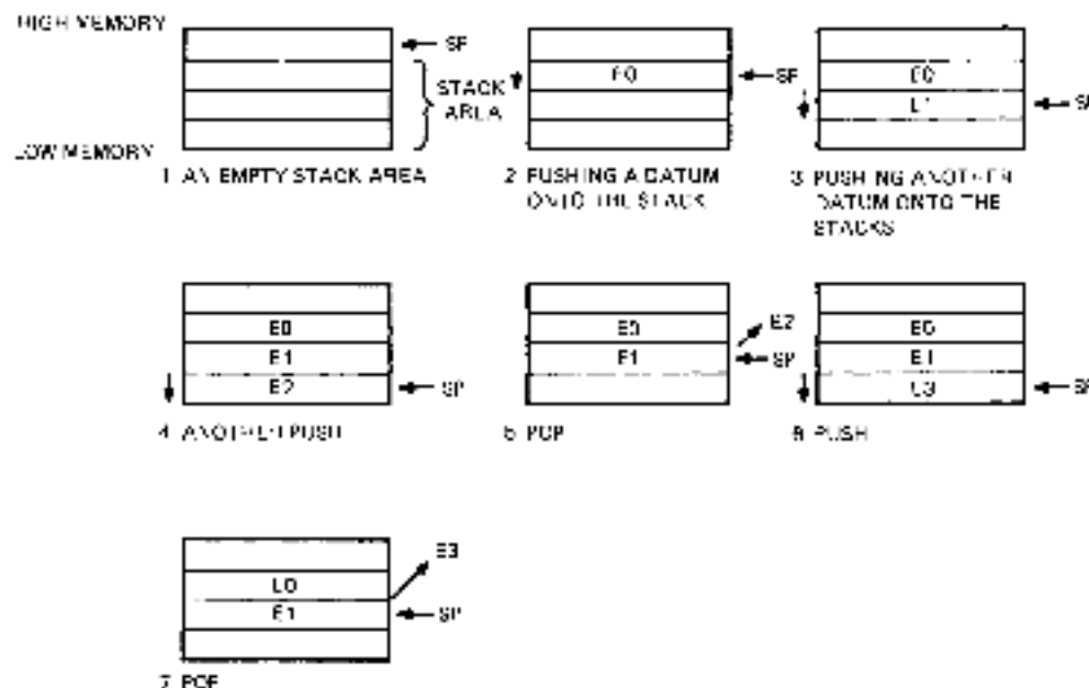
Figure 8-2. Push and Pop Operations
