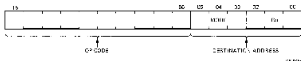
Figure 6-1 Single-Operand Addressing
