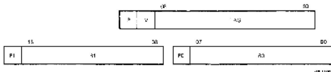
Figure 4-18 Cache Data
