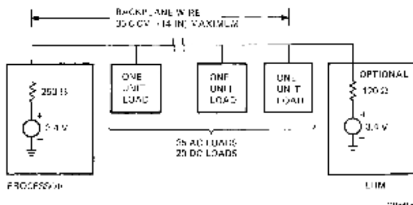
Figure 5-15 Single-Backplane Configuration
