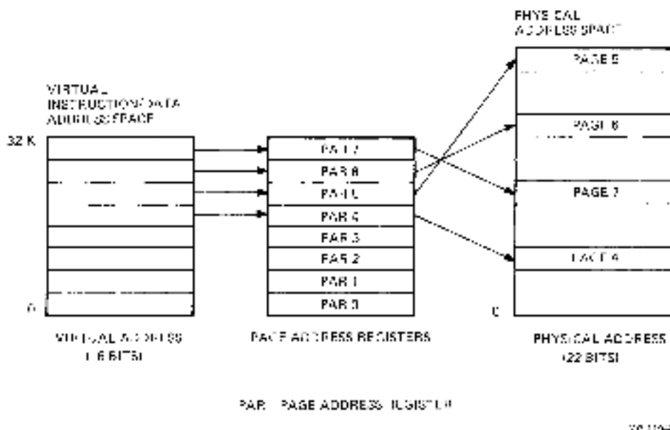
Figure 1-10 Virtual Address Mapping into Physical Address
