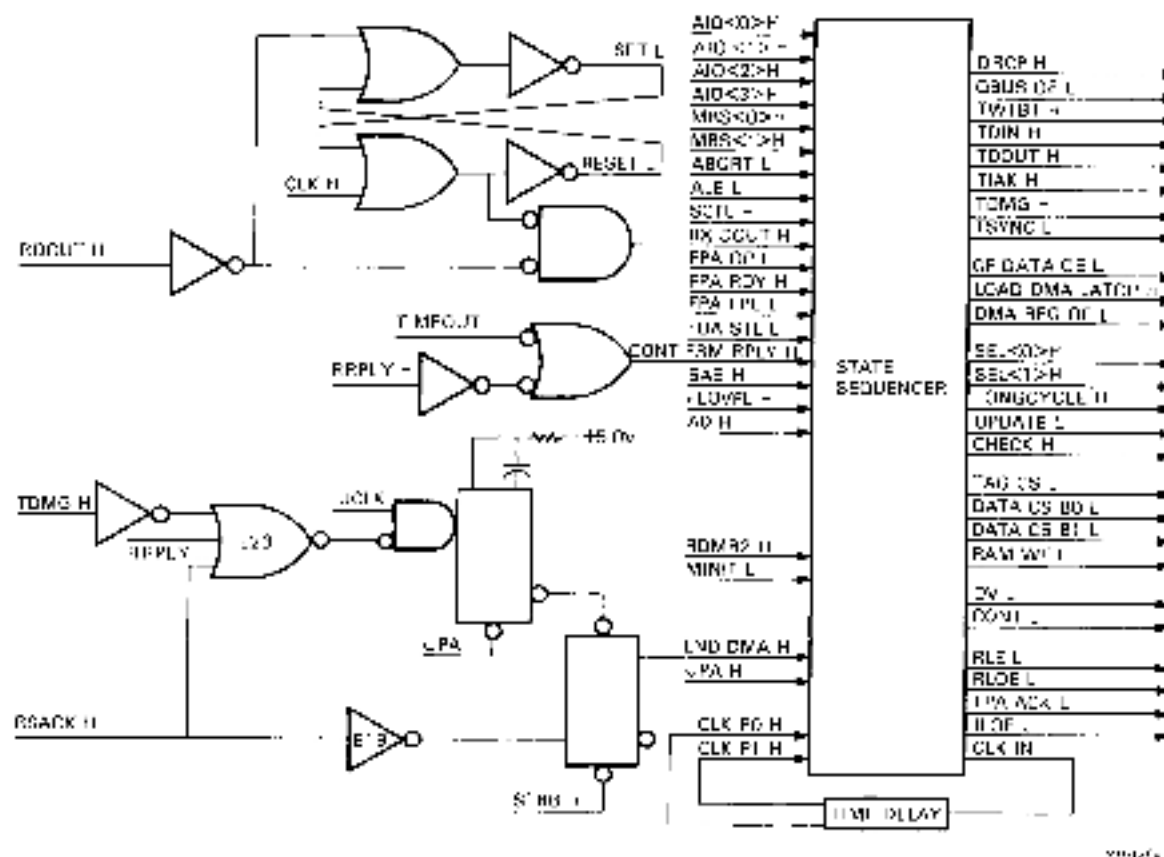
Figure 4-11 State Sequence
