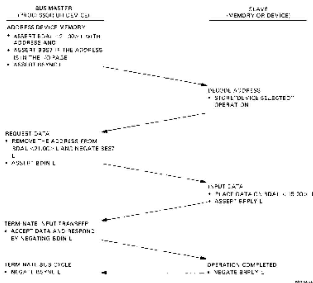
Figure 5-1 DATI Bus Cycle
