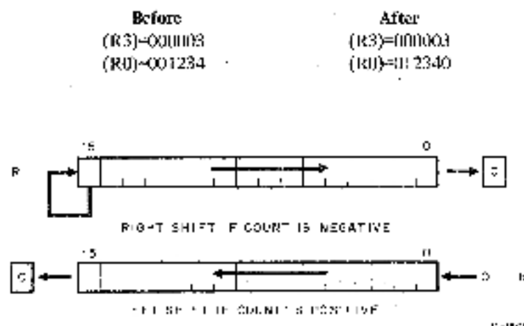
Figure 2-3 ASH Operation
