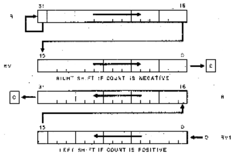
Figure 2-4 ASHC Operation
