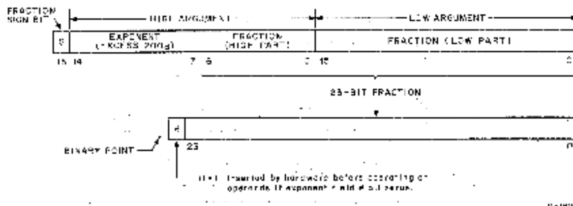
Figure 2-5 FIS Number Format
