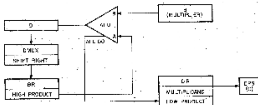
Figure 4-9. MUL Flow, Block Diagram
