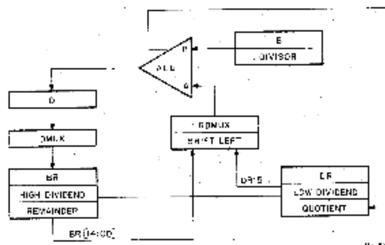
Figure 4-10 DIV Flow Block Diagram
