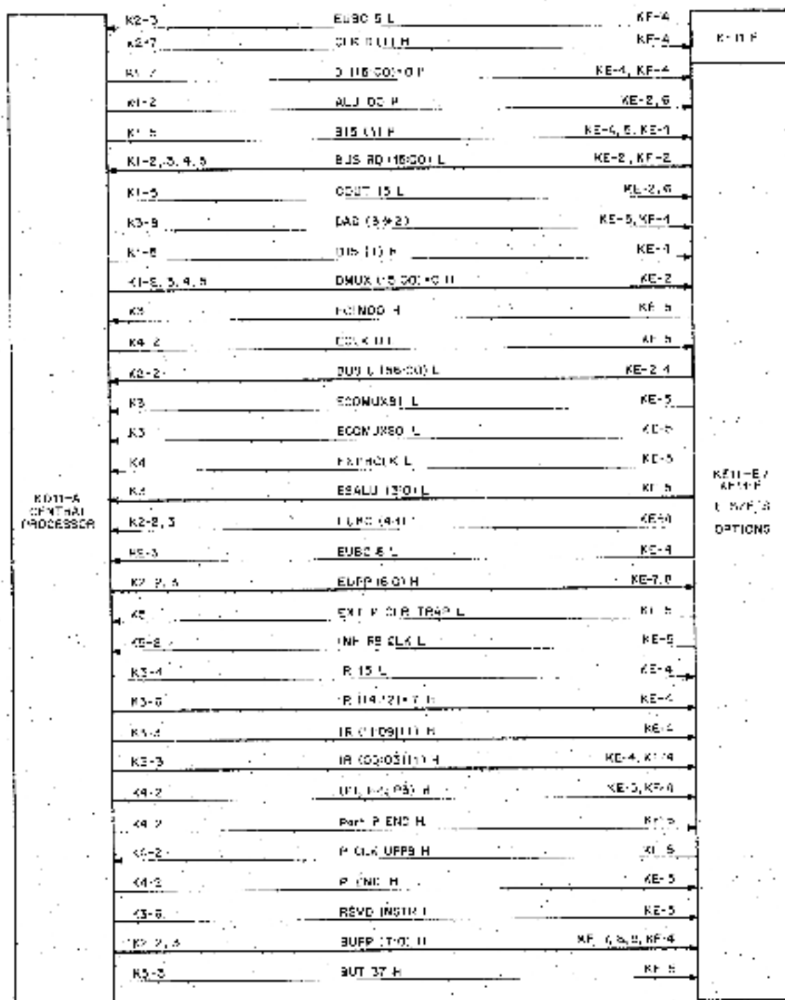
Figure 4-2 KD11-E/F/KD11-A Interfacing Signals
