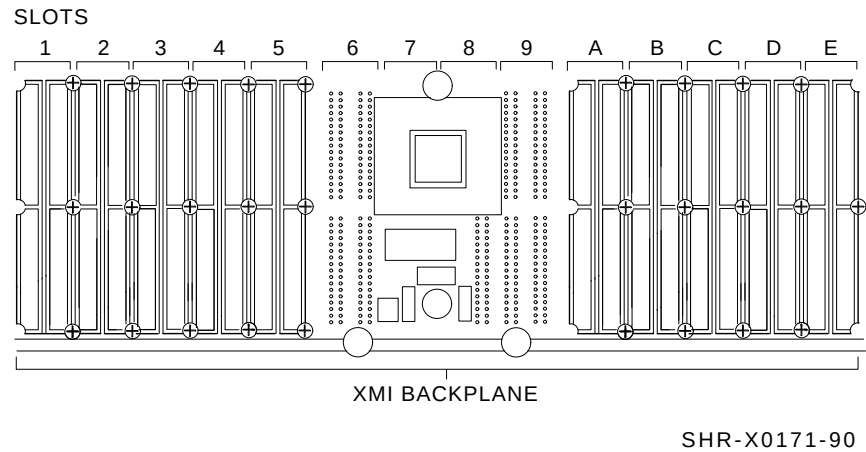
Figure 1-8 XMI Backplane (VAX 6000 Series)
