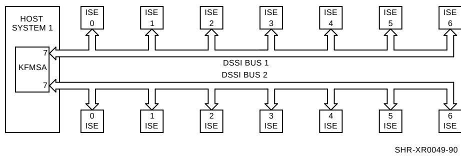
Figure 1-2 Single System DSSI Configuration
