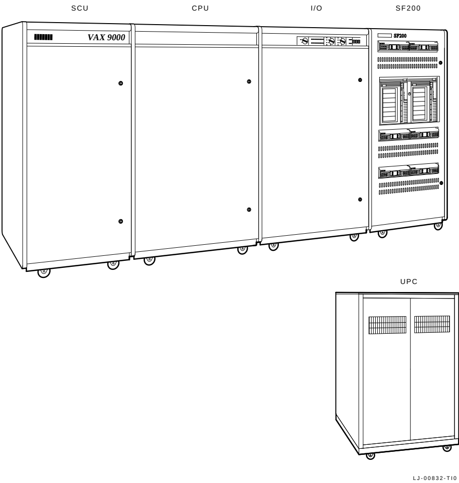
Figure 1-5 VAX 9000 Model 200 System
