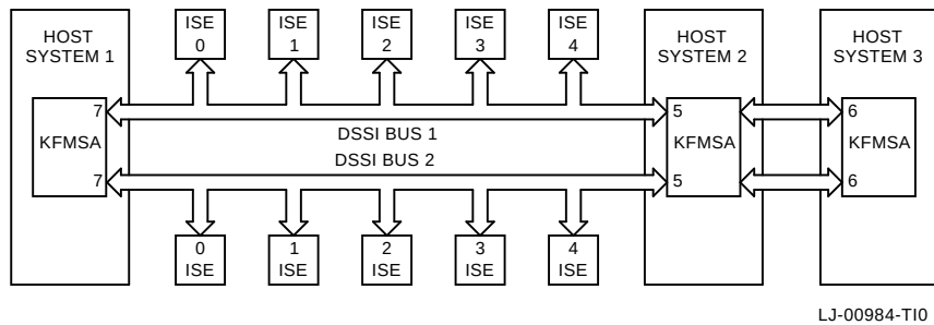
Figure 1-3 DSSI VAXcluster Configuration
