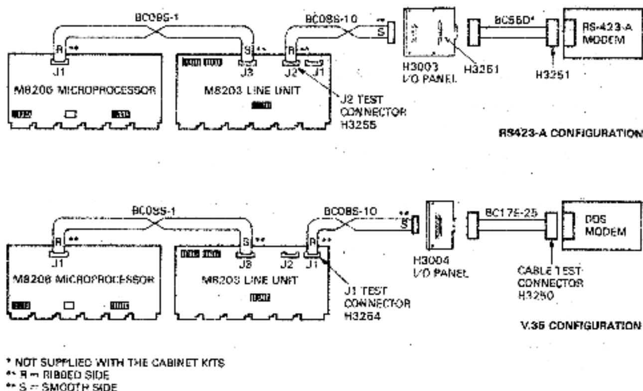
Figure 2-11 Remote System Cable Diagram for RS-423 and V.35
