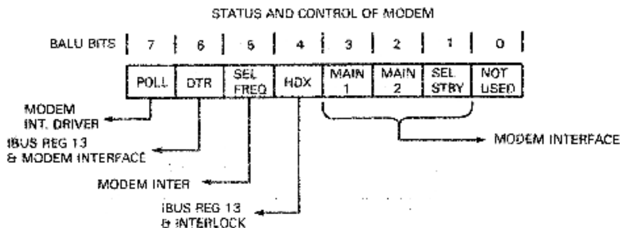
Figure 3-13 OBUS Register 13
