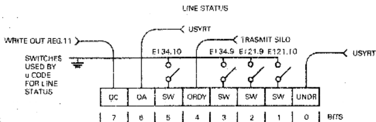
Figure 3-8 IBUS Register 11
