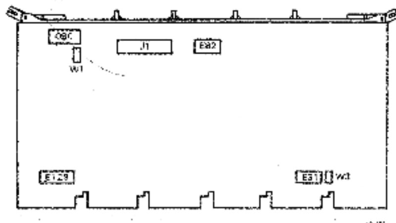
Figure 2-1 M8206 (KMC11-B) Switch and Jumper Locations
