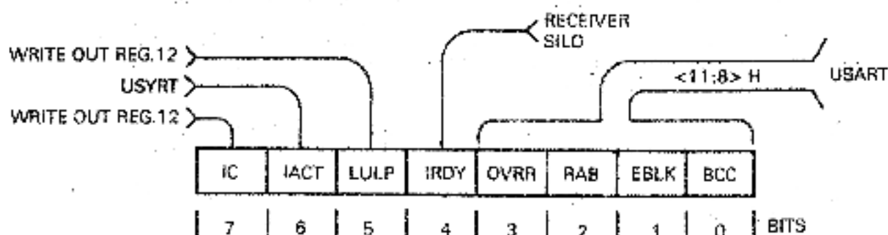
Figure 3-10 IBUS Register 12
