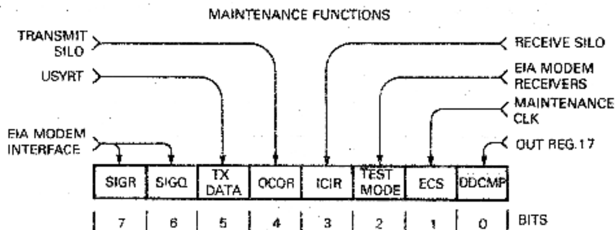
Figure 3-20 IBUS Register 17
