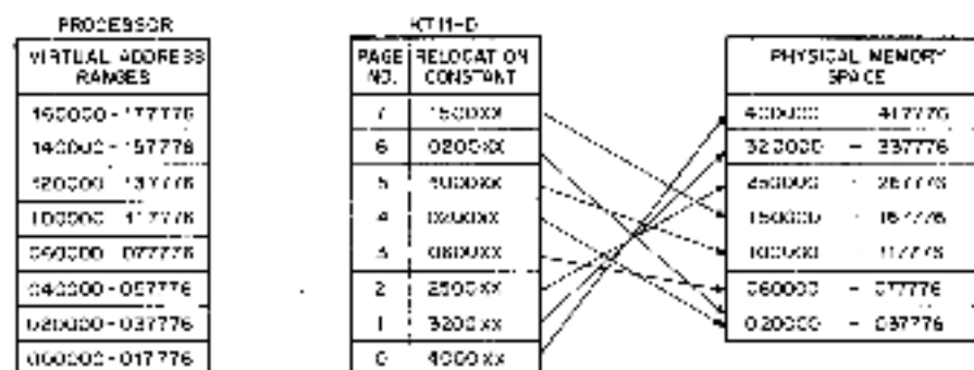
Figure 3-2 Relocation of a 32K Word Program Into 124K Word Physical Memory
