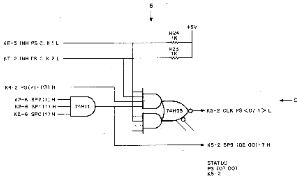
Figure 2-12 KT-2 INH PS CLK 2 L Hook in KD11-A
