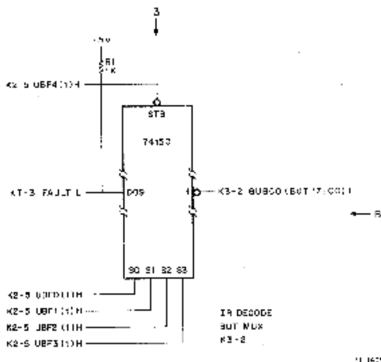
Figure 2-7 KT-3 Fault II Hook in KD11-A
