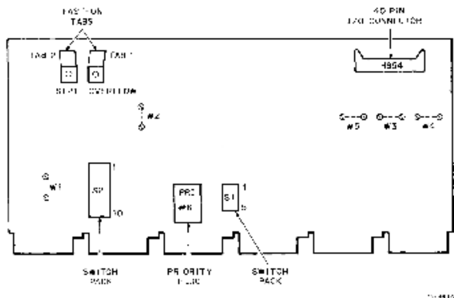
Figure 2-9 M7025 Module Component Locations
