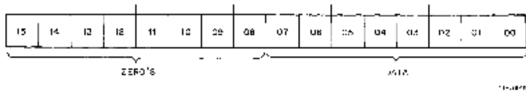
Figure 3-5 B Preset Register
