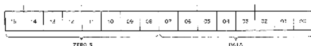
Figure 3-3 B Counter
