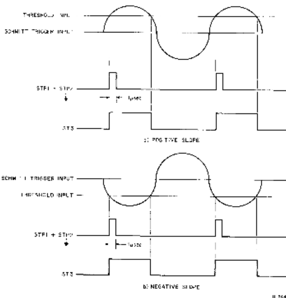
Figure 2-7 Schmitt Trigger Slope Relationship
