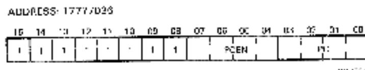
Figure 5-13 Port C Data Register
