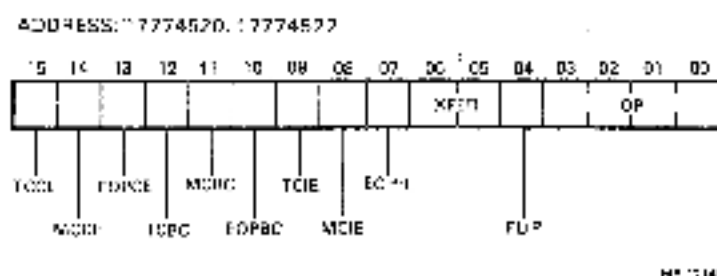
Figure 4-15 Channel Mode Low
