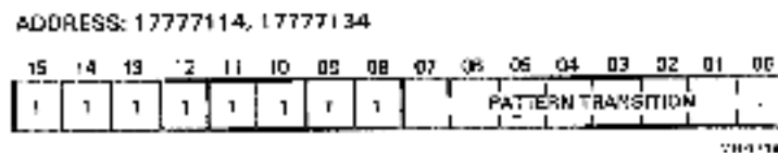
Figure 5-10 Pattern Transition Registers (Ports A and B)
