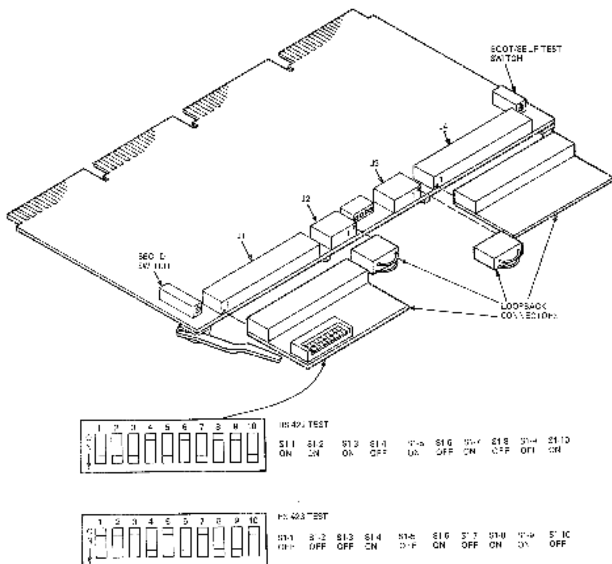
Figure 2-25 Loopback Connectors
