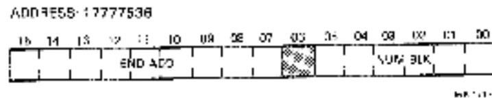
Figure 3-18 KXJ11 Control/Status Register II
