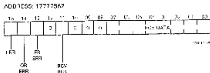
Figure 6-2 Receiver Buffer Register (RBUF)
