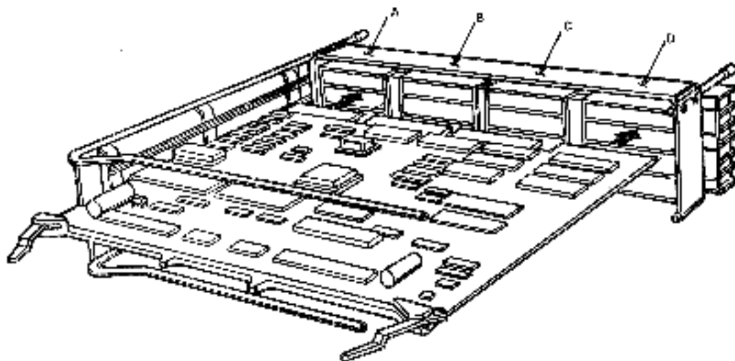
Figure 2-20 Backplane Installation
