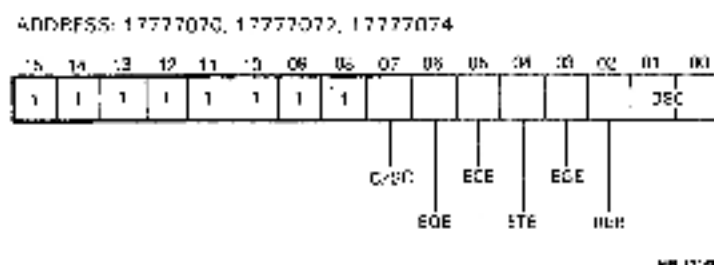
Figure 5-14 Counter/Timer Mode Specification (Counter/Timers 1, 2, and 3)
