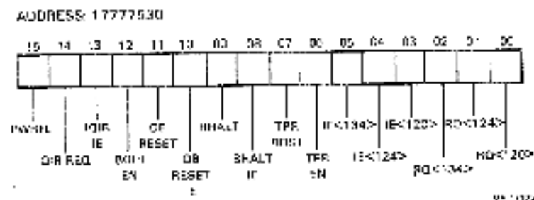
Figure 3-16 KXJ11 Control/Status Register D
