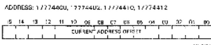
Figure 4-4 Current A or B Address Offset
