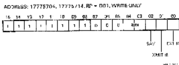
Figure 6-10 Control Register 1
