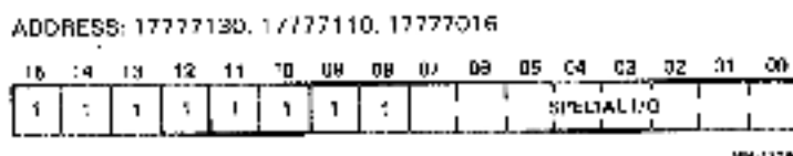
Figure 5-8 Special I/O Registers (Ports A, B, and C)
