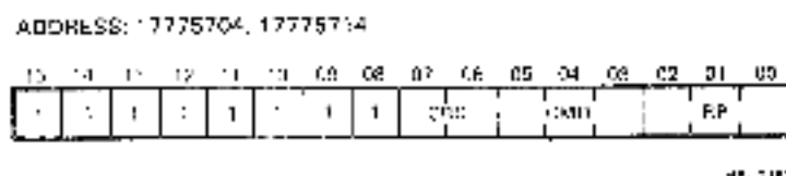
Figure 6-9 Control Register 0
