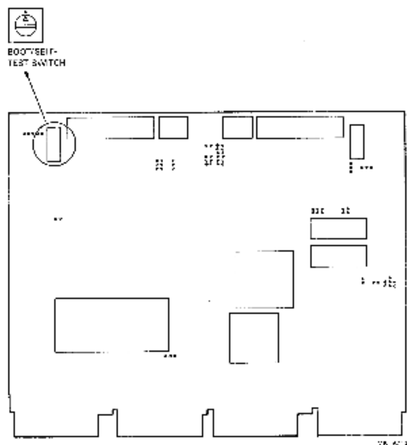
Figure 2-4 Boot/Self-test Switch
