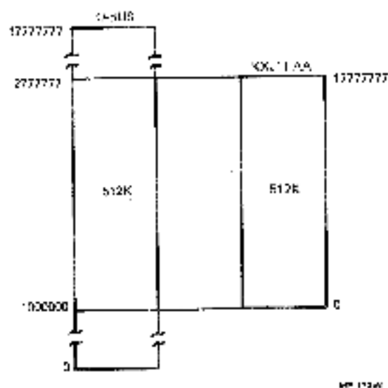
Figure 3-33 Defining 64 Blocks of Shared Memory
