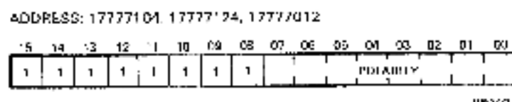
Figure 5-6 Data Path Polarity Registers (Ports A, B, and C)
