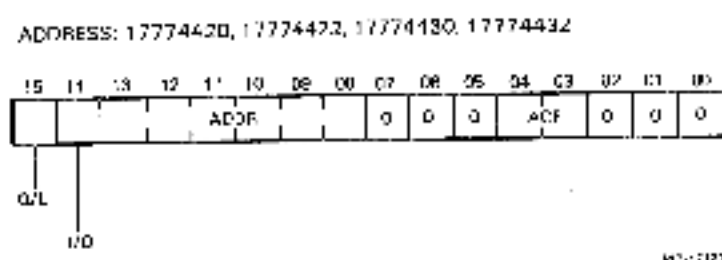
Figure 4-3 Current A or B Address Segment/Tag
