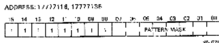
Figure 5-11 Pattern Mask Registers (Ports A and B)
