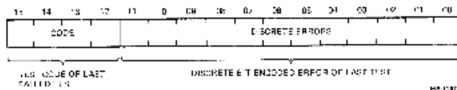
Figure 3-6 TPR3 as a Test Result Register
