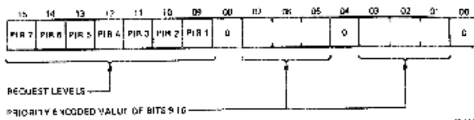
Figure 3-22 PIRQ Register
