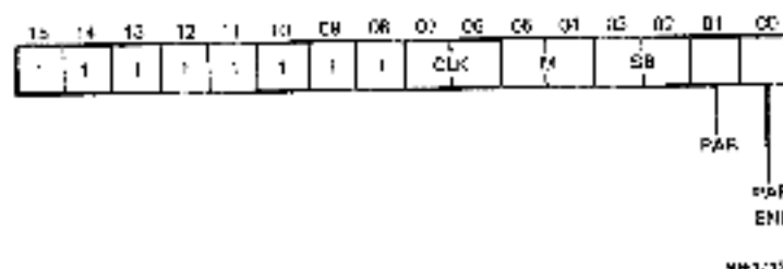
Figure 6-14 Control Register 4
