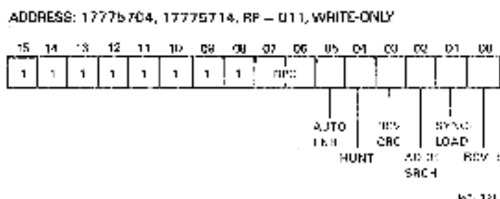
Figure 6-13 Control Register 3
