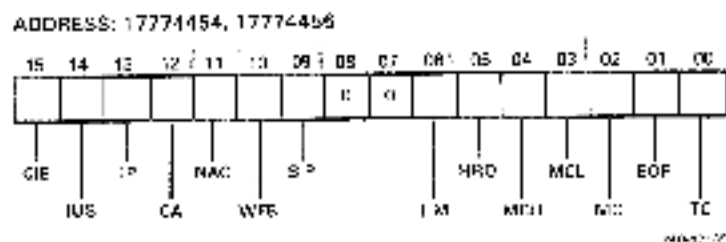
Figure 4-9 Status Register
