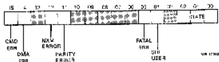
Figure 3-8 TPR1
