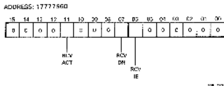
Figure 6-1 Receiver Control/Status Register (RCSR)
