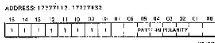
Figure 5-9 Pattern Polarity Registers (Ports A and B)
