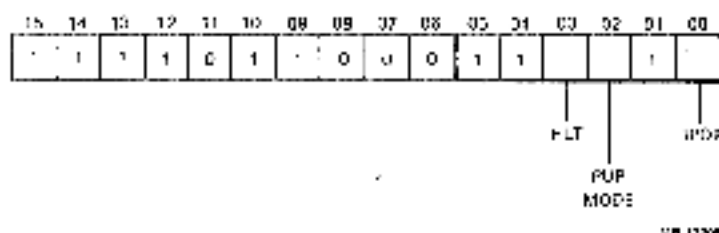
Figure 3-21 Maintenance Register
