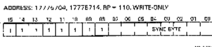
Figure 6-16 Control Register 6
