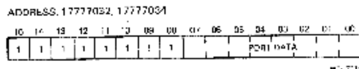
Figure 5-12 Port Data Registers (Ports A and B)
