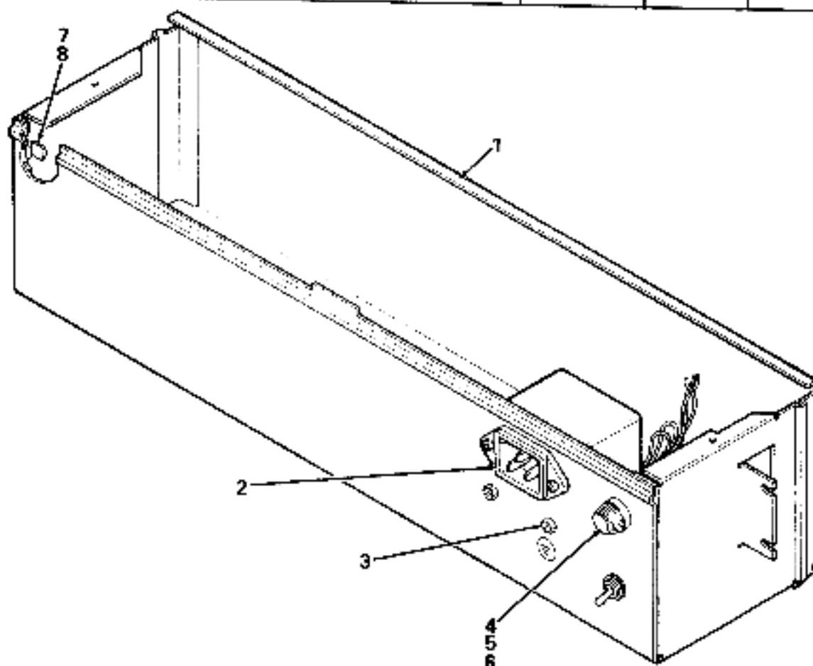
Figure 21. Chassis Assembly
