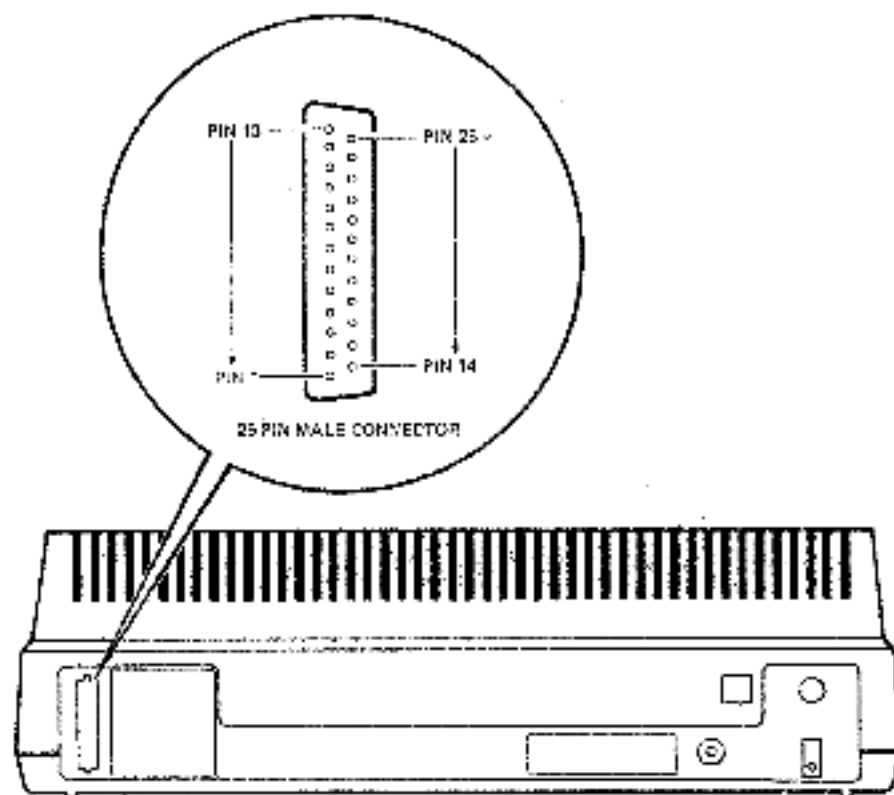
Figure 1-2 EIA Connector
