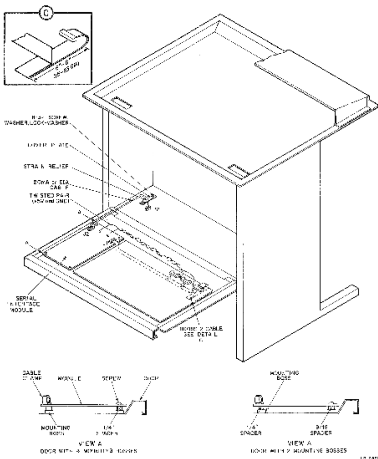
Figure 13 Module Installation on LA130 Rear Door
