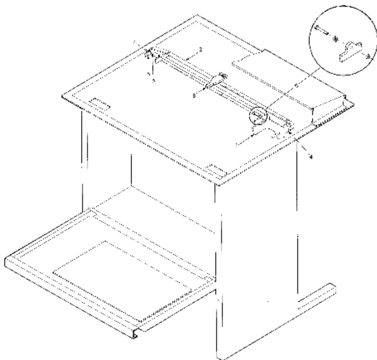
Figure 21 Installation of Compressed Front Option Kit (LAXX-KJ)
