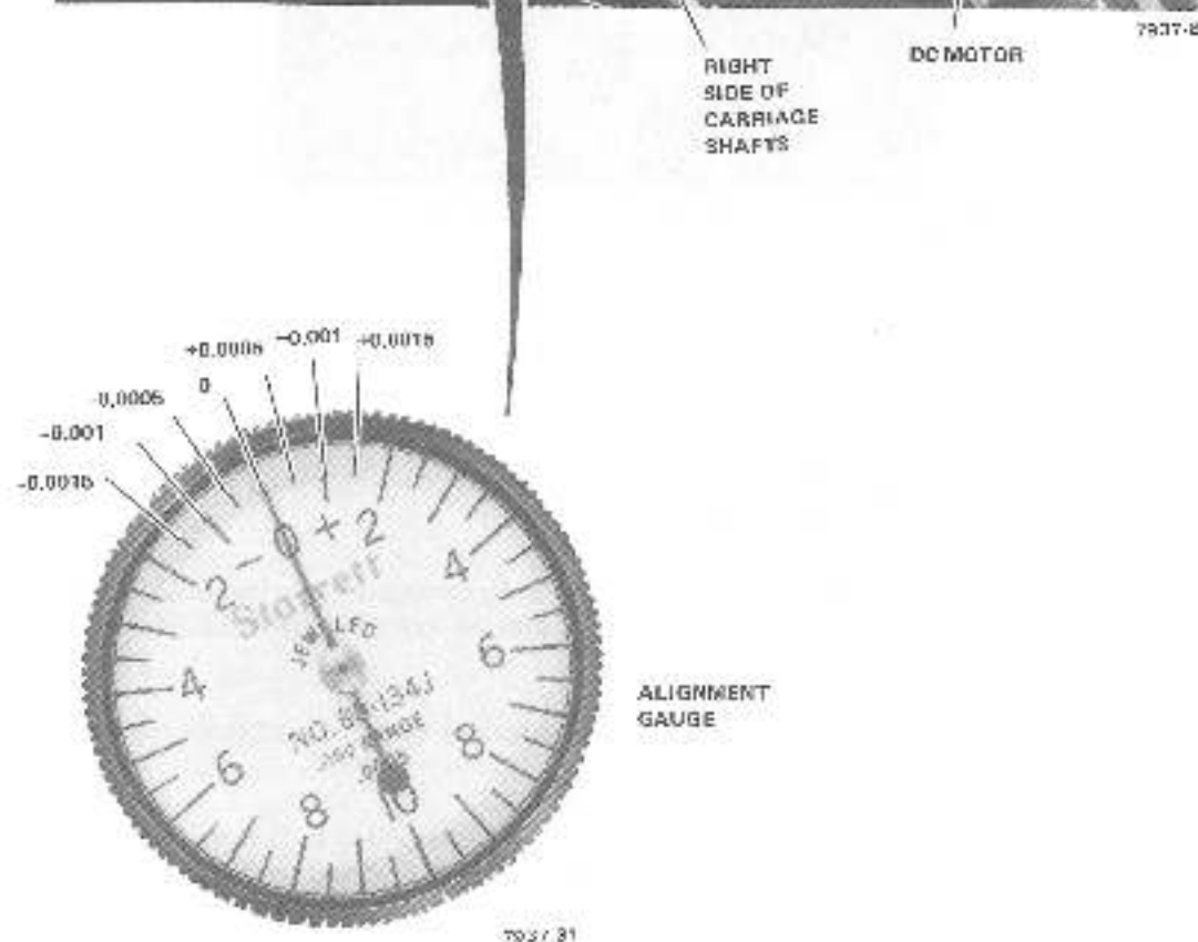
Figure 22 Alignment Gauge Positioning
