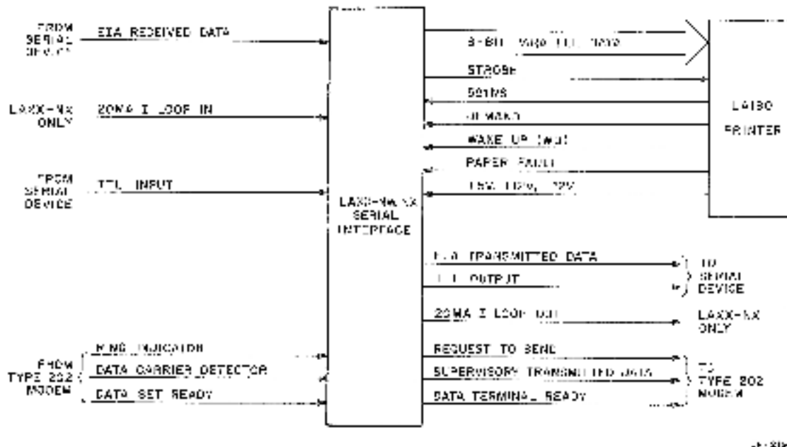
Figure 12 Serial Interface/LA180 Simplified Interface Diagram
