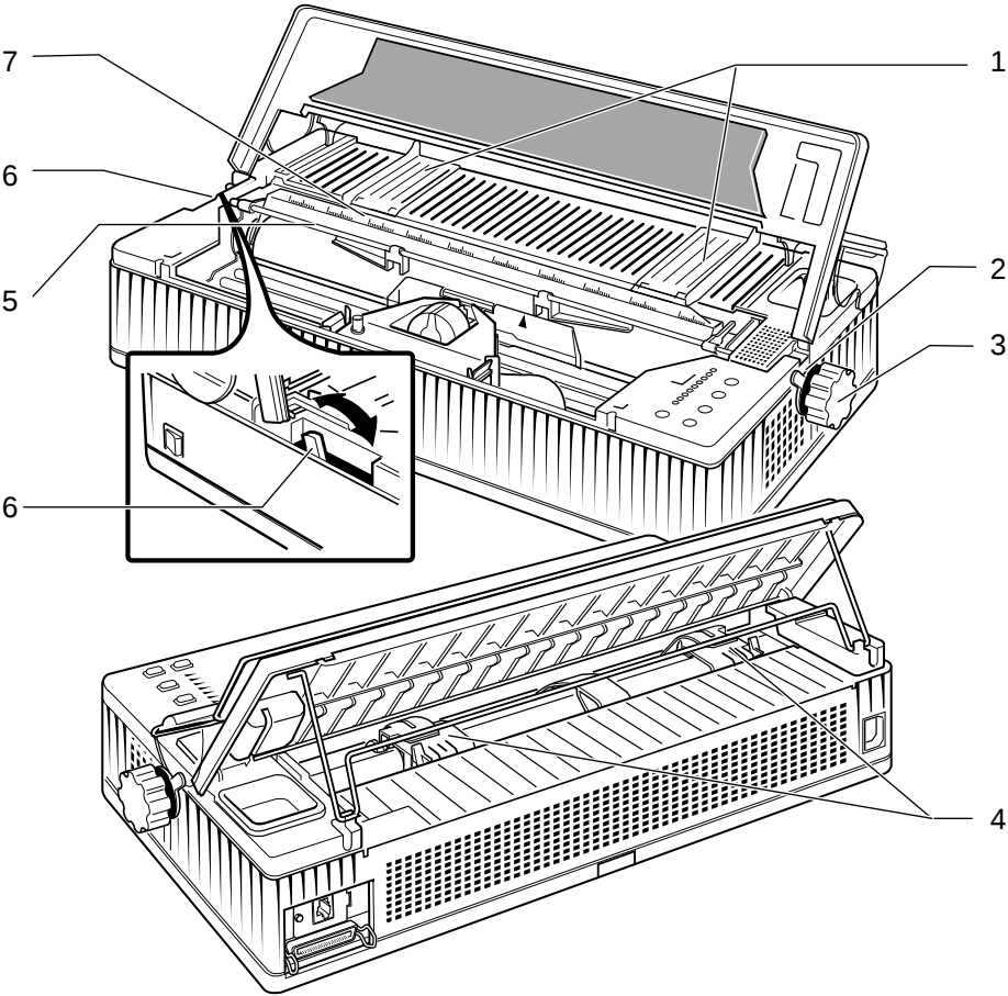
Figure 3-1 Paper Controls
