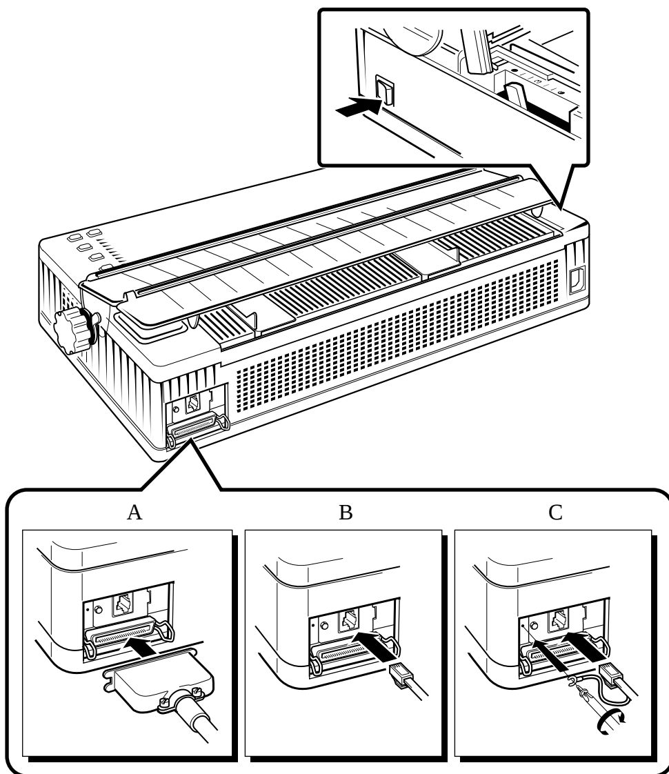
Figure 1-13 Interface Cable
