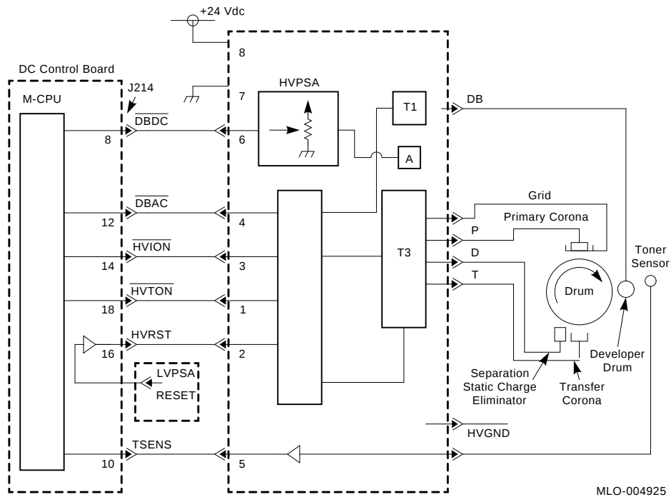
Figure 1–15: HVPSA Image Circuits
