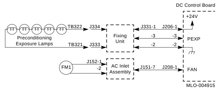
Figure 1-11: 2100 DC Control Board Output Signals (Part 2)
