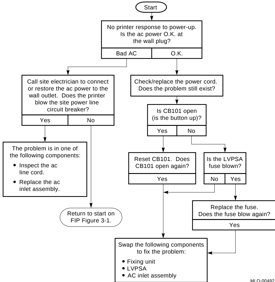
Figure 3-2: Power-Up Fault
