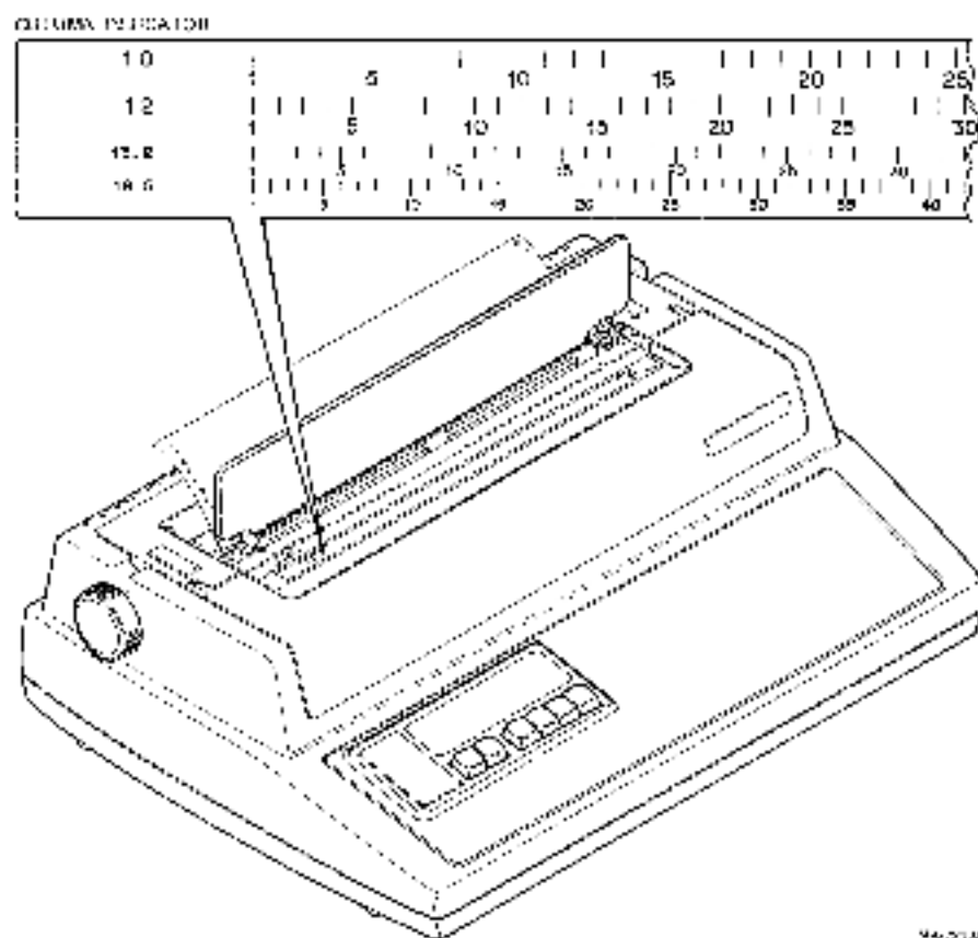
Figure 1-18 Column Indicator
