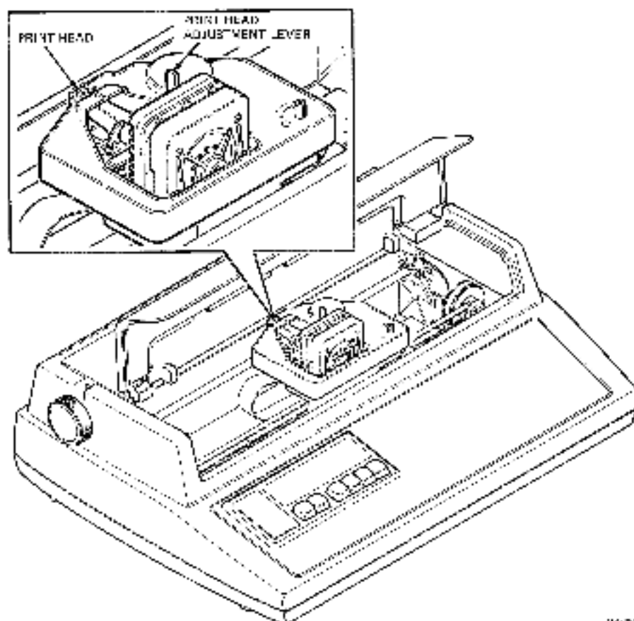
Figure 2-18 Printhead Adjustment
