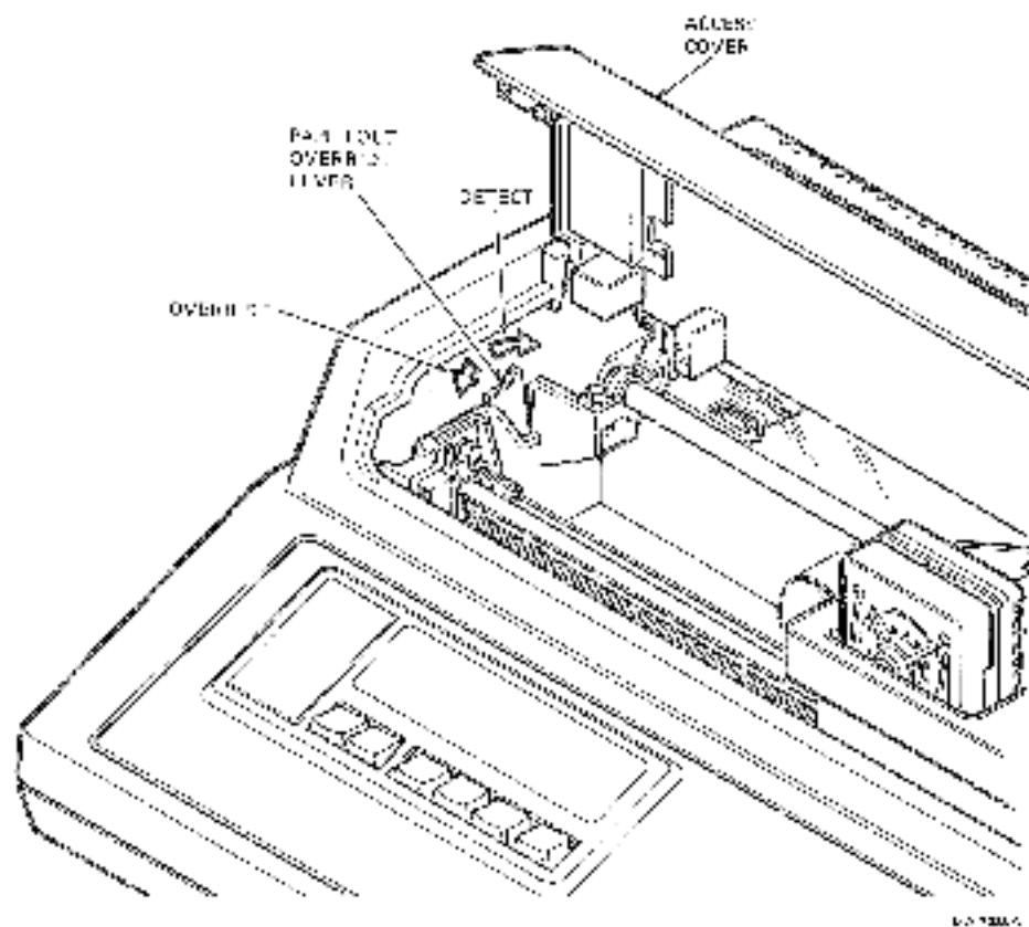
Figure 1-15 Paper Out Override Lever
