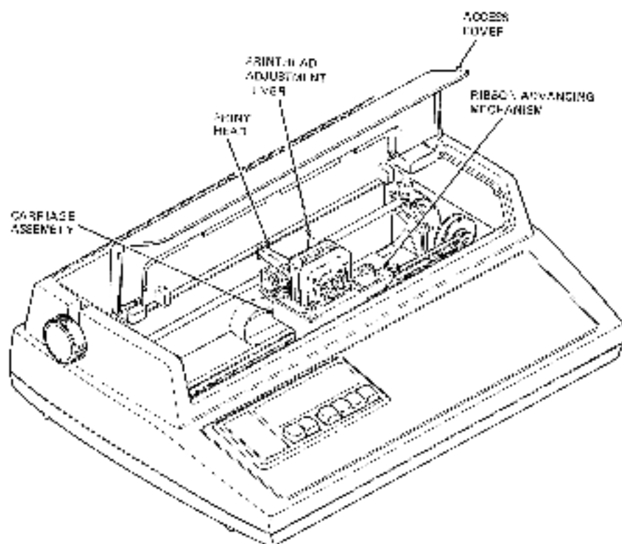
Figure 2-1 Carriage Assembly
