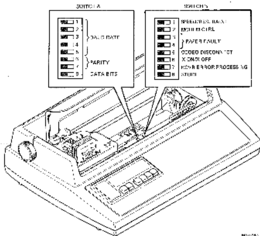
Figure 1-14 Communication Switches
