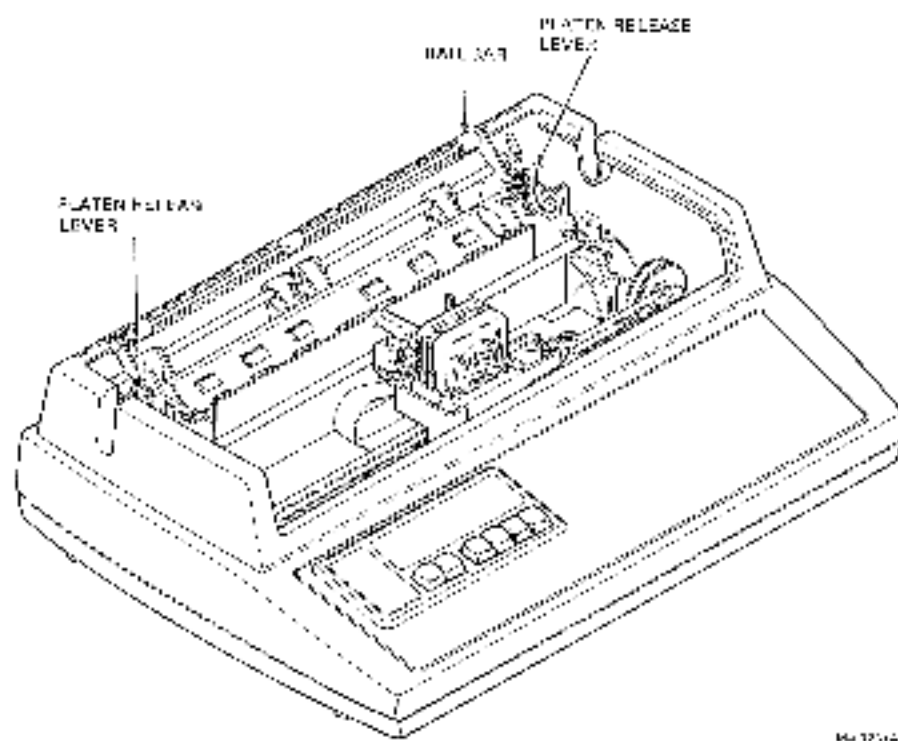
Figure 4-2 Platen Removal
