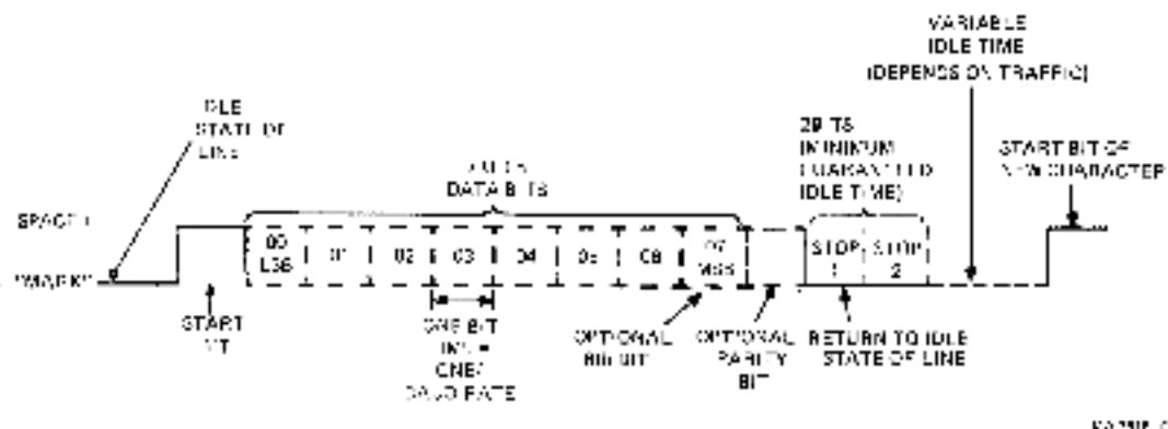
Figure 1-1 Serial Character Format in Terminal-to-Host Direction
