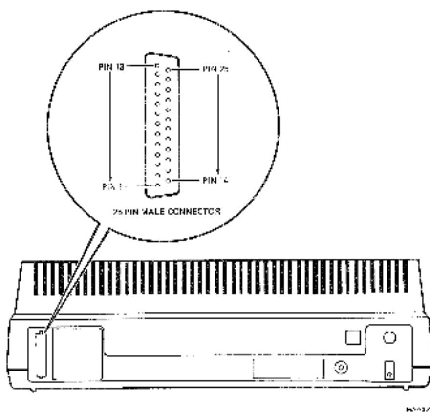
Figure 1-3 EIA Connector
