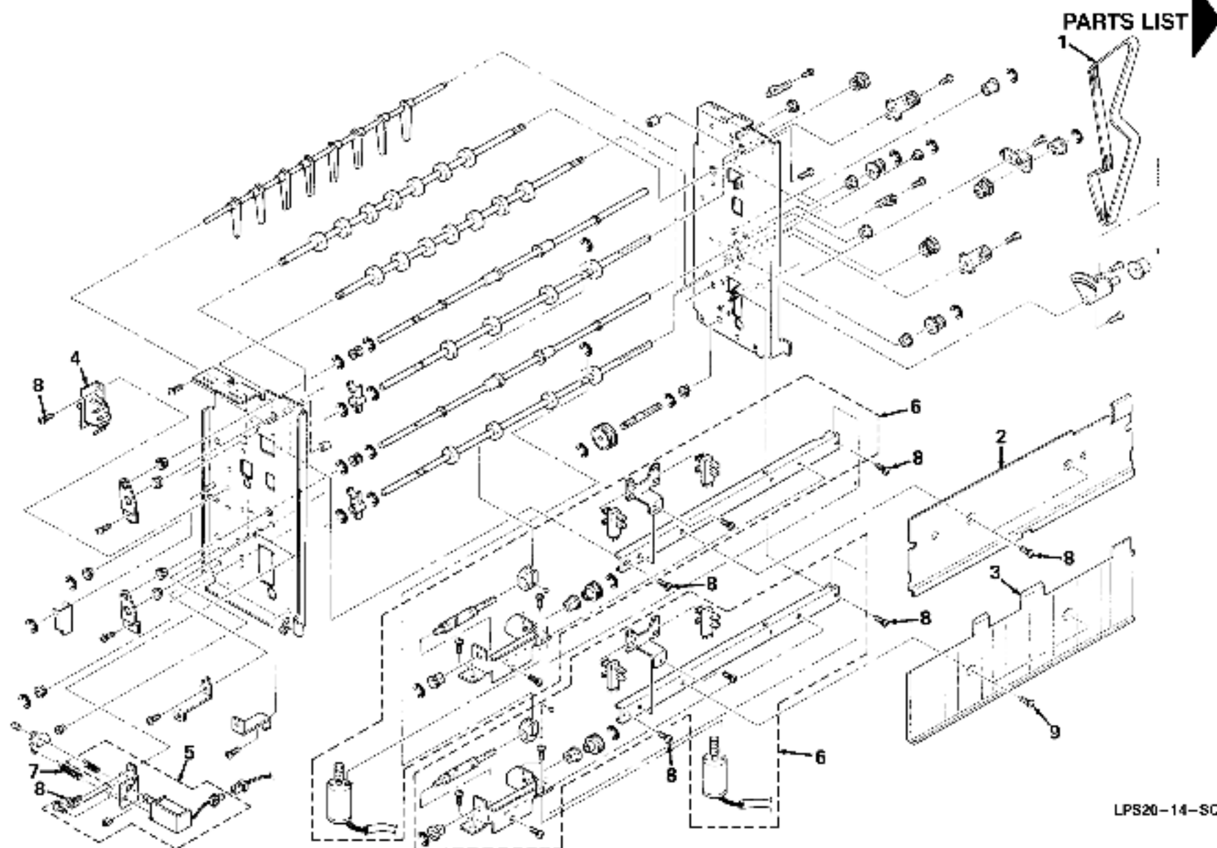
Figure 14. Tray Assembly, Large Capacity Output #2
