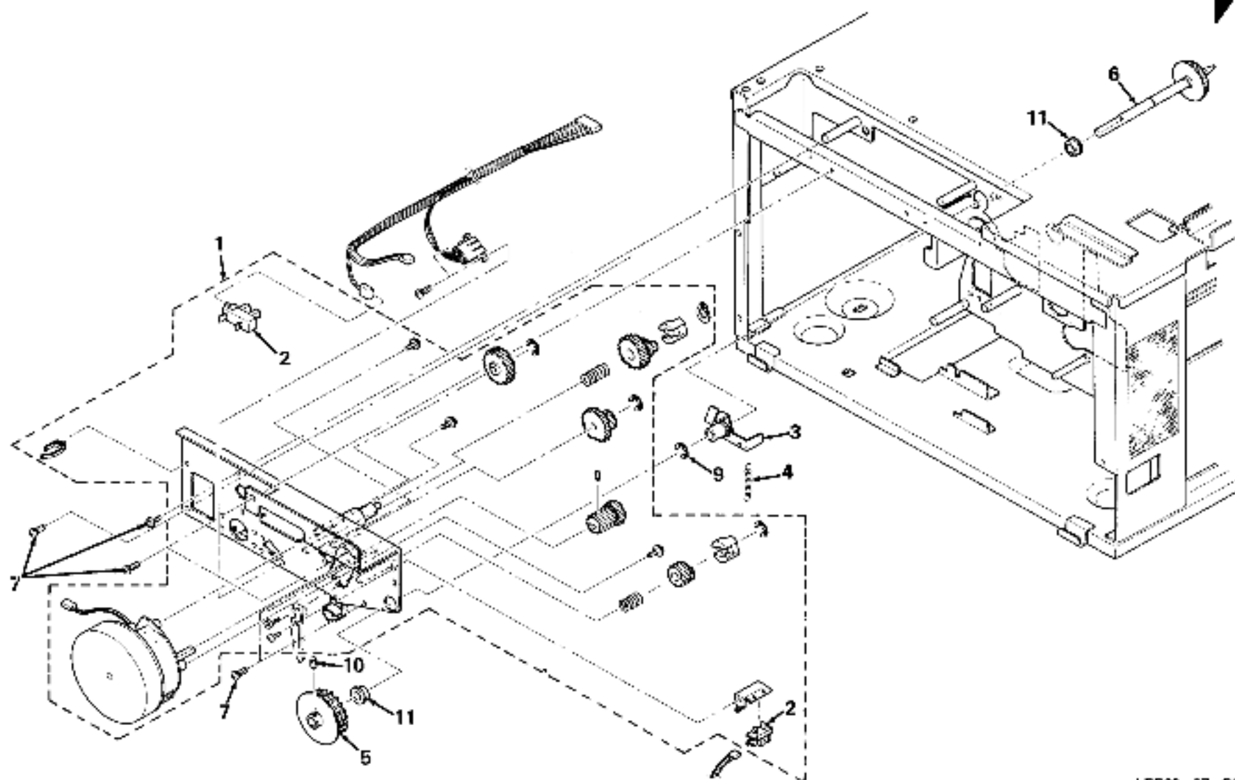
Figure 7. Drive Assembly, Development
