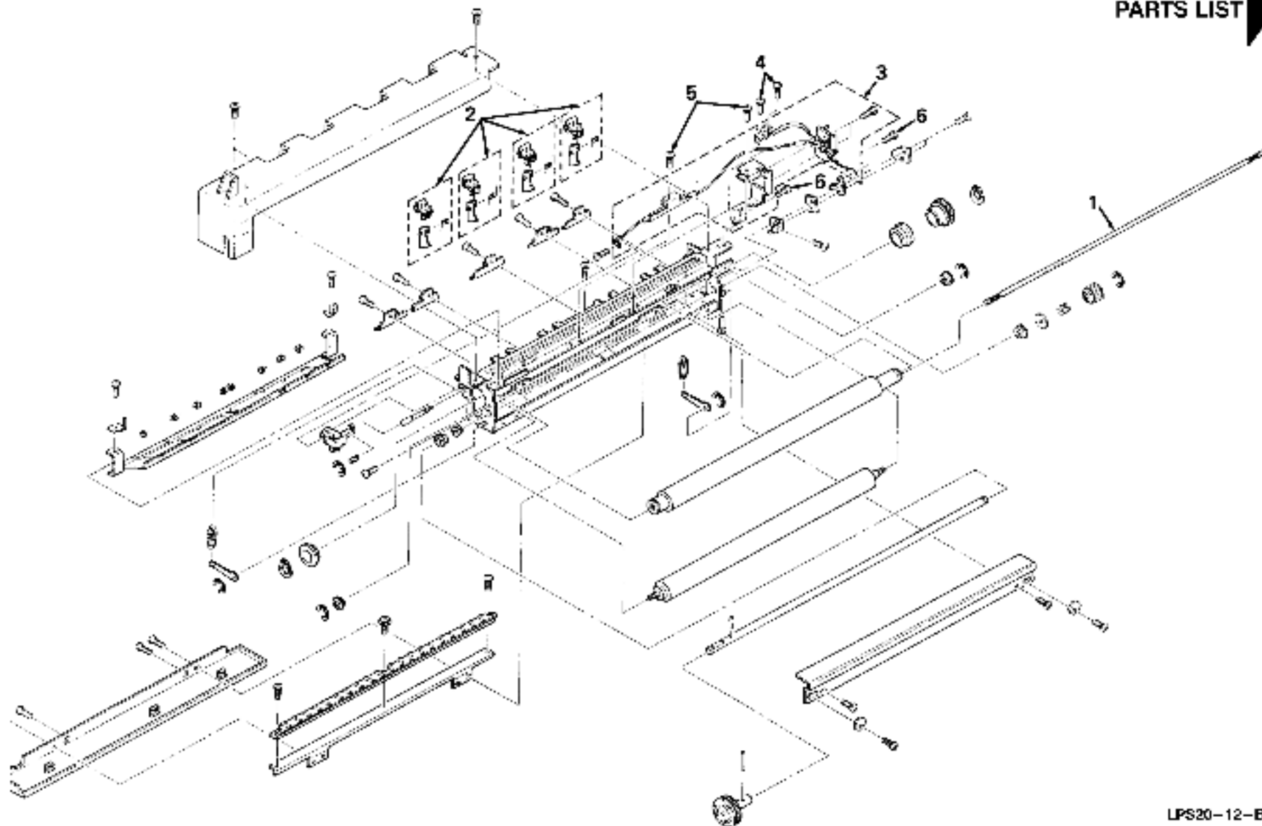
Figure 12. Fusing Assembly
