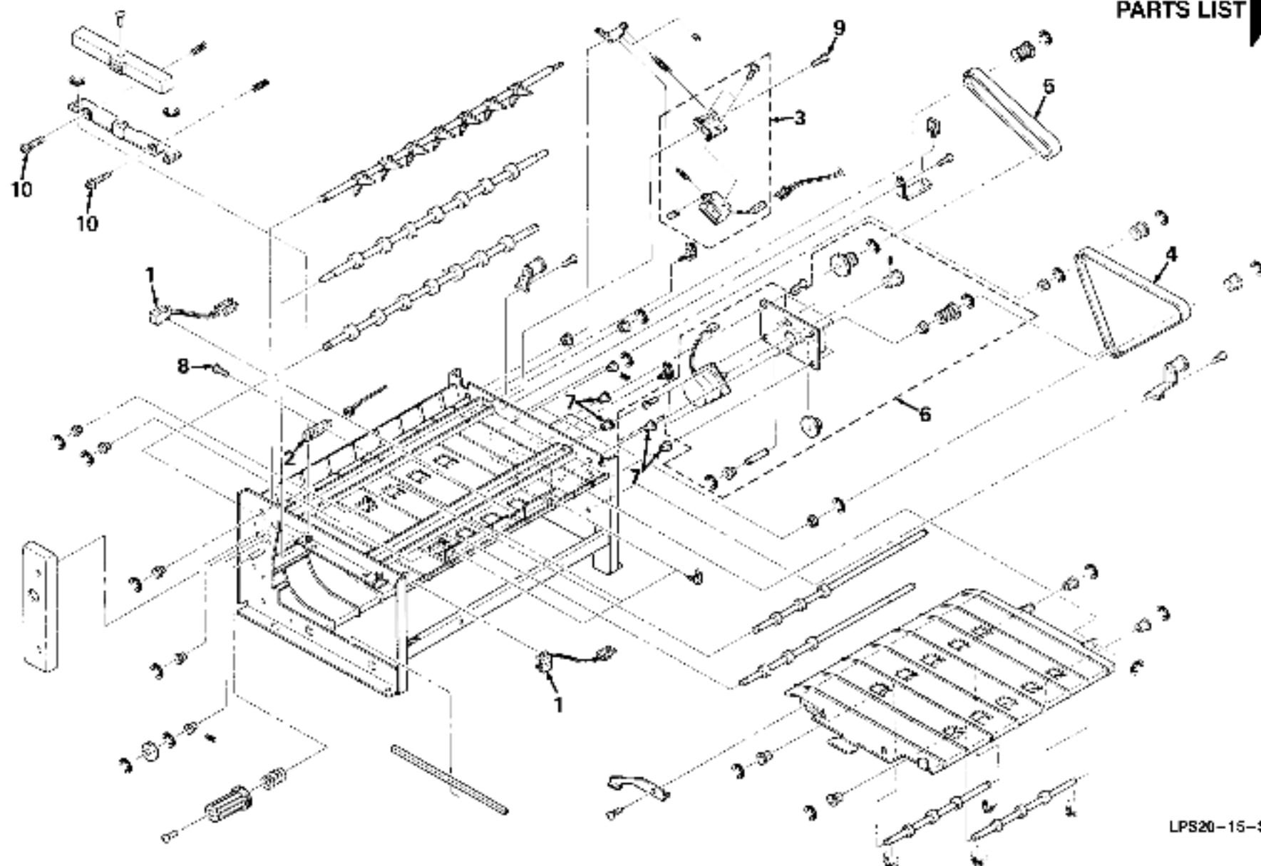
Figure 15. DPX Assembly
