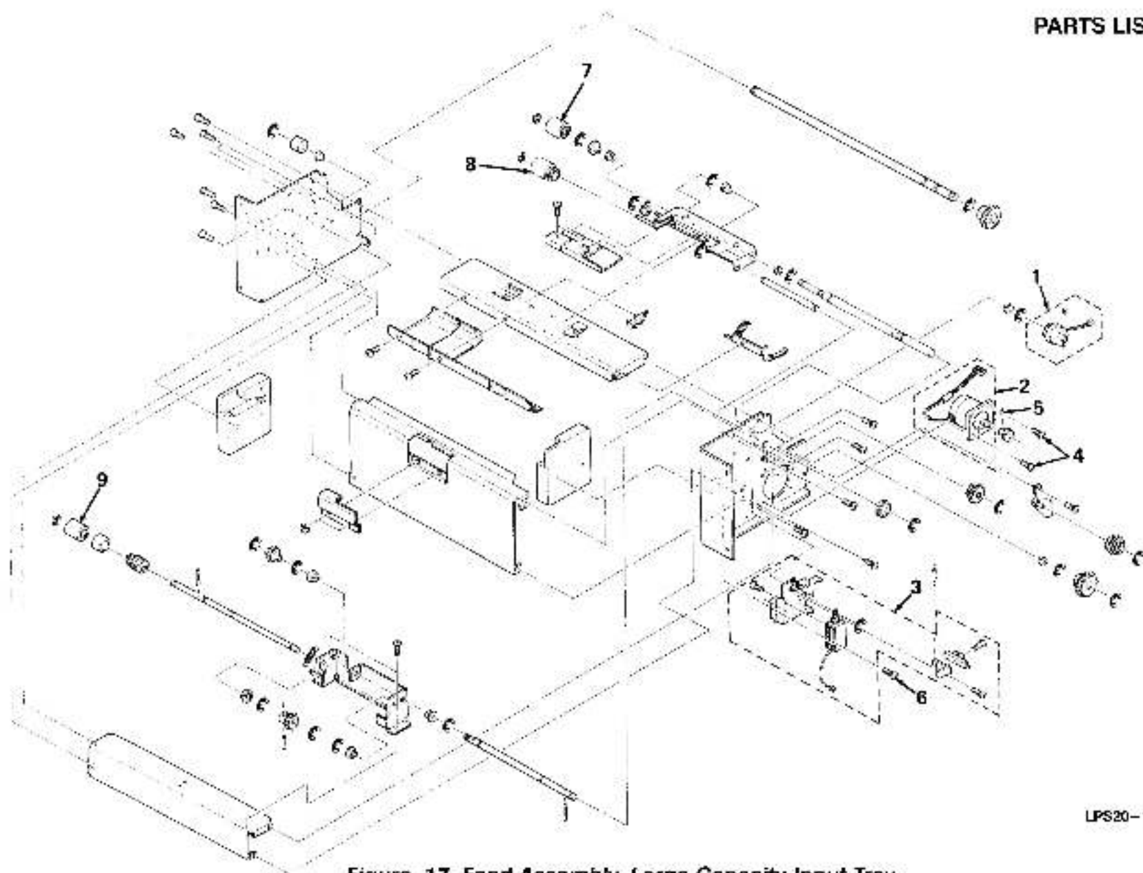
Figure 17. Feed Assembly, Large Capacity Input Tray
