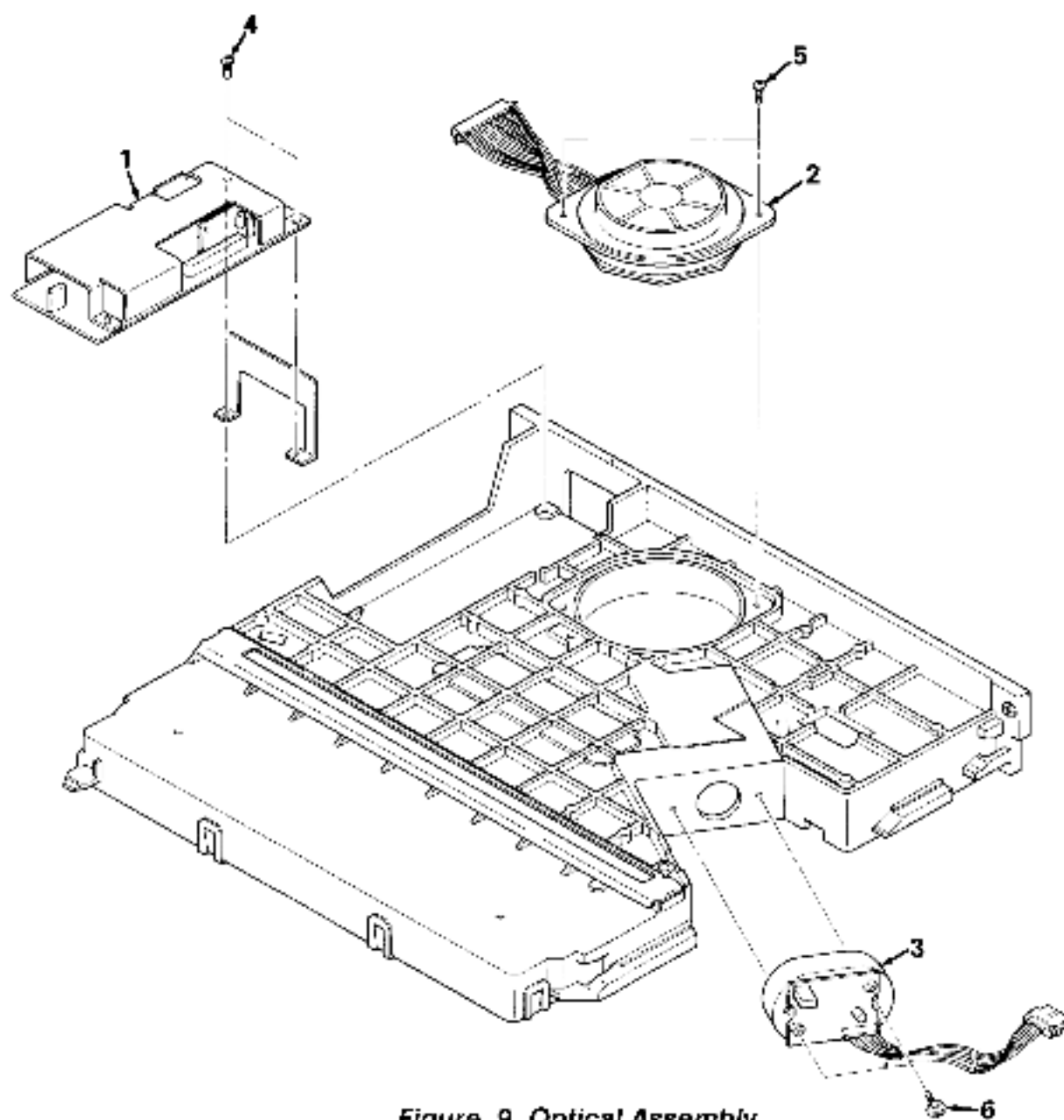
Figure 9. Optical Assembly
