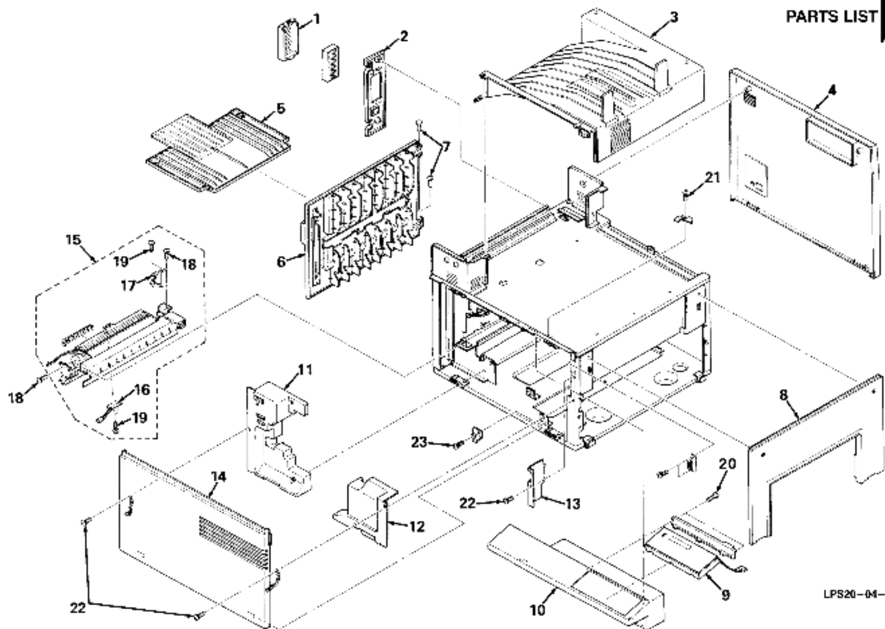
Figure 4. Exterior Assembly
