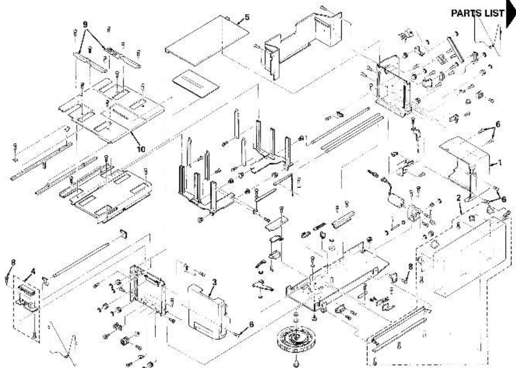
Figure 16. Tray Assembly, Large Capacity Input
