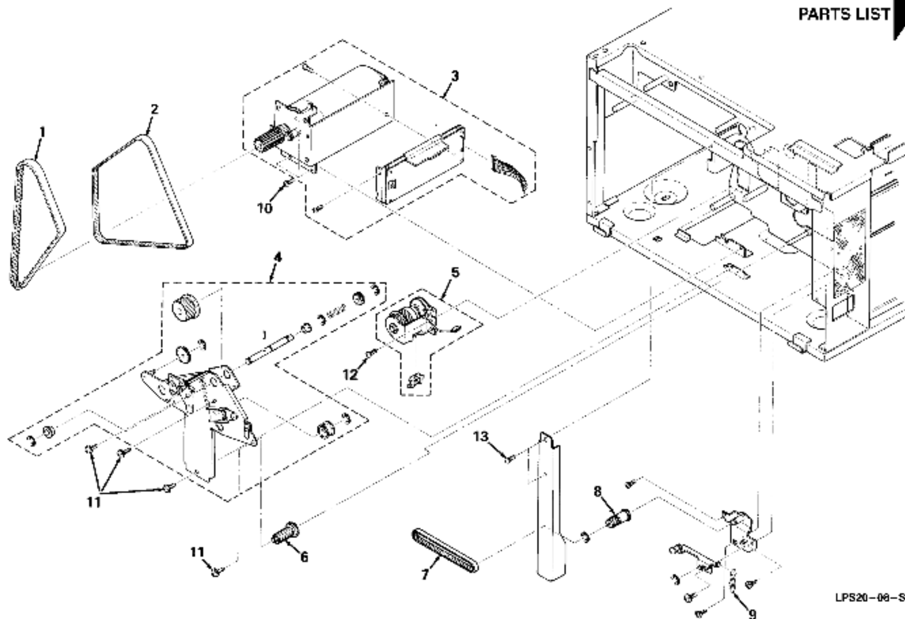
Figure 8. Drive Assembly, Main
