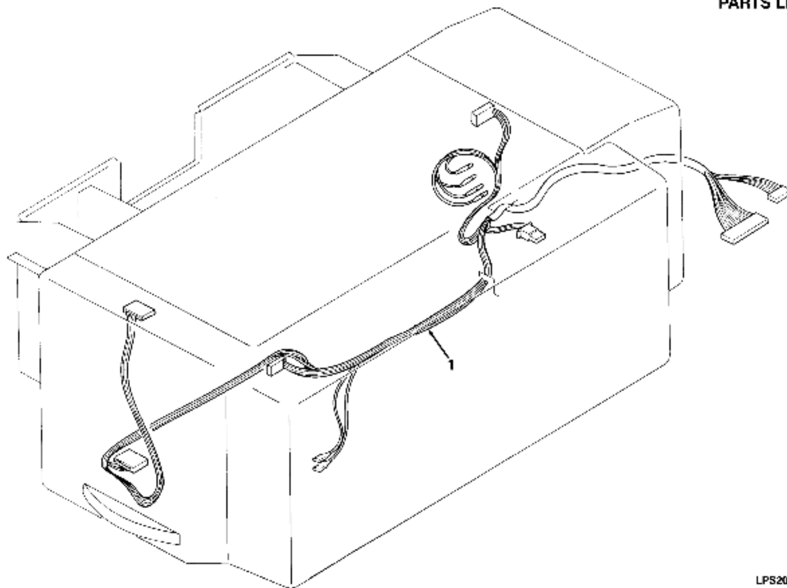
Figure 21. Harness Assembly, Large Capacity Input Tray
