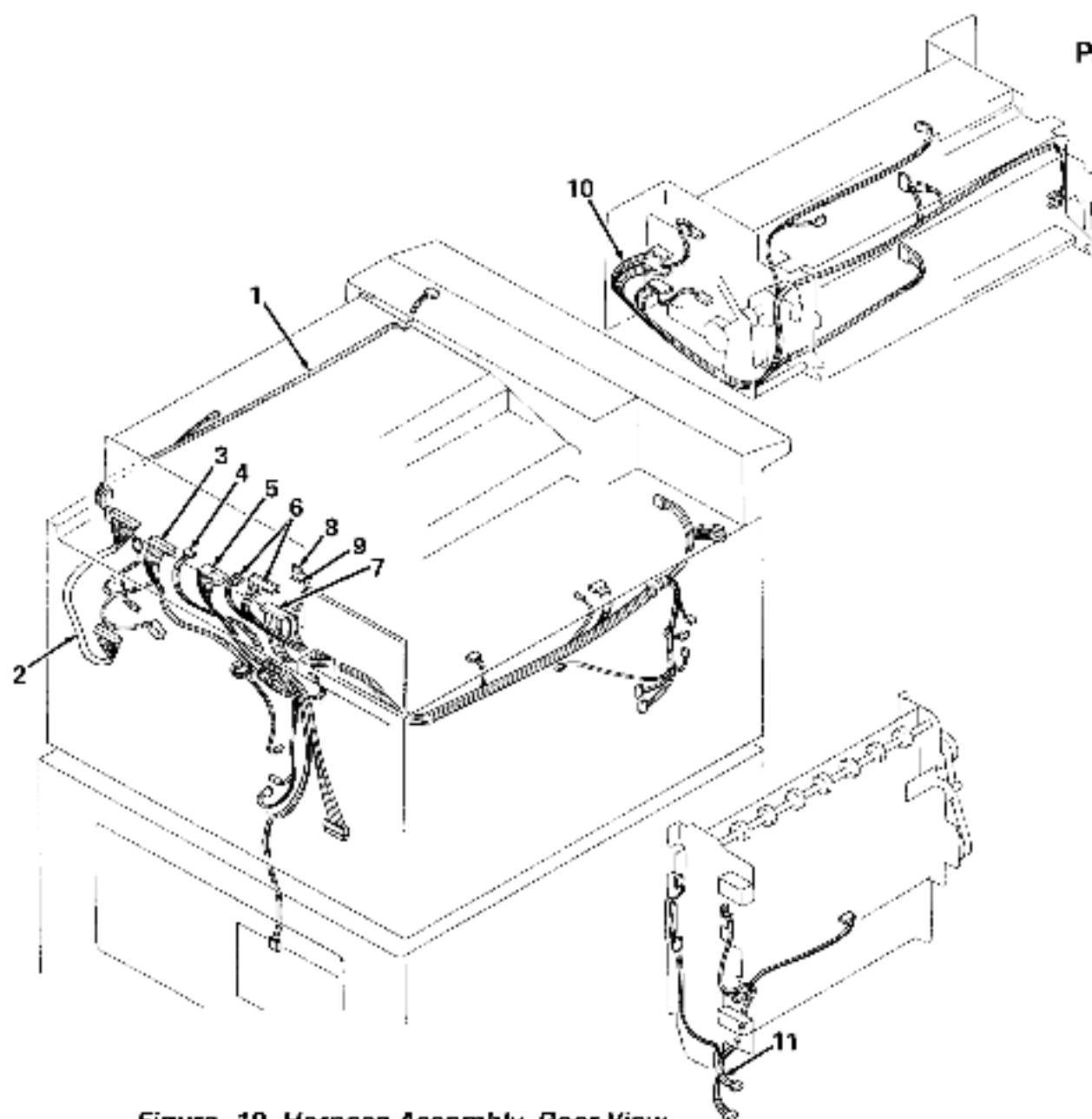
Figure 19. Harness Assembly, Rear View
