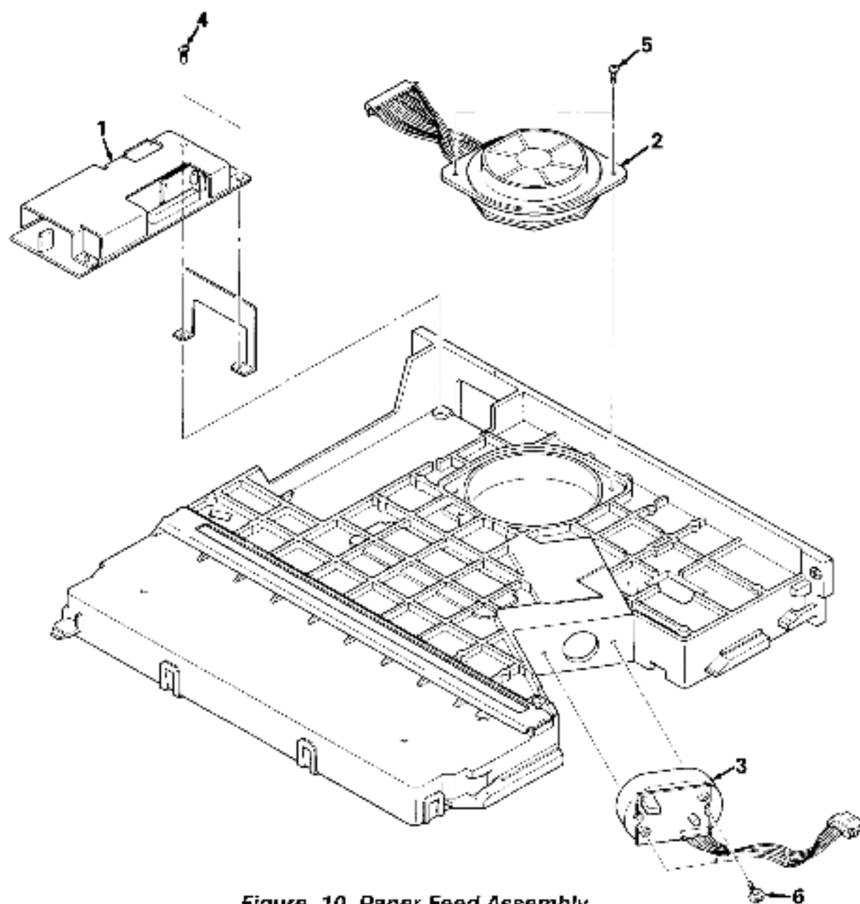
Figure 10. Paper Feed Assembly
