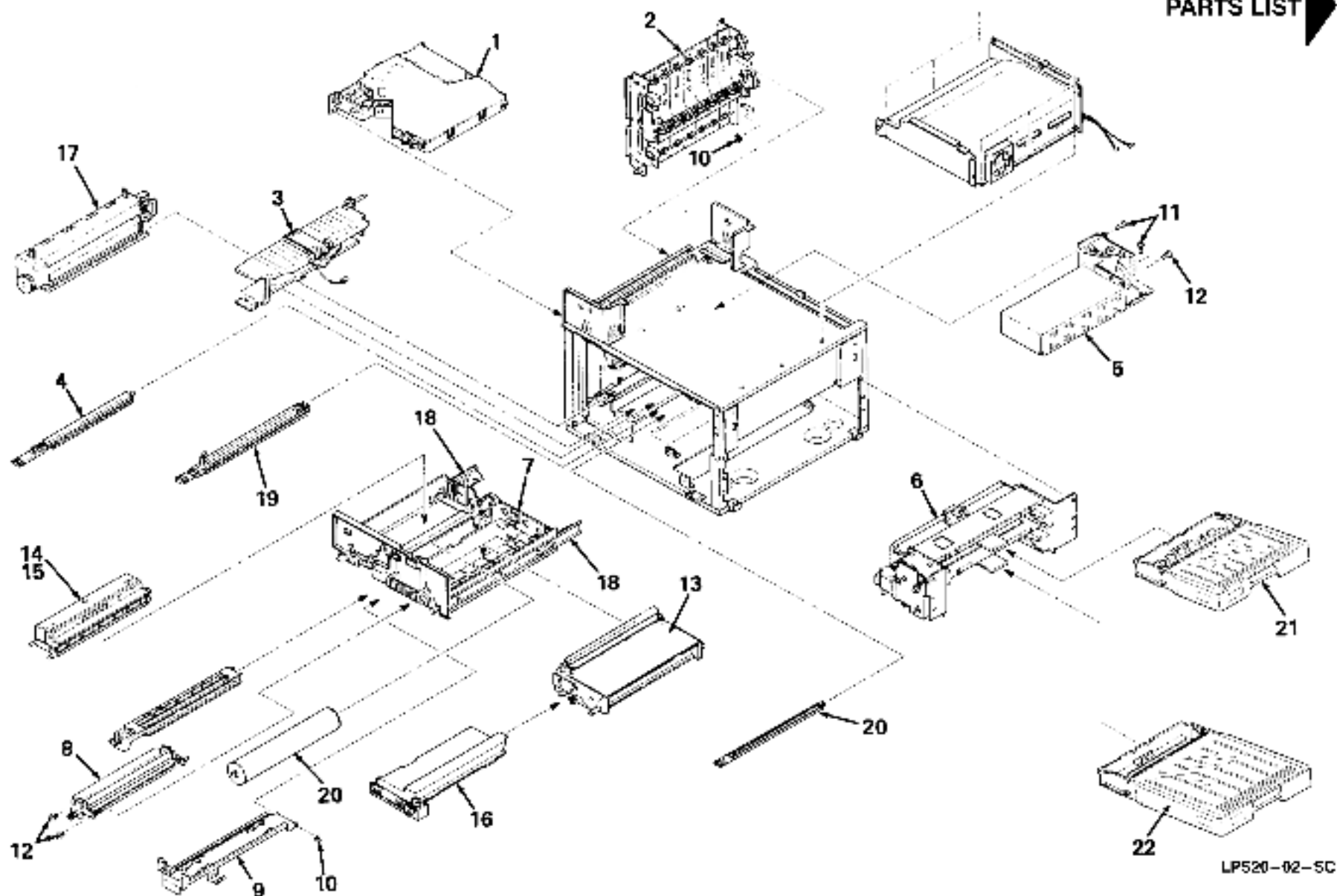
Figure 2. Component Assembly
