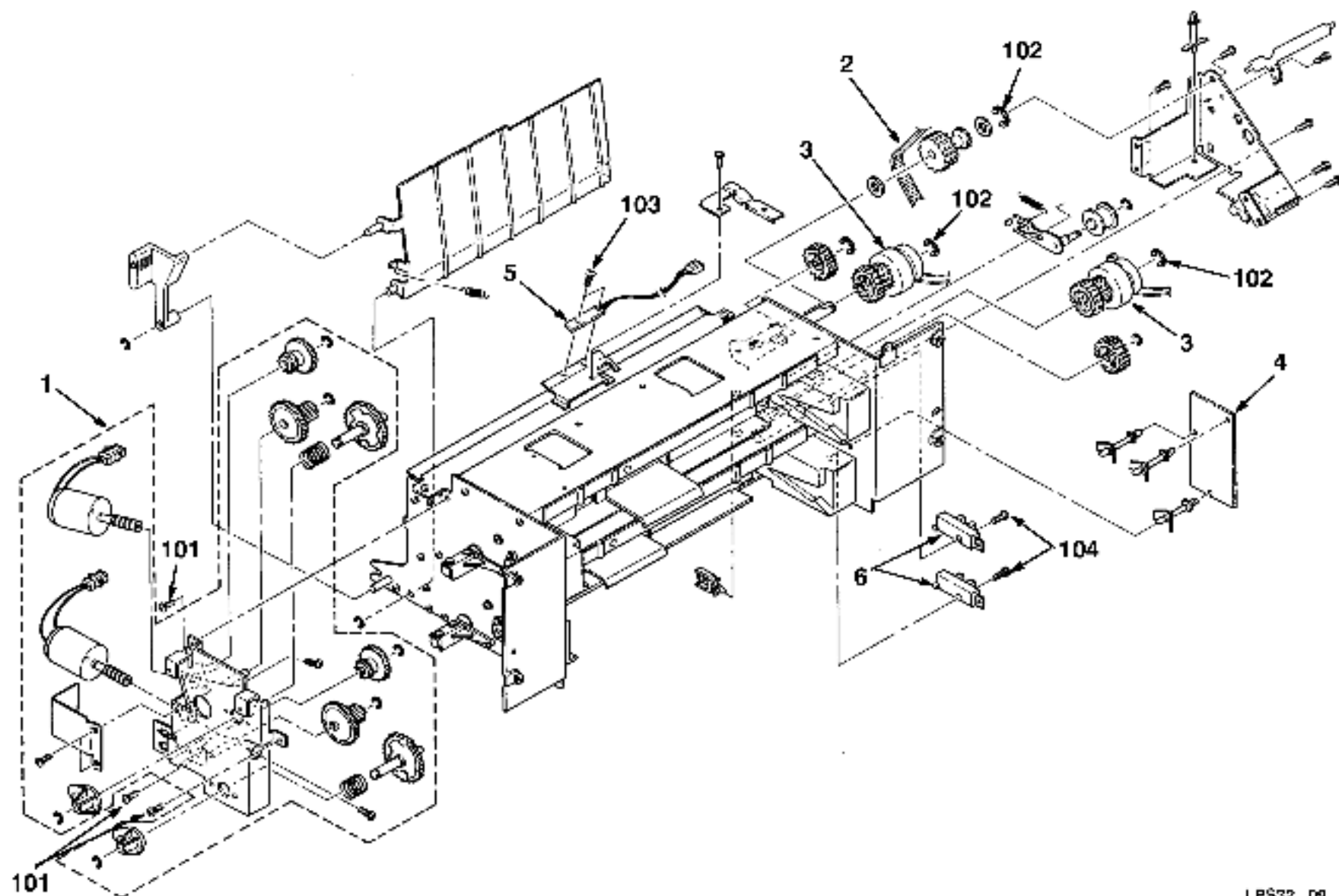
Figure 9. Feed Assembly, Paper (Cassette)
