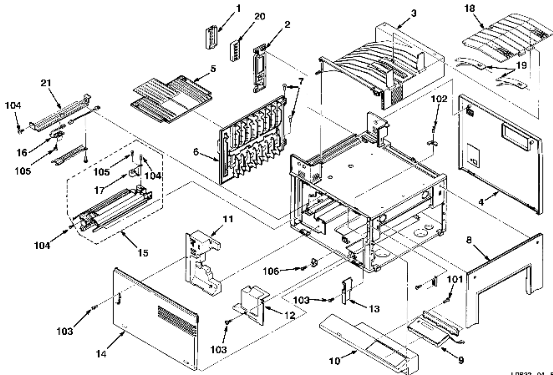
Figure 4. Exterior, LPS32
