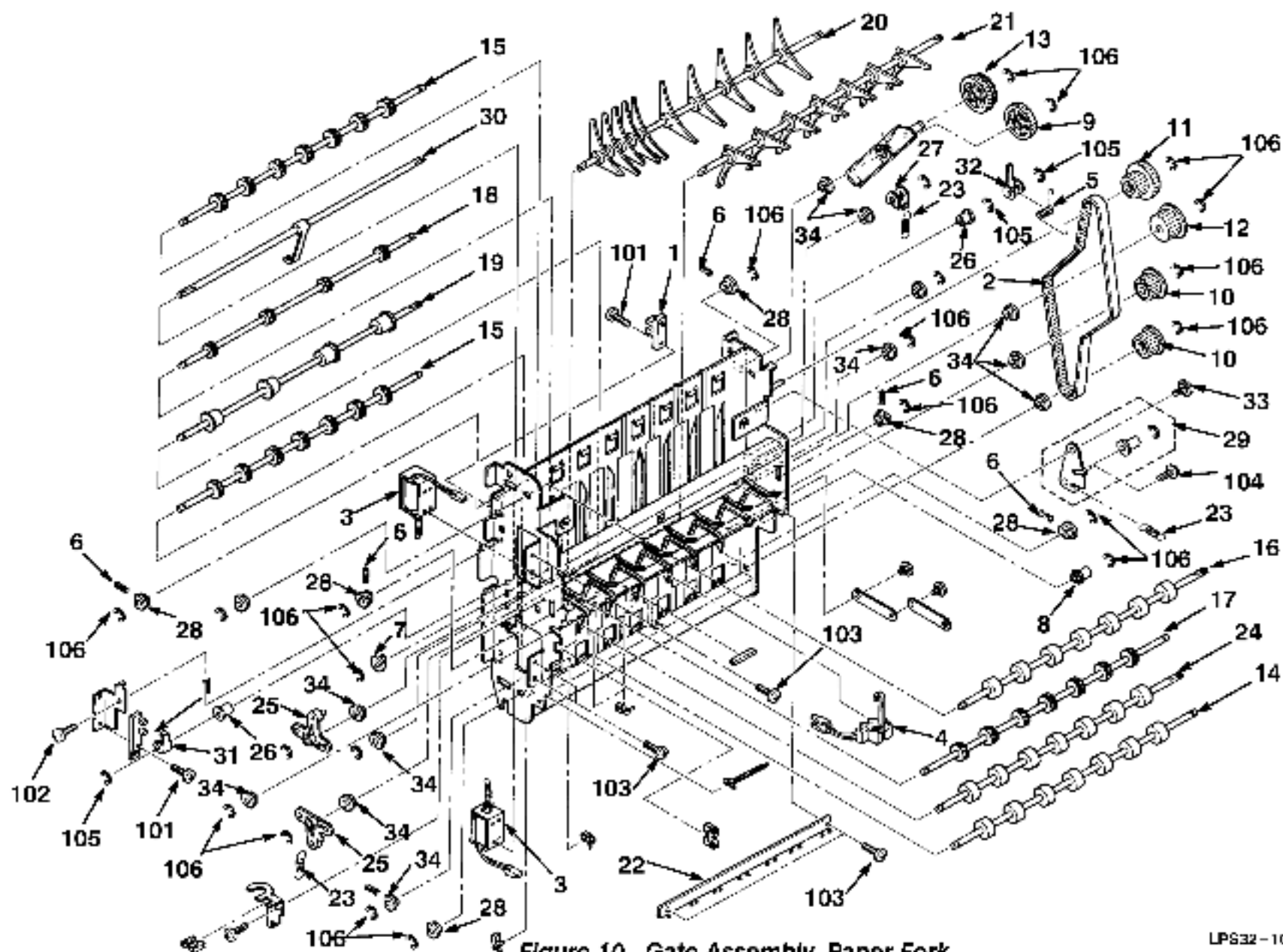
Figure 10. Gate Assembly, Paper Fork
