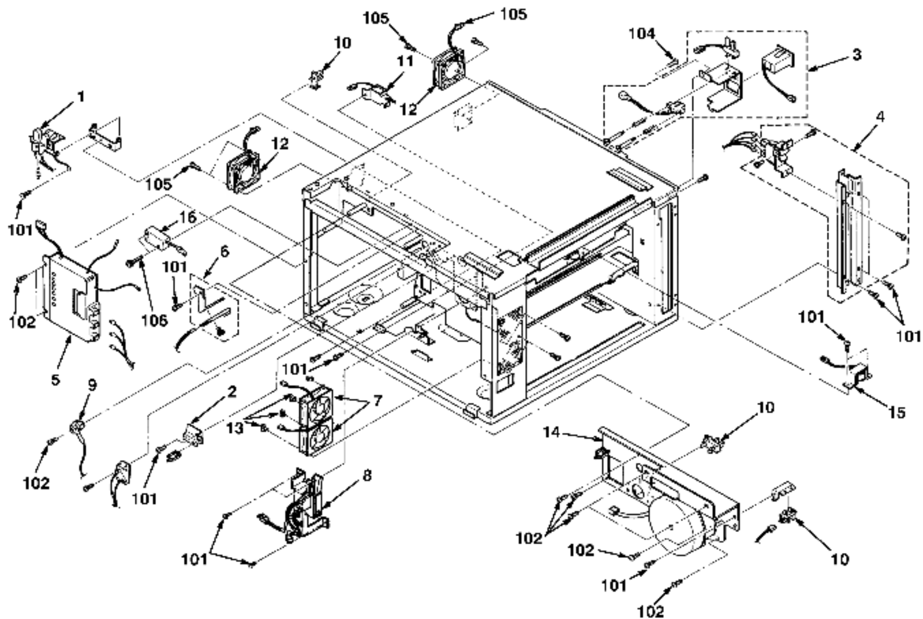
Figure 6. Electrical Assembly
