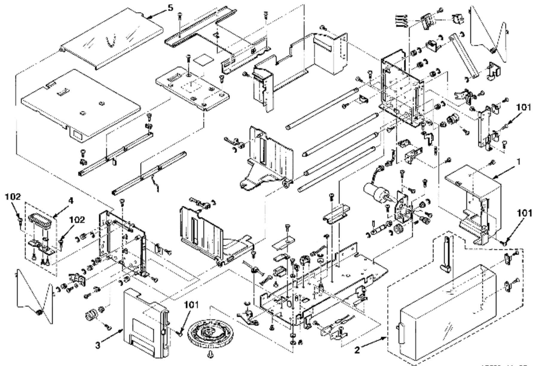
Figure 14. LCIT (Large Capacity Input Tray)
