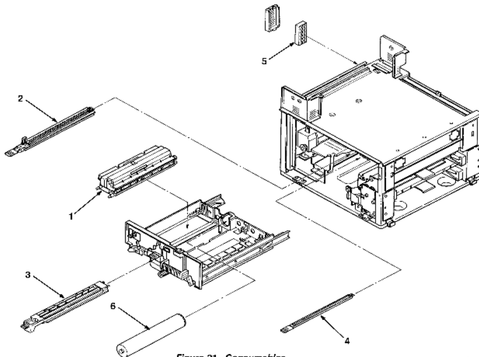
Figure 21. Consumables
