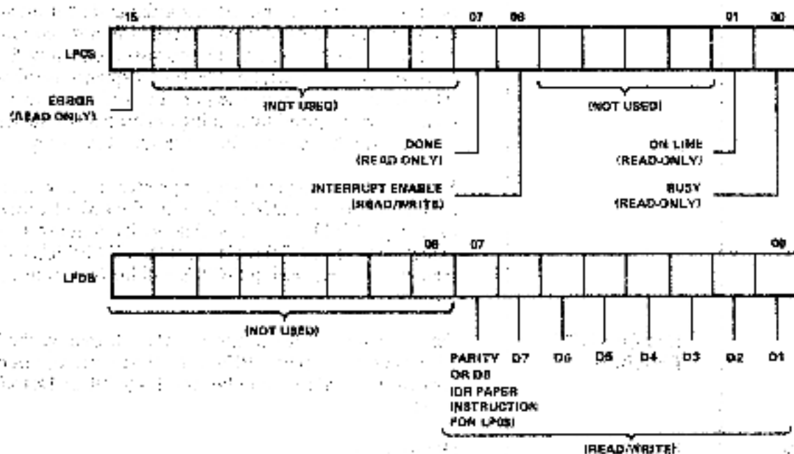
Figure 3-1 LPV11 Word Formats
