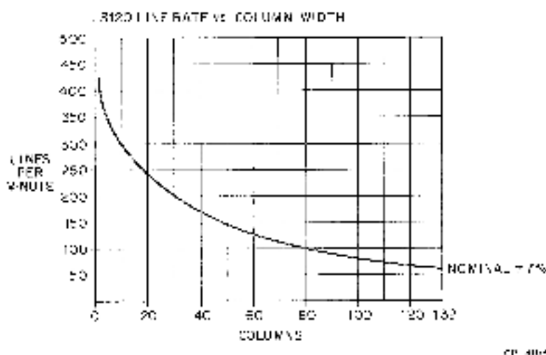
Figure 4-2 LS120 Line Rate Versus Column Width
