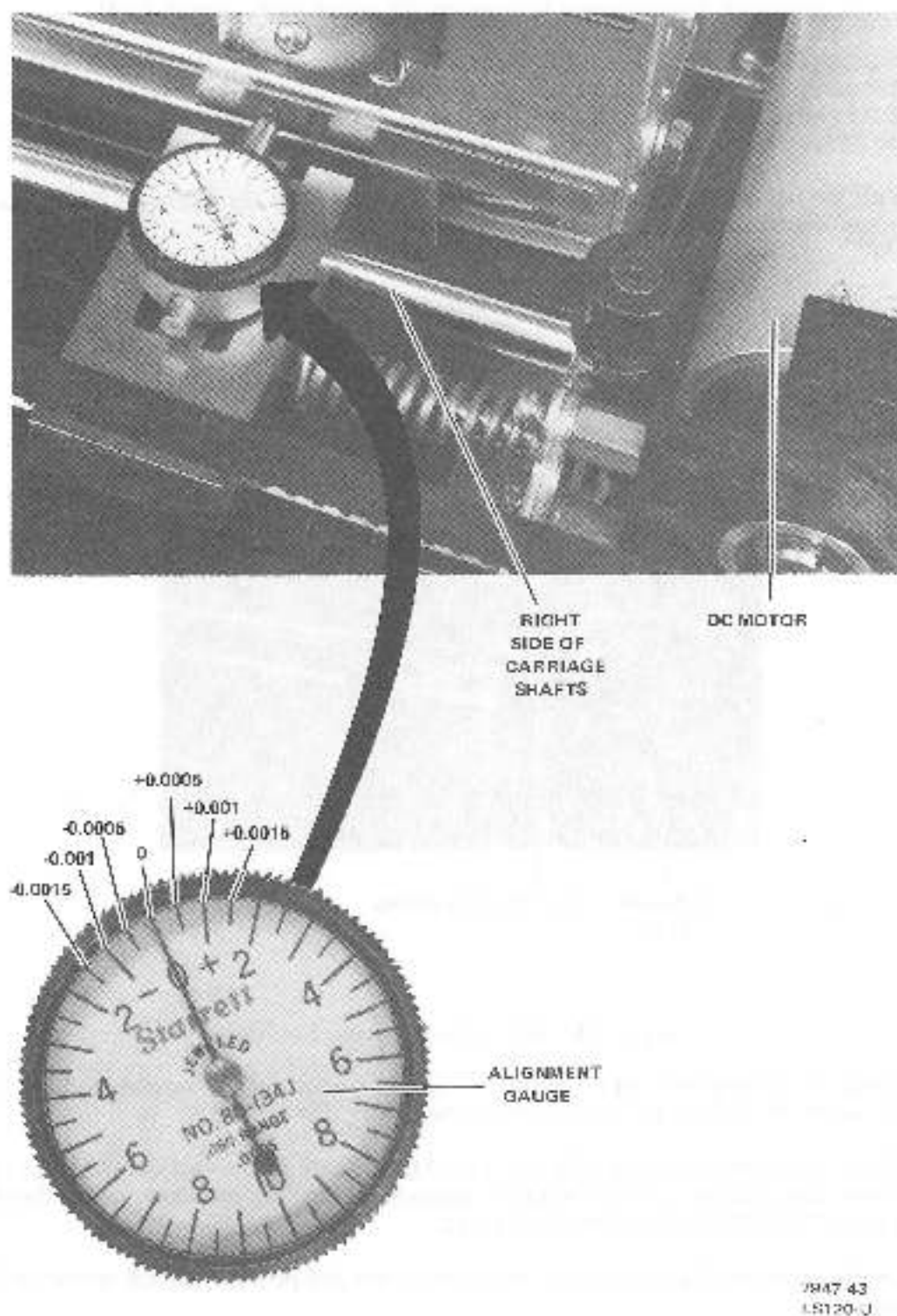
Figure 7-14 Alignment Gauge Positioning
