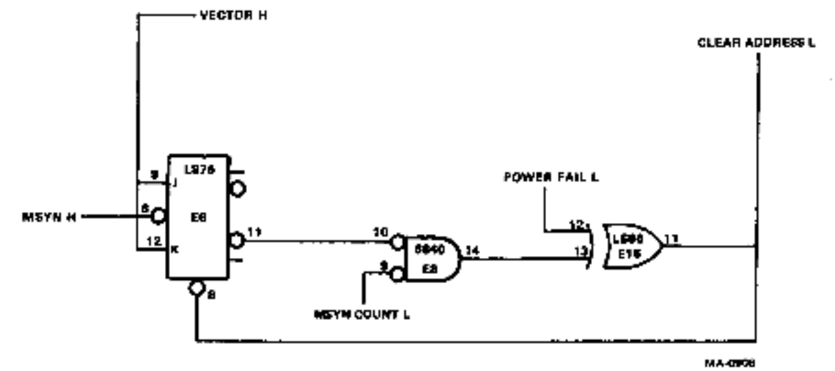
Figure 2-8 Power-Up Transfer Detection Logic
