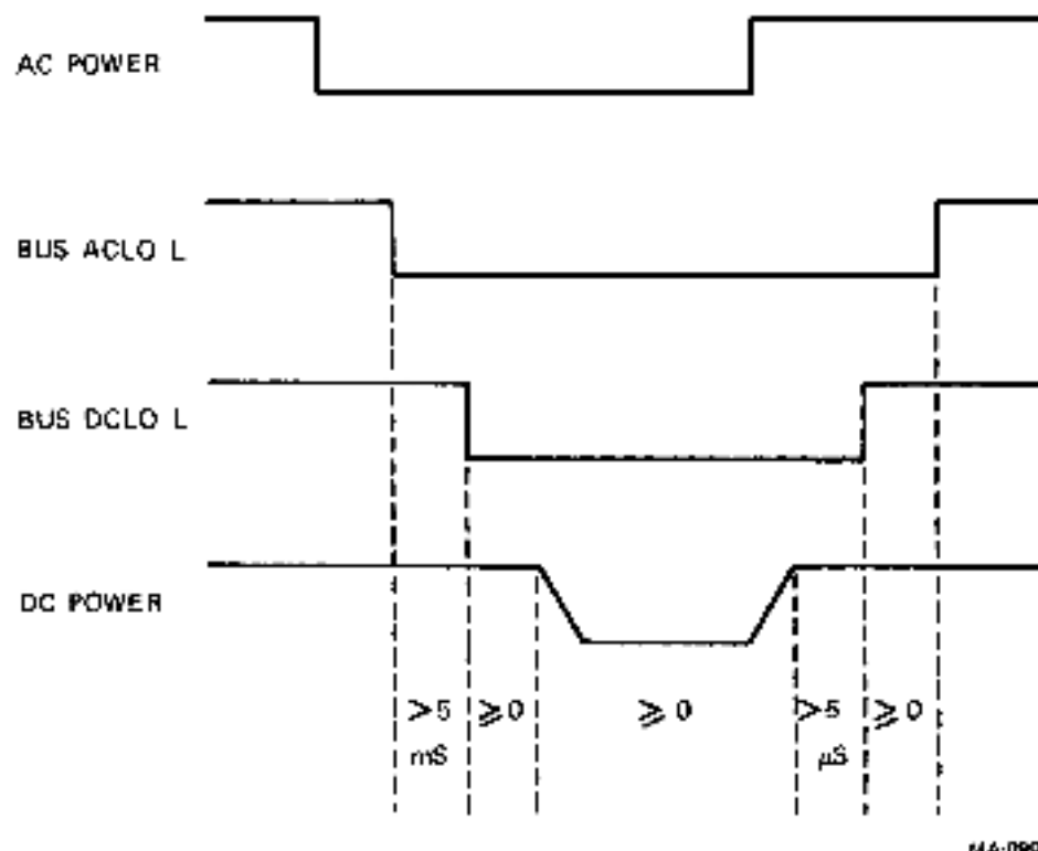
Figure 2-3 Power-Down/Power-Up Sequence
