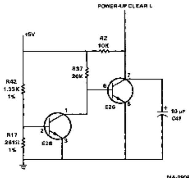
Figure 2-9 Power-Up Clear Circuitry
