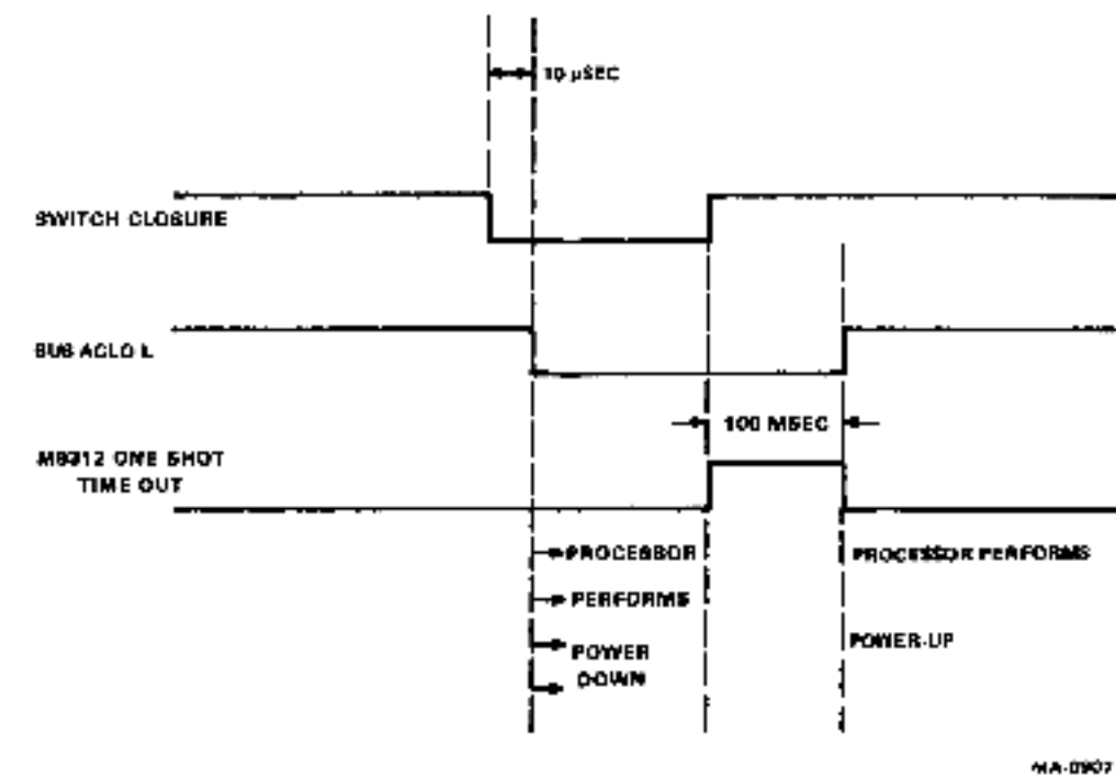
Figure 2-7 External Boot Timing
