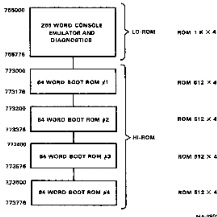
Figure 2-1 ROM Segregation
