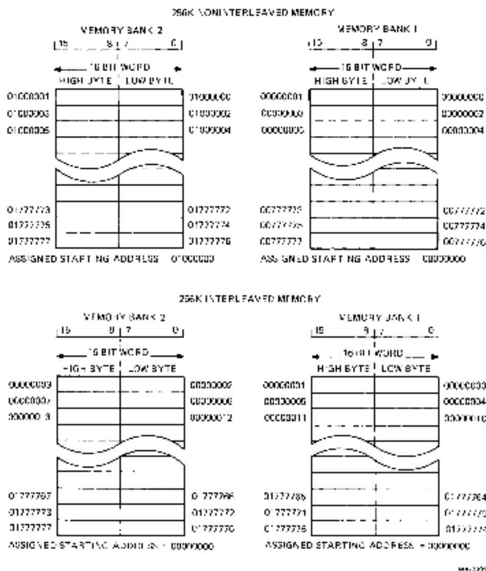
Figure 2-2 Interleaved Versus Noninterleaved Memory Organization of Two 128K Memory Banks
