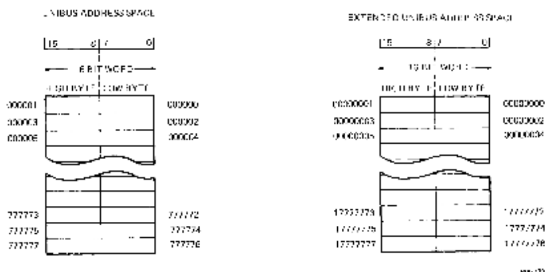
Figure 2-2 Bus Accessible Data Locations
