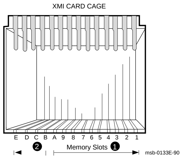
Figure 1–2: MS65A Configuration
