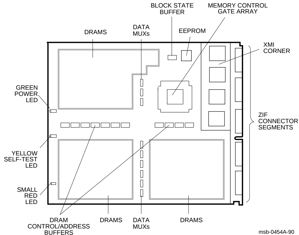
Figure 1-1: MS65A Module
