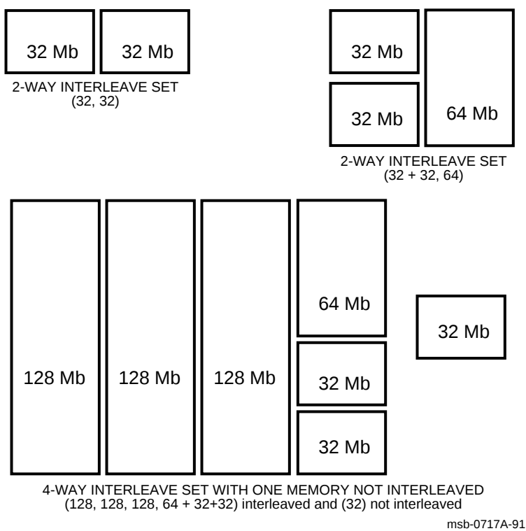
Figure B-1: MS65A Interleaving
