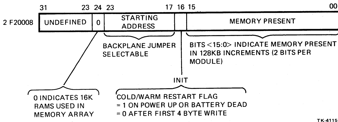
Figure 3-22 CSR2 Bit Allocations
