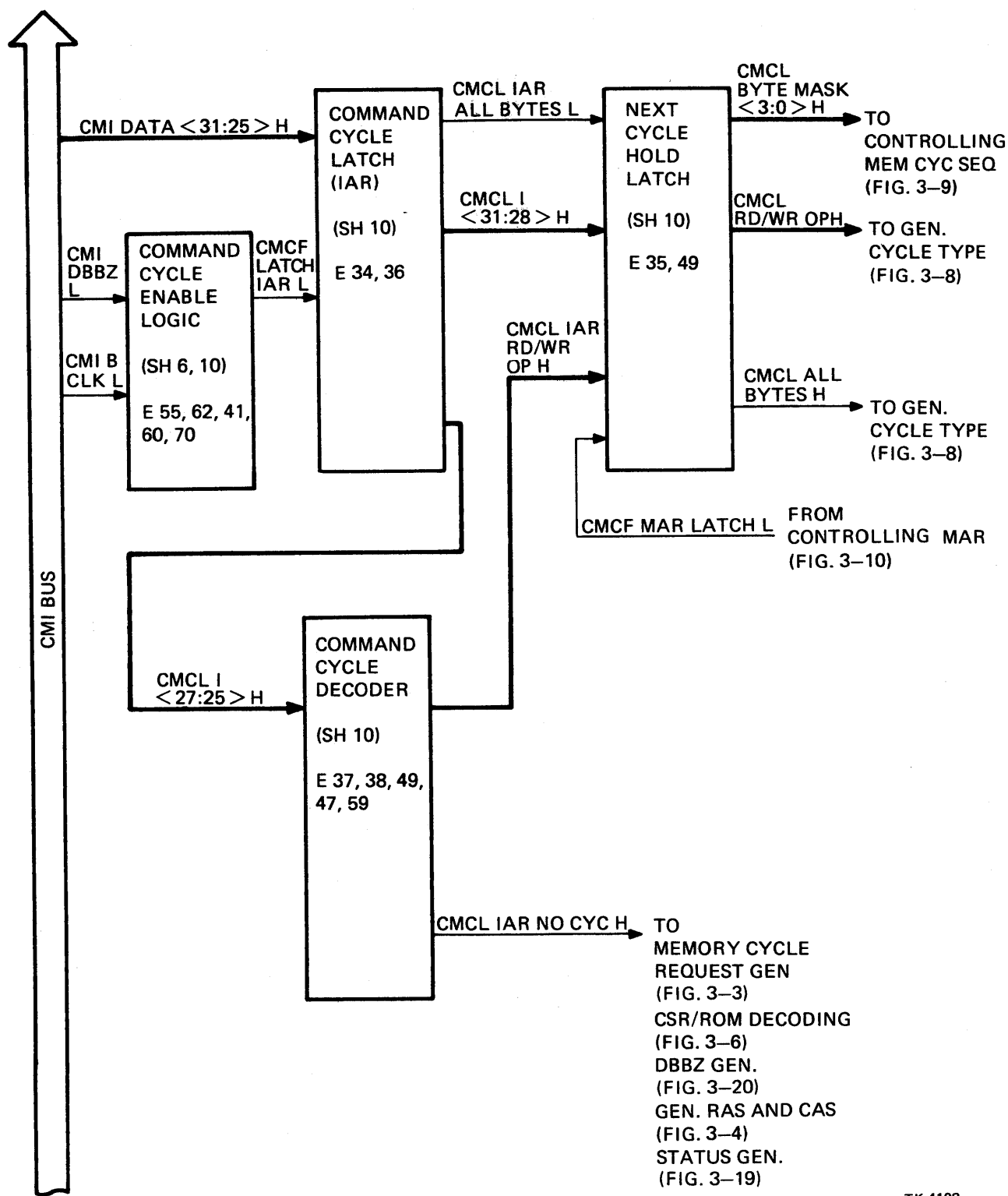
Figure 3-5 Intermediate Address Register Decoding
