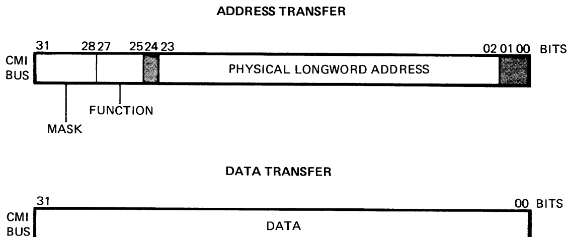
Figure 2-2 Address/Data Formats
