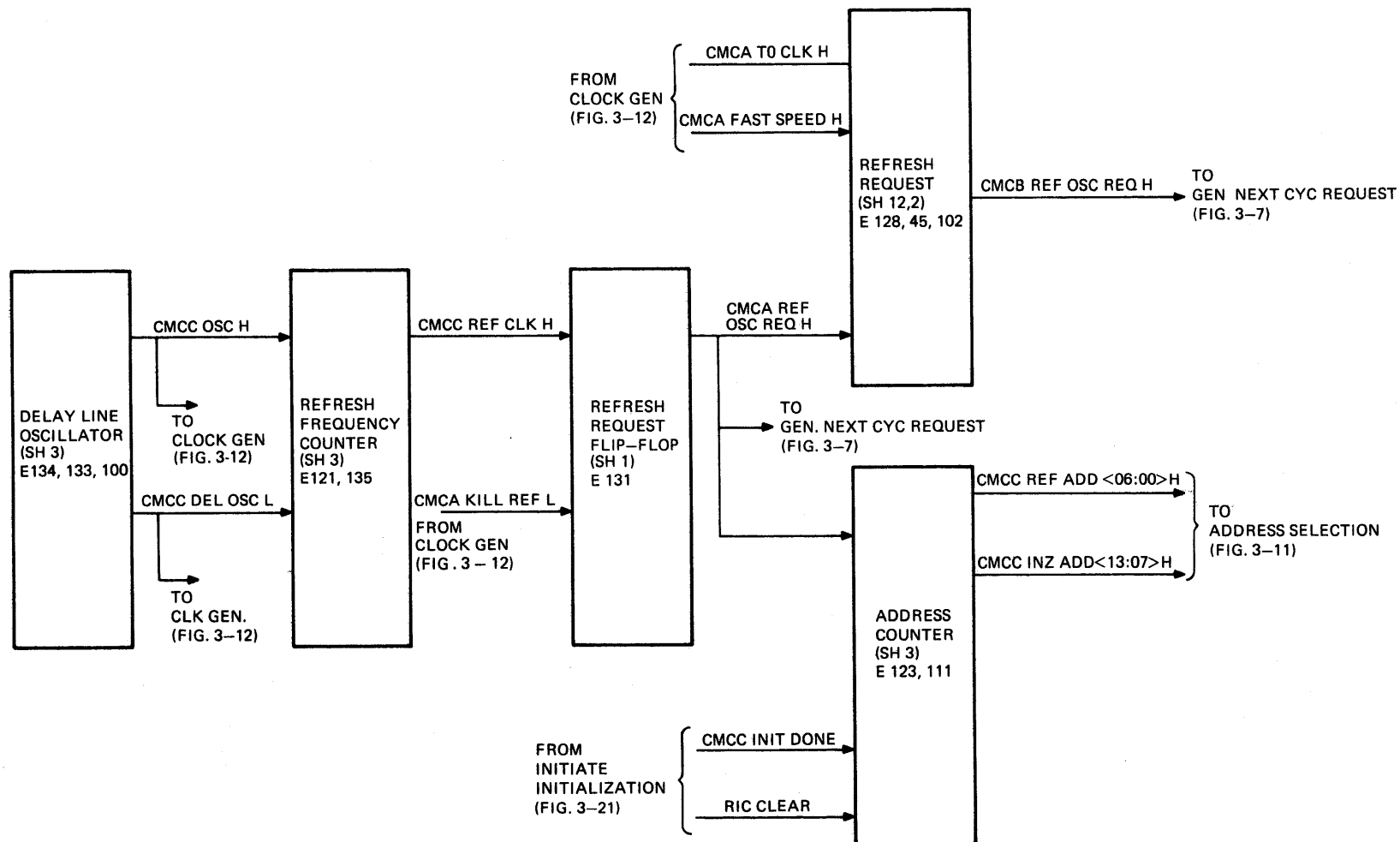
Figure 3-13 Refresh and Initialize Addressing
