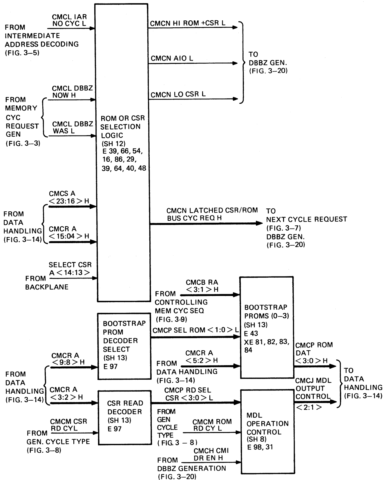
Figure 3-6 CSR and ROM Decoding
