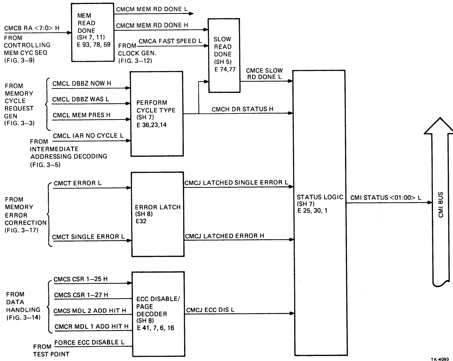
Figure 3-19 Status Generation
