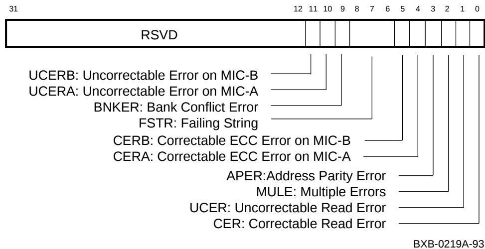
Figure 3: Memory Error Register A
