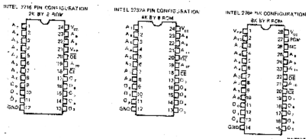
Figure 3-4 PROM Chips
