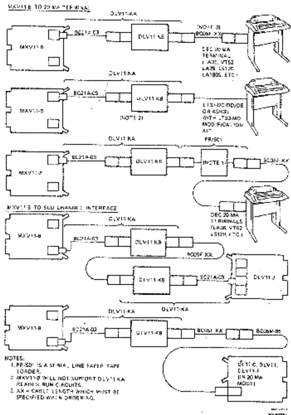
Figure 2-10 MXV11-B 20 mA Cable Configurations
