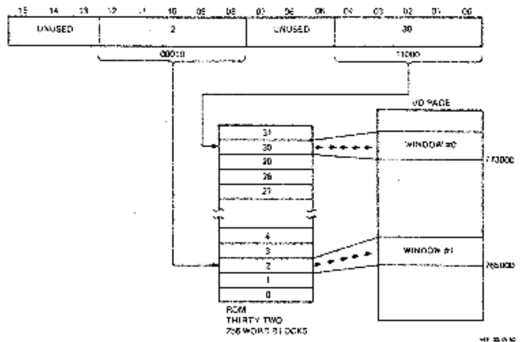
Figure 2-2 Page Mode Addressing
