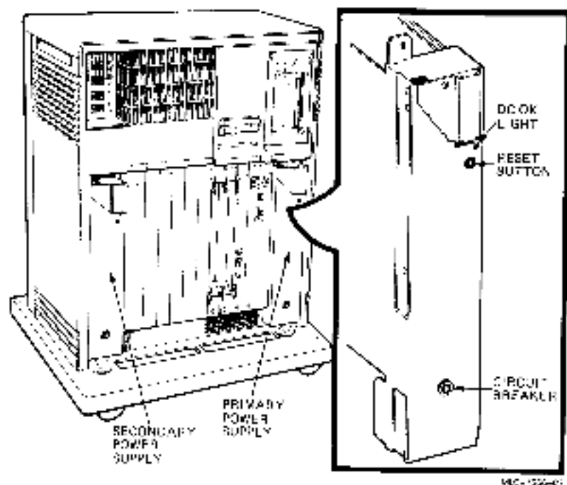
Figure 1-12: Power Supply
