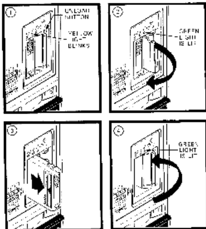
Figure 3 7: Removing a Tape Cartridge
