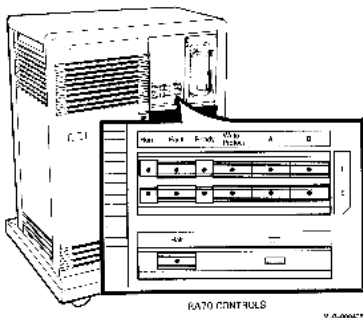
Figure 3-1: RA70 Controls and Indicators
