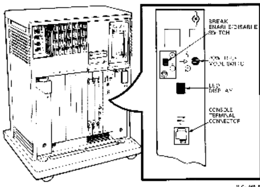
Figure 1-11: CPU Cover Panel
