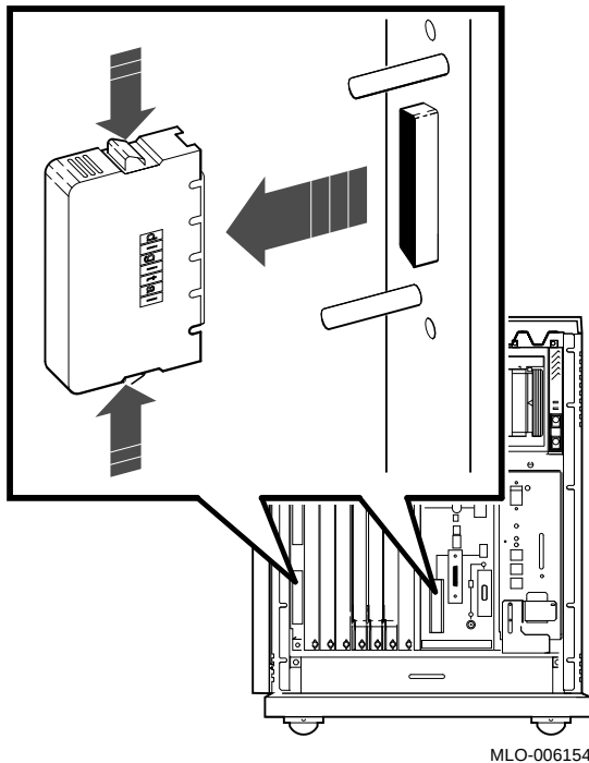
Figure 31: Removing the DSSI Terminator
