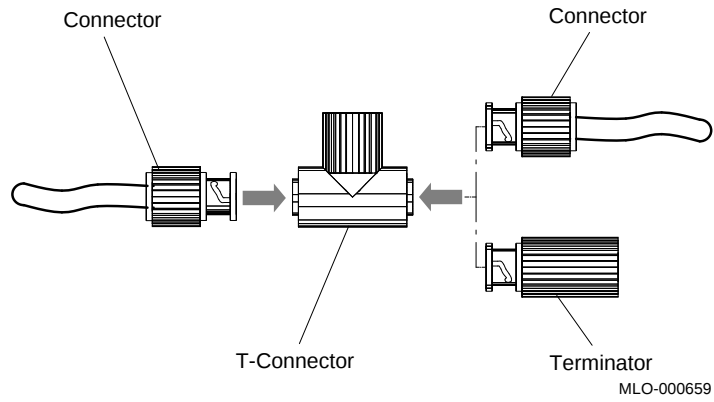
Figure 20: ThinWire Cable, T-Connector, and Terminator
