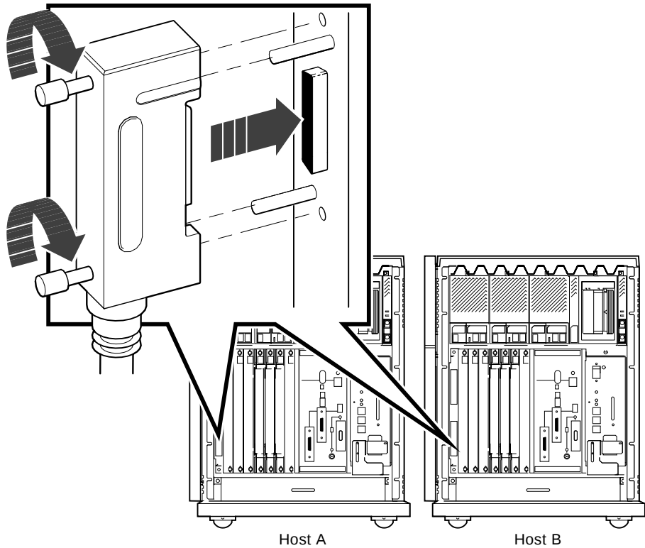
Figure 41: Connecting the DSSI Cable
