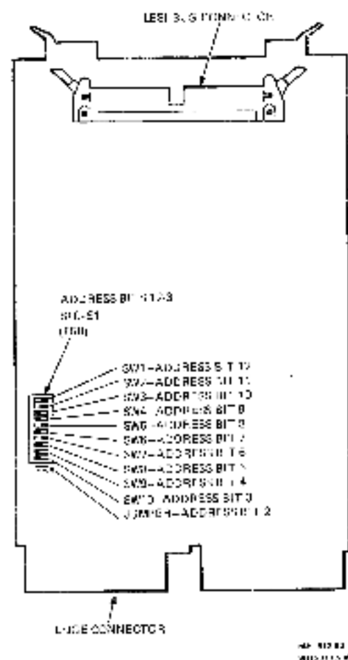
Figure 2-8: M7740 KLES-Q Adapter Module
