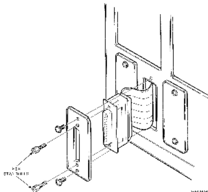
Figure 2-12: KLES1-Q I/O Connector
