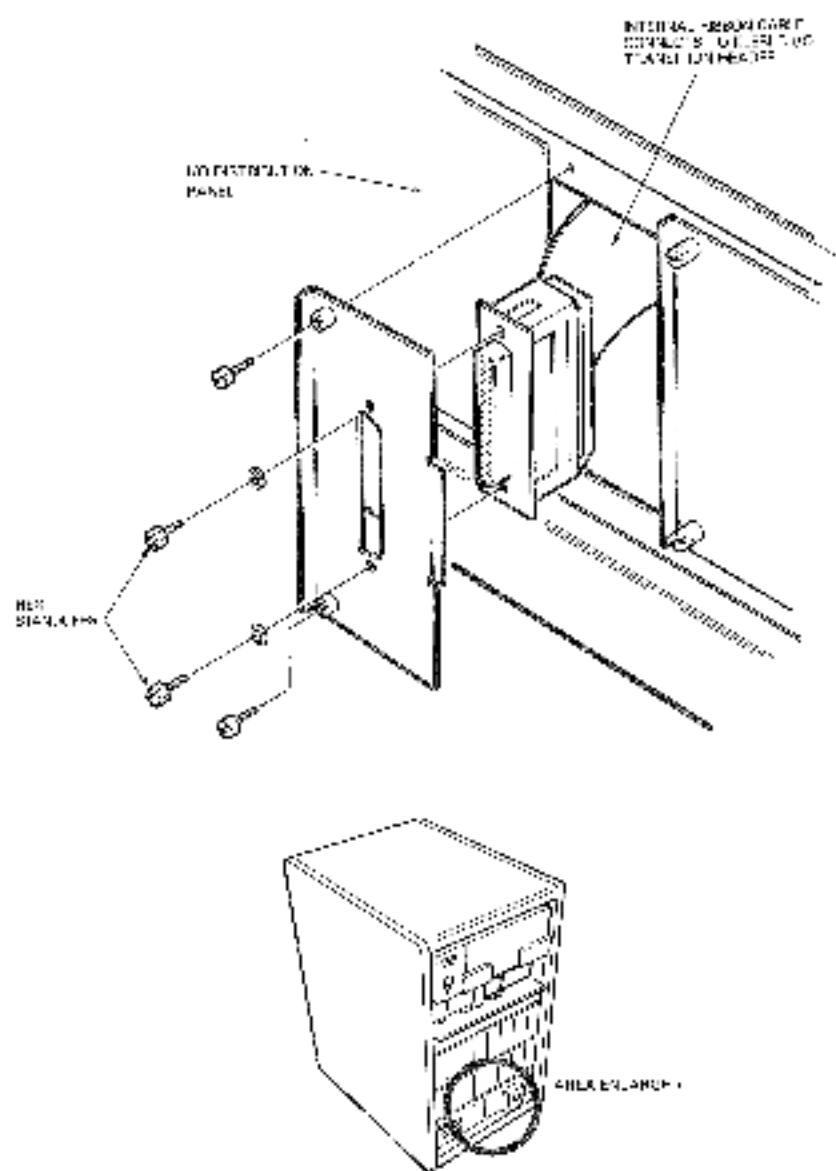
Figure 2-5: KLES1-B I/O Connector
