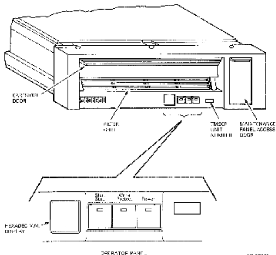
Figure 2-15: RV20 Front Panel
