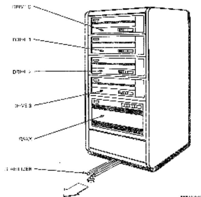
Figure 4-1: H9643 Cabinet
