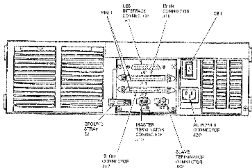
Figure 2-13: RV20 Rear Panel
