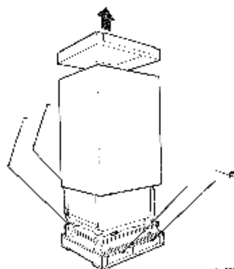
Figure 1-3: Removing the RV20 from its Skid - Step 1
