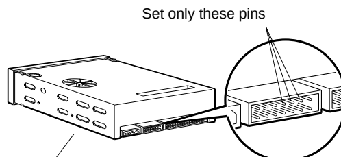
TZK10 QIC tape drive
