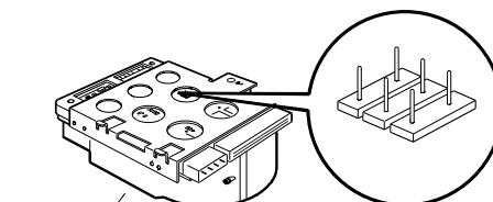
RZ24 hard disk drive
